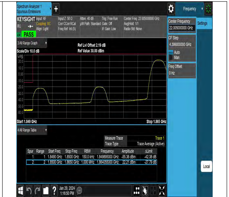
Band2_15MHz_QPSK_18675_1RB#74
