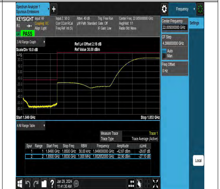
Band2_3MHz_QPSK_18615_1RB#14
