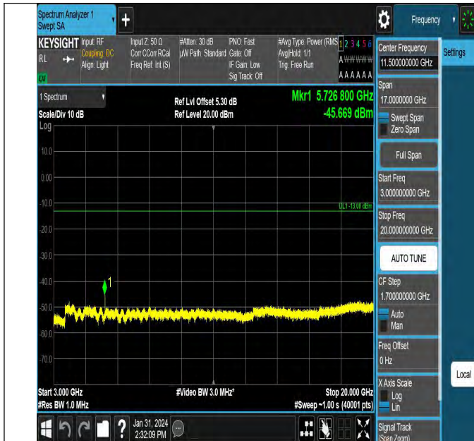
Band2_1.4MHz_QPSK_19193_1RB#0_3000~20000_3000~20000
