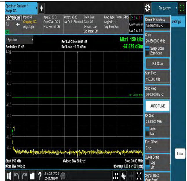
Band2_3MHz_QPSK_18900_1RB#0_0.15~30_0.15~30
