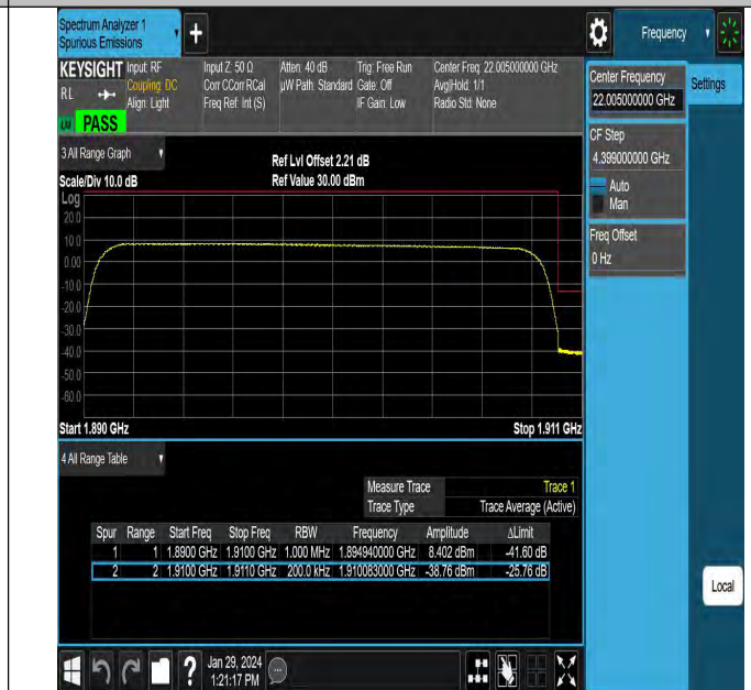
Band2_20MHz_QPSK_19100_100RB#0
