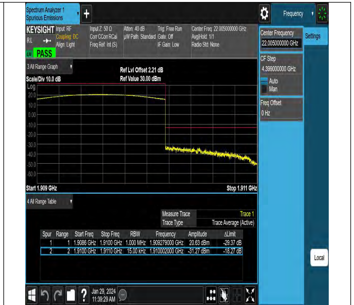
Band2_1.4MHz_QPSK_19193_6RB#0
