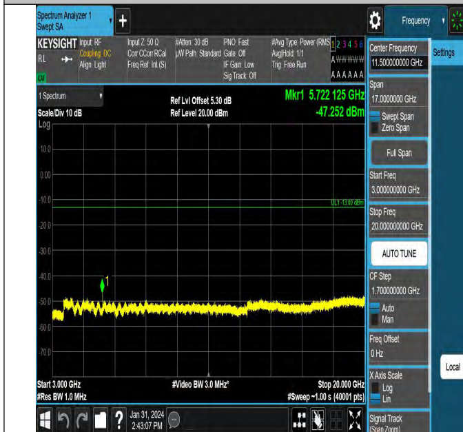
Band2_3MHz_QPSK_19185_1RB#0_3000~20000_3000~20000
