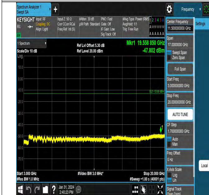
Band2_3MHz_QPSK_18615_1RB#0_3000~20000_3000~20000
