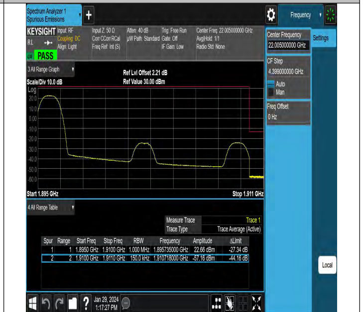
Band2_15MHz_QPSK_19125_1RB#0
