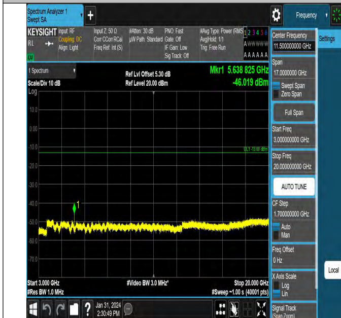
Band2_1.4MHz_QPSK_18900_1RB#0_3000~20000_3000~200
