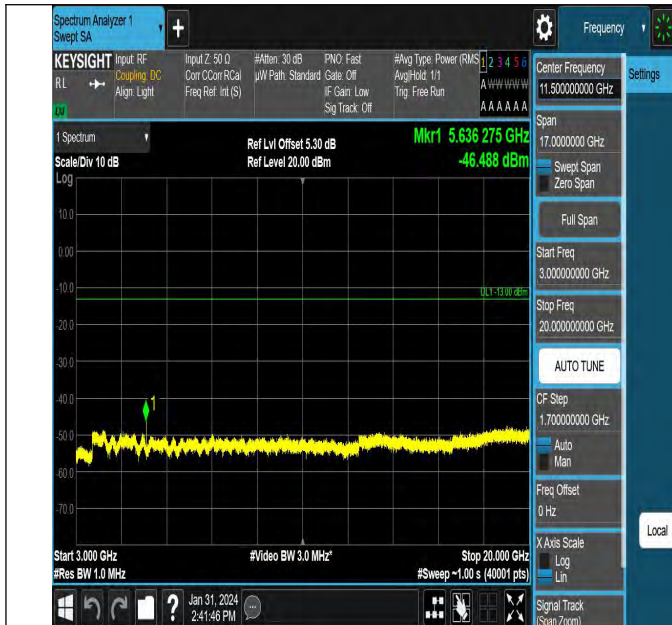
Band2_3MHz_QPSK_18900_1RB#0_3000~20000_3000~20000
