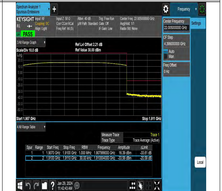
Band2_3MHz_QPSK_19185_15RB#0
