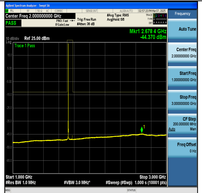
NTNV-n66-PC3-15-45-M-DFT-BPSK-Edge_1RB_Left- 1000-3000-PASS
