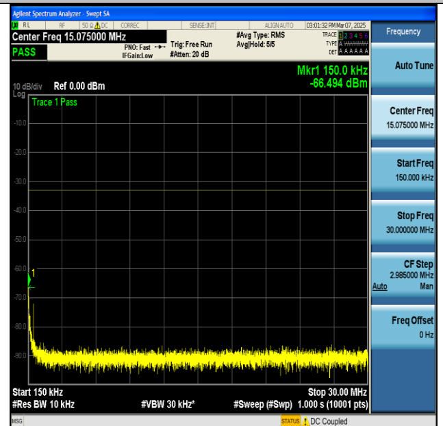
NTNV-n66-PC3-15-45-H-CP-QPSK-Edge_1RB_Left-0.15- 30-PASS
