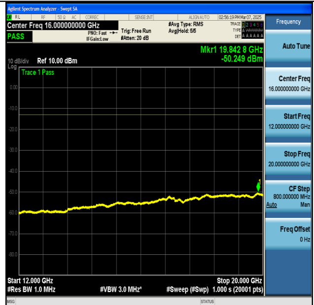
NTNV-n66-PC3-15-45-L-CP-QPSK-Edge_1RB_Left-12000-20000-PASS
