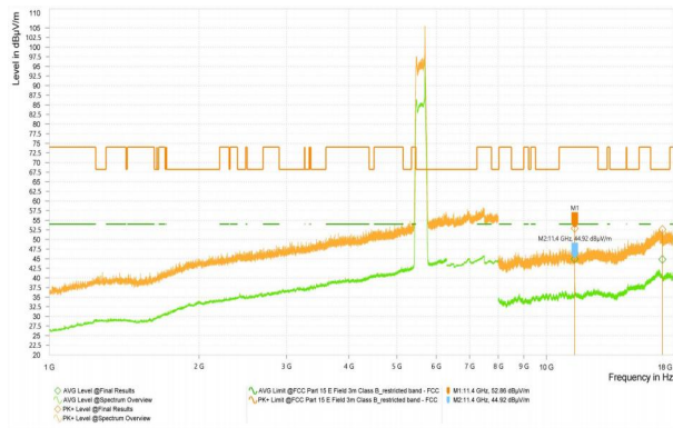
Wi-Fi 5G-11N20_5180_High
