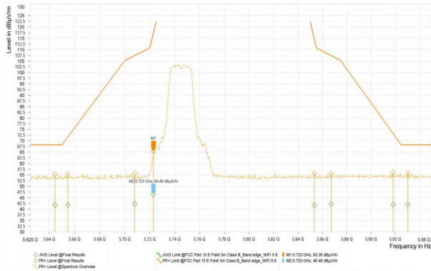
Wi-Fi 5G_11N40_5755
