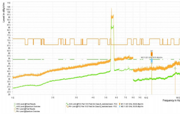
Wi-Fi 5G-11N40_5710_High
