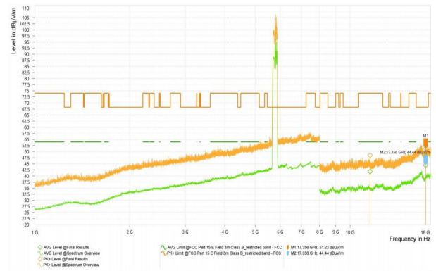
Wi-Fi 5G-11N40_5755_High
