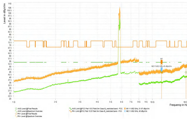
Wi-Fi 5G-11N20_5825_High
