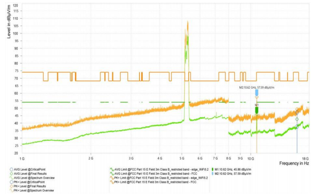
Wi-Fi 5G-11N40_5670_High
