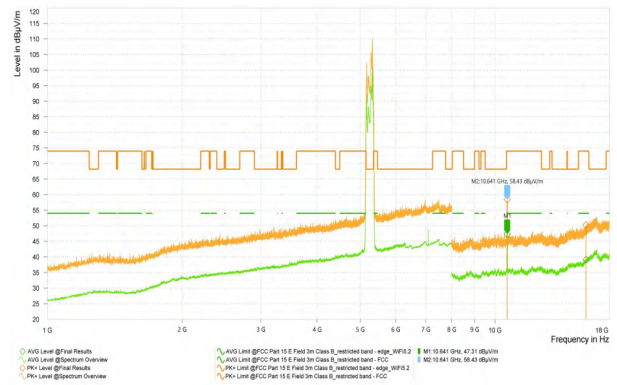
Wi-Fi 5G-11N20_5580_High
