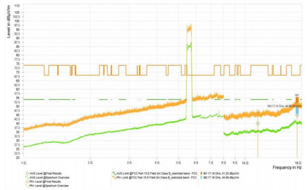
Wi-Fi 5G-11N20_5220_High
