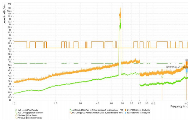
Wi-Fi 5G-11N40_5795_High
