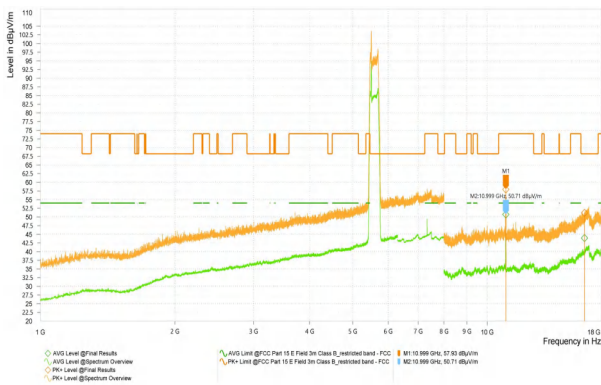
Wi-Fi 5G-11N20_5700_High
