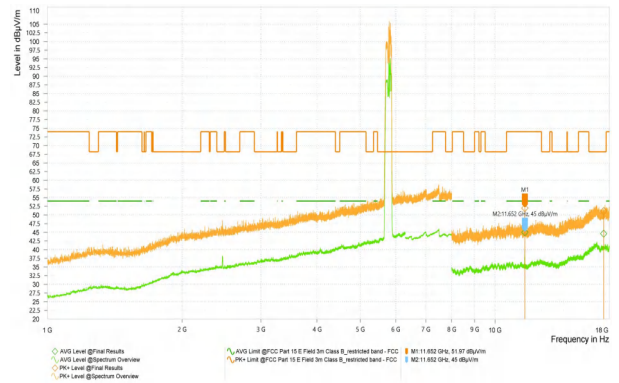
Wi-Fi 5G-11N20_5785_High
