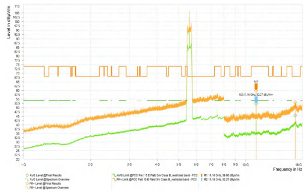
Wi-Fi 5G-11N20_5720_High
