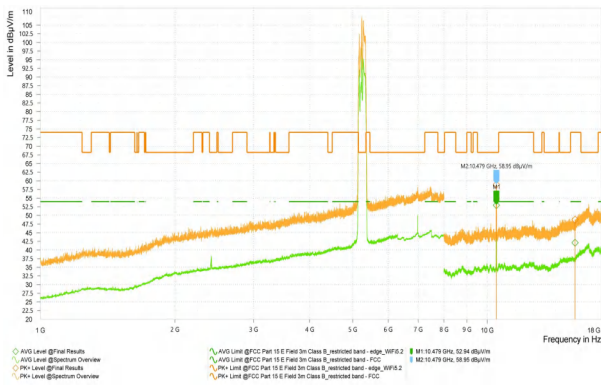
Wi-Fi 5G-11N20_5300_High
