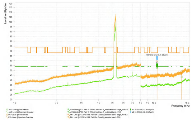
Wi-Fi 5G-11N20_5320_High
