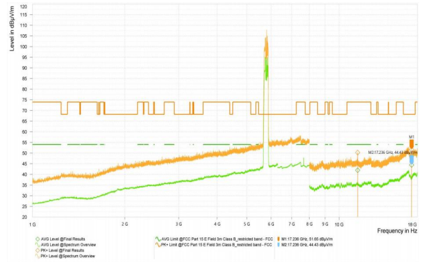
Wi-Fi 5G-11A_5825_High
