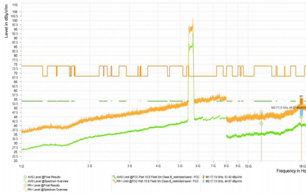
Wi-Fi 5G-11A_5785_High
