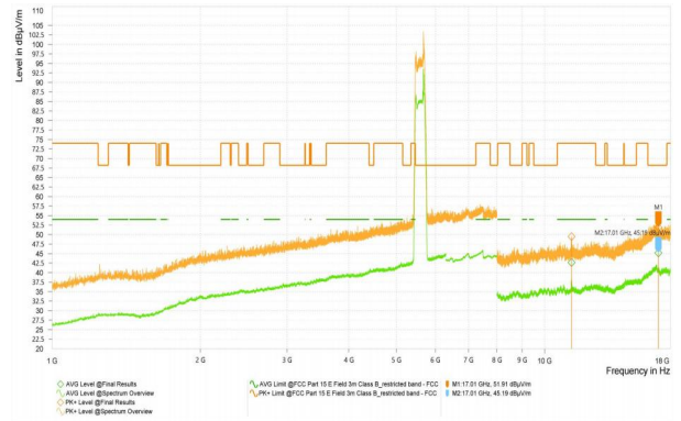
Wi-Fi 5G-11A_5745_High
