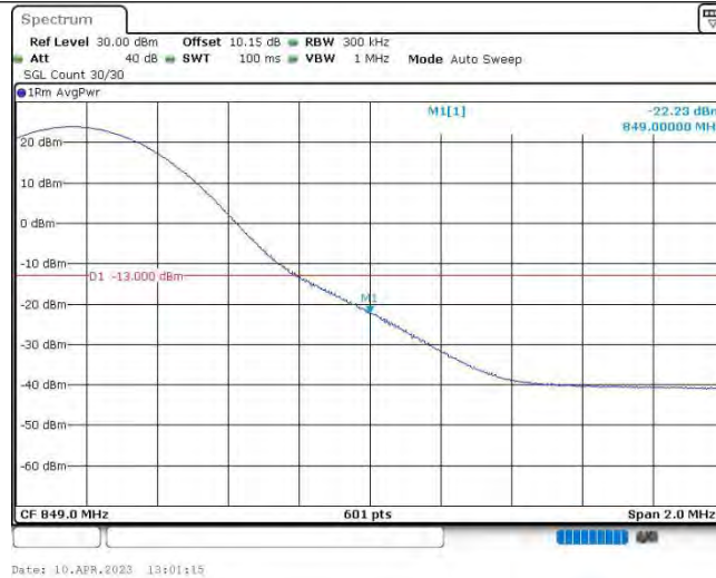
Band26@22-15MHz-QPSK-26965-1RB#74
