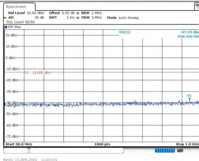
Band4-3MHz-QPSK-20385-1RB#0-Range1:30~1000MHz
