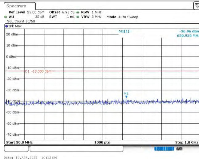
Band2-3MHz-QPSK-18615-1RB#0-Range1:30~1000MHz
