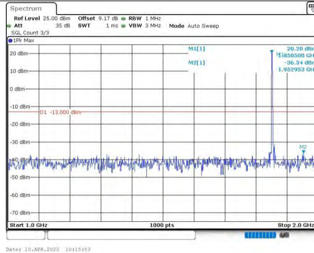
Band2-5MHz-16QAM-18625-1RB#0-Range2:1000~2000MHz
