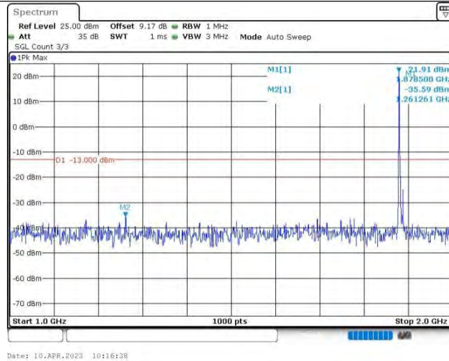
Band2-5MHz-16QAM-18900-1RB#0-Range2:1000~2000MHz
