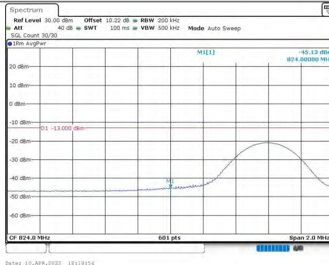
Band26@22-10MHz-16QAM-26840-1RB#49
