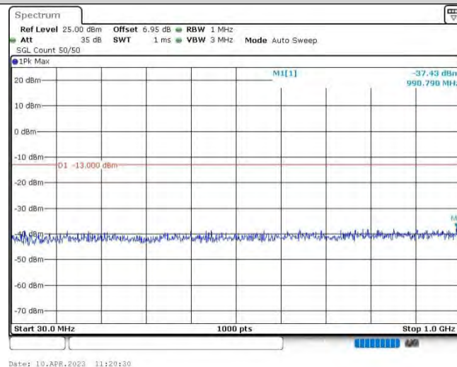
Band4-3MHz-QPSK-20175-1RB#0-Range1:30~1000MHz
