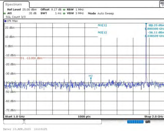
Band2-1.4MHz-QPSK-18900-1RB#0-Range2:1000~2000MHz
