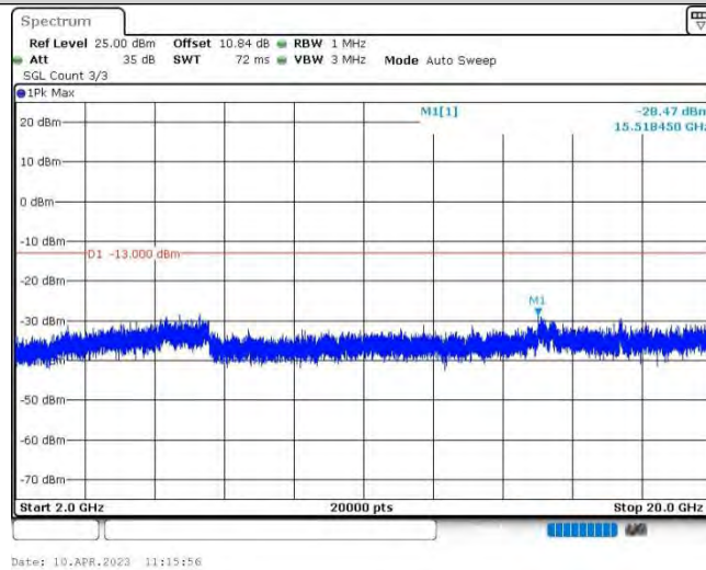
Band4-1.4MHz-QPSK-20393-1RB#0-Range3:2000~20000MHz
