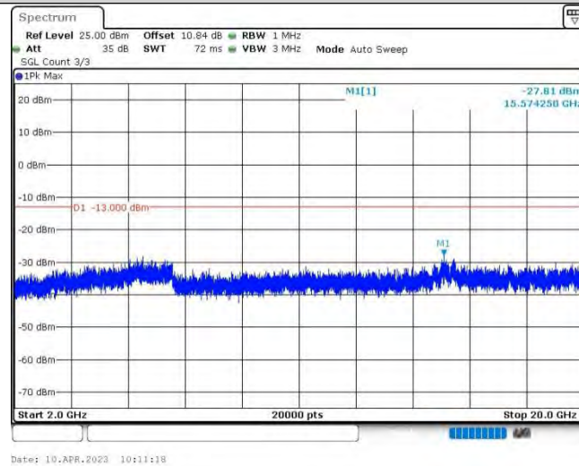
Band2-1.4MHz-QPSK-19193-1RB#0-Range3:2000~20000MHz
