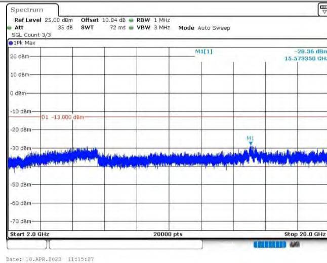
Band4-1.4MHz-16QAM-20175-1RB#0-Range3:2000~20000MHz
