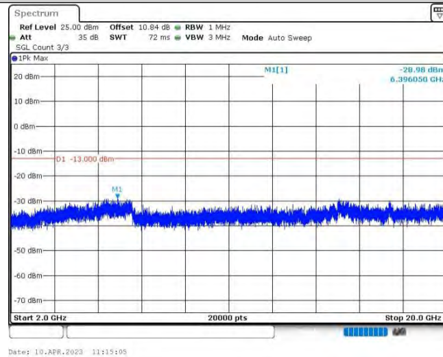
Band4-1.4MHz-QPSK-20175-1RB#0-Range3:2000~20000MHz
