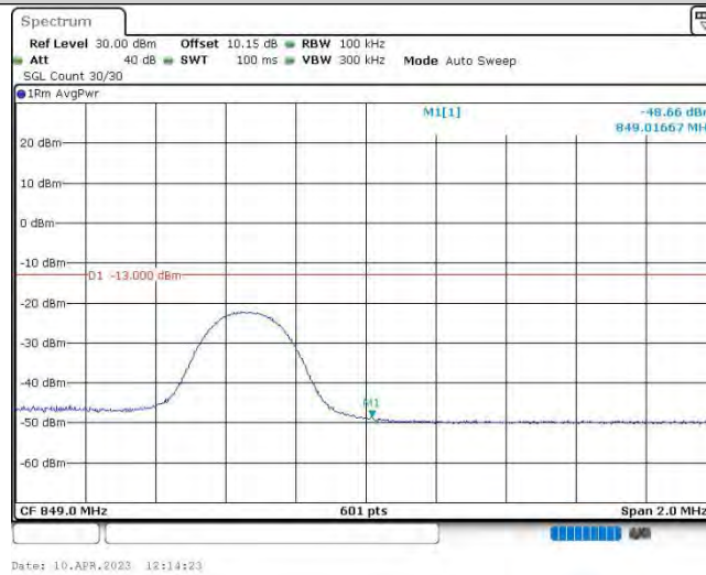
Band26@22-5MHz-16QAM-27015-1RB#0
