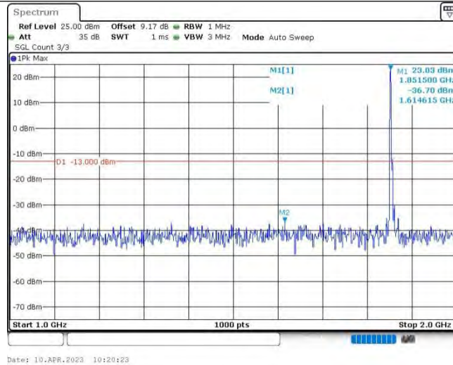
Band2-10MHz-16QAM-18650-1RB#0-Range2:1000~2000MHz
