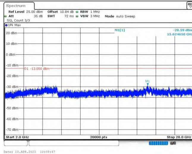
Band2-1.4MHz-QPSK-18607-1RB#0-Range3:2000~20000MHz
