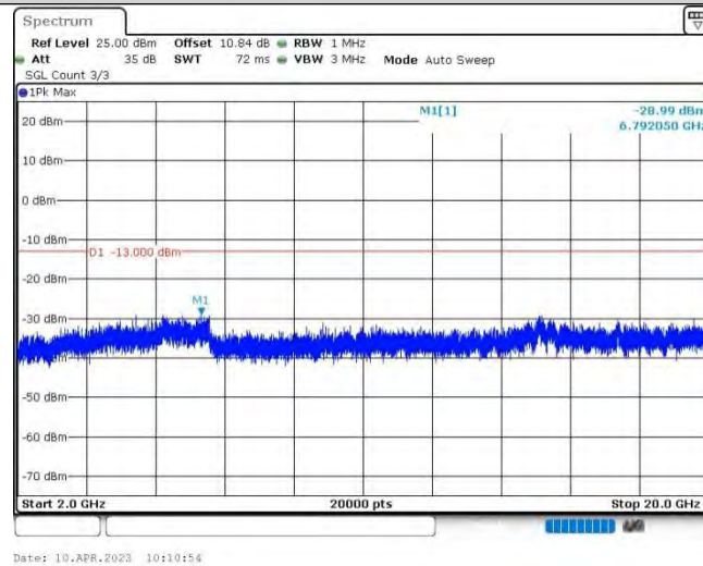
Band2-1.4MHz-16QAM-18900-1RB#0-Range3:2000~20000MHz
