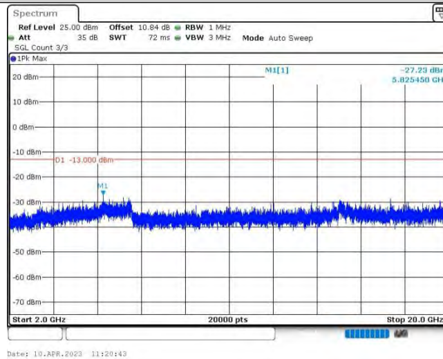
Band4-3MHz-QPSK-20175-1RB#0-Range3:2000~20000MHz
