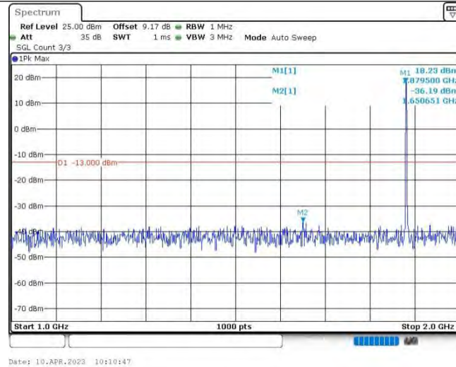
Band2-1.4MHz-16QAM-18900-1RB#0-Range2:1000~2000MHz
