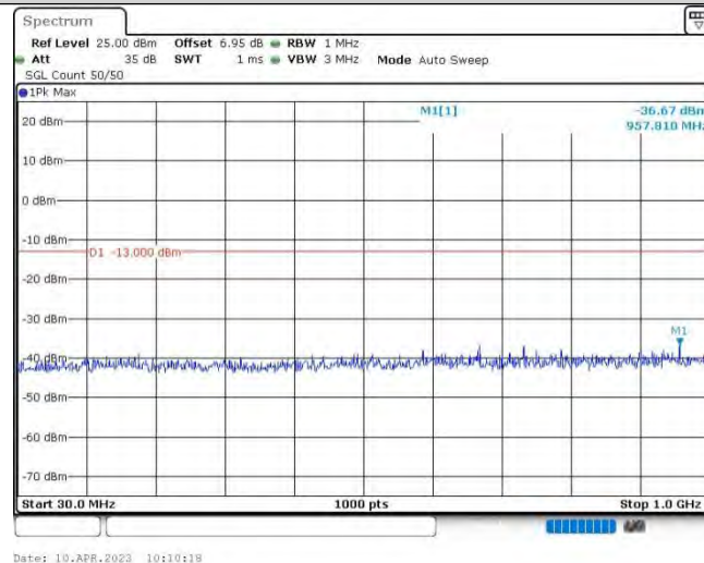
Band2-1.4MHz-QPSK-18900-1RB#0-Range1:30~1000MHz
