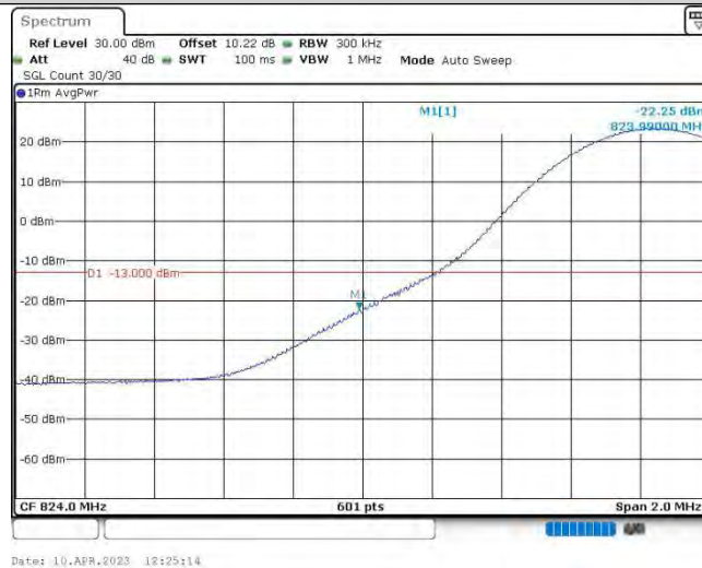
Band26@22-15MHz-16QAM-26865-1RB#0
