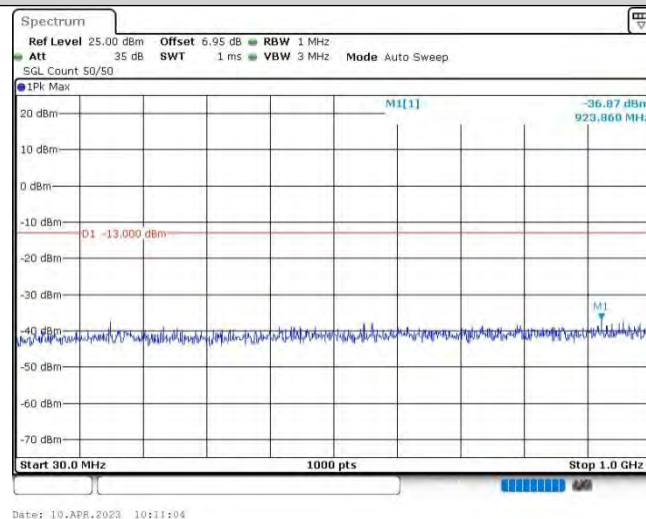
Band2-1.4MHz-QPSK-19193-1RB#0-Range1:30~1000MHz
