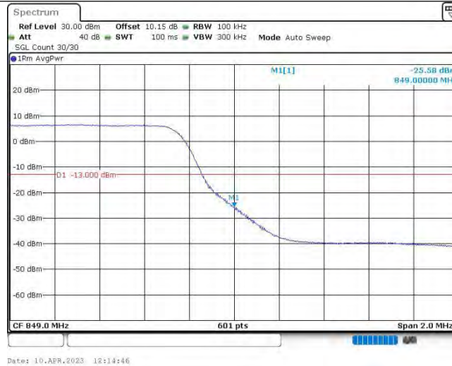
Band26@22-5MHz-QPSK-27015-25RB#0
