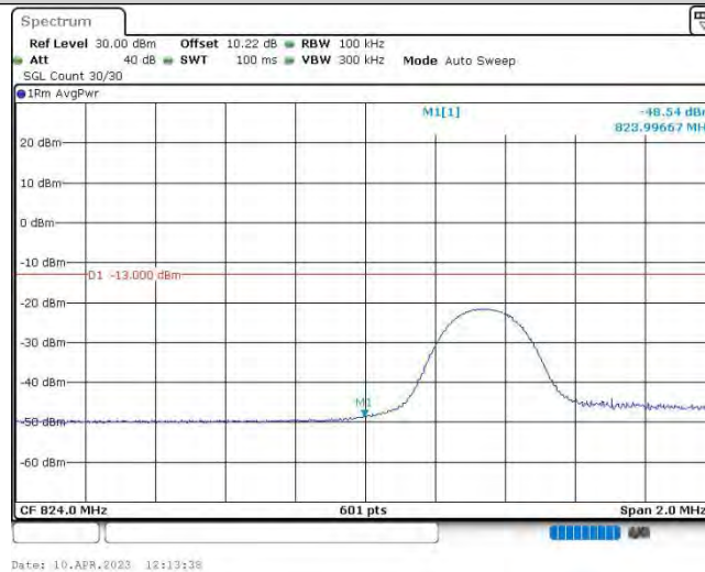
Band26@22-5MHz-16QAM-26815-1RB#24
