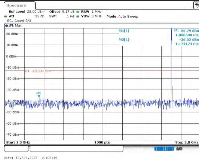
Band2-1.4MHz-QPSK-18607-1RB#0-Range2:1000~2000MHz
