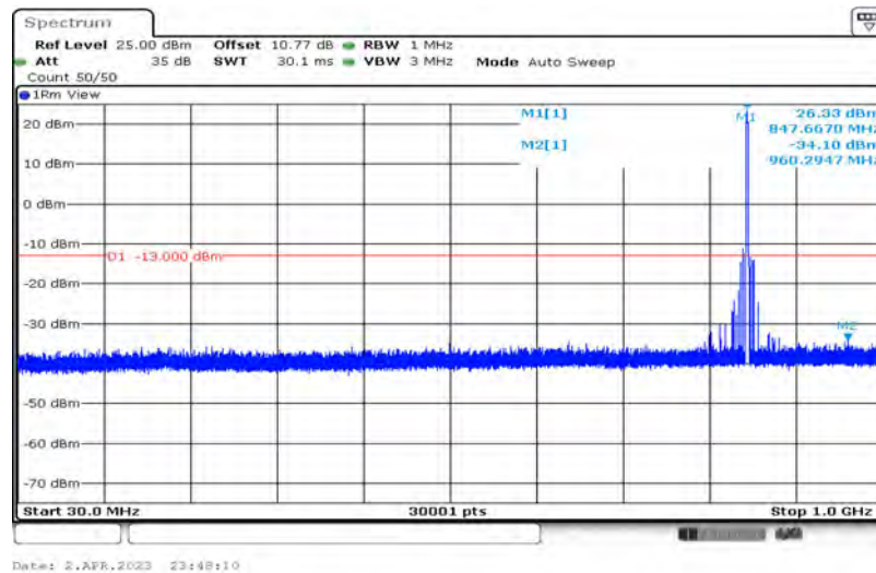
Band5-3MHz-QPSK-20635-1-0-High-30-1000--34.1-PASS
