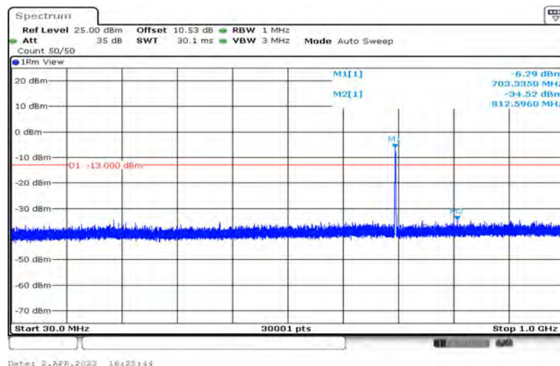
Band12-10MHz-16QAM-23095-1-0-Low-30-1000--34.52-PASS
