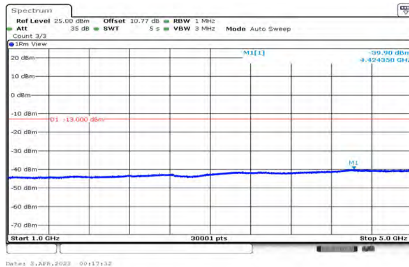
Band5-10MHz-16QAM-20525-1-0-Low-1000-5000--39.9-PASS
