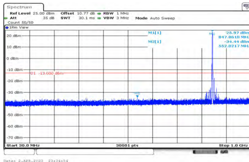
Band5-1.4MHz-16QAM-20643-1-0-High-30-1000--34.44-PASS
