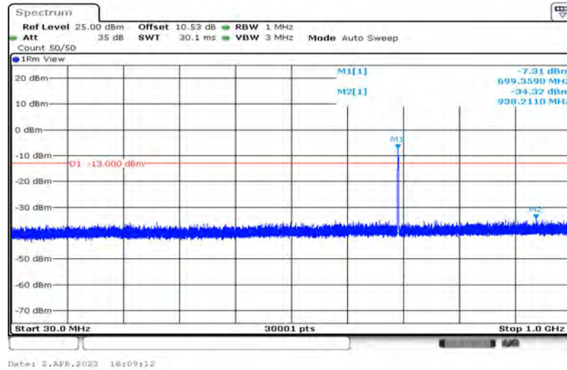
Band12-5MHz-16QAM-23035-1-0-Low-1000-5000--40.15-PASS
