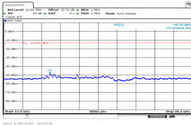
Band13-5MHz-QPSK-23205-1-0-Low-12000-26500--48.34-PASS
