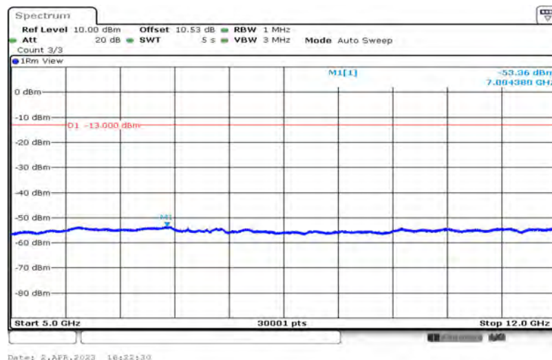
Band12-10MHz-QPSK-23060-1-0-Low-5000-12000--53.36-PASS
