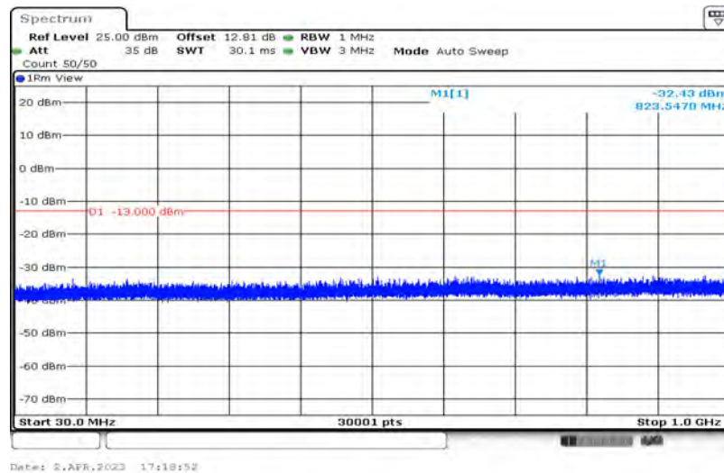
Band25-3MHz-16QAM-26675-1-0-High-30-1000--32.43-PASS
