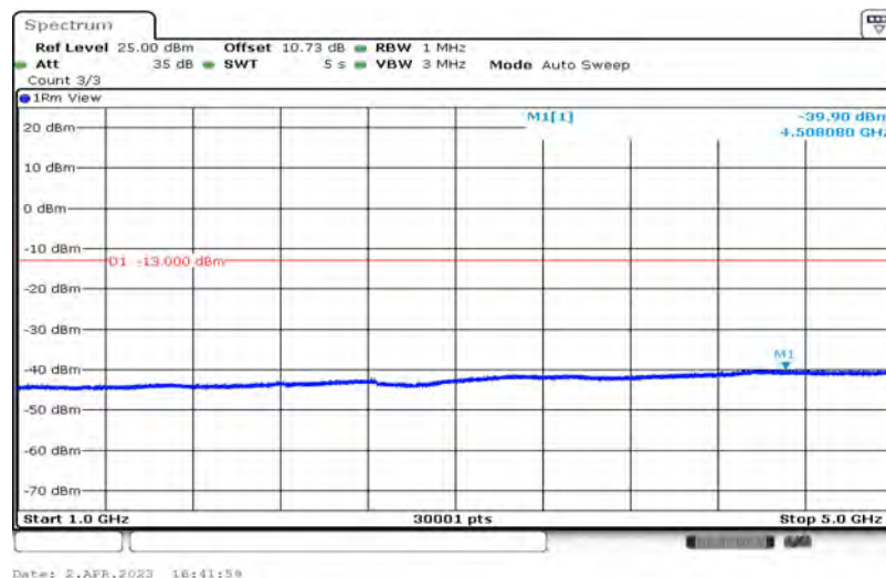
Band13-5MHz-16QAM-23230-1-0-Low-1000-5000--39.9-PASS
