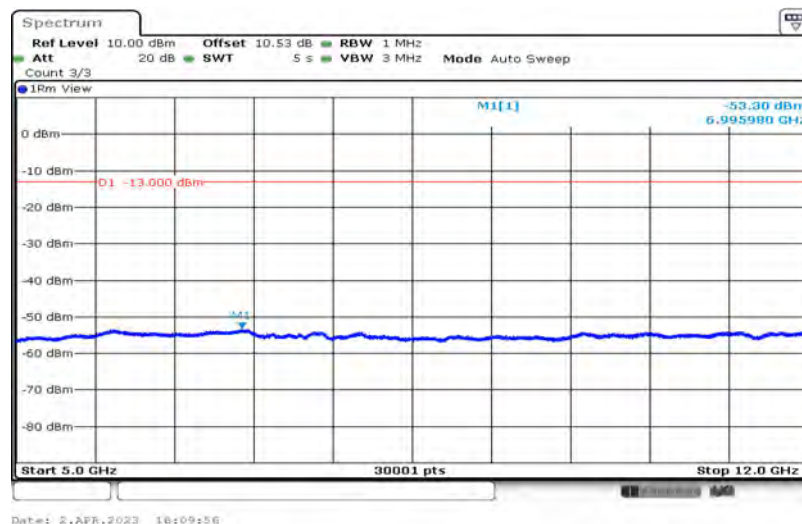
Band12-5MHz-16QAM-23035-1-0-Low-5000-12000--53.3-PASS
