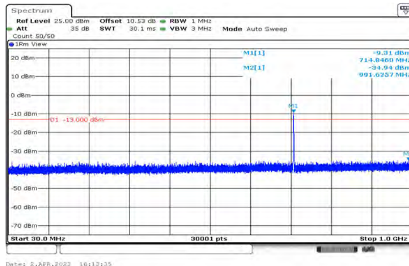
Band12-5MHz-QPSK-23155-1-0-High-30-1000--34.94-PASS
