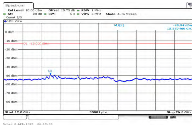
Band5-10MHz-QPSK-20450-1-0-Low-12000-26500--48.54-PASS
