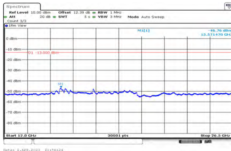
Band4-20MHz-QPSK-20300-1-0-High-12000-26500--46.76-PASS
