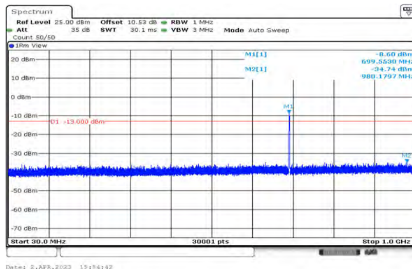
Band12-3MHz-QPSK-23025-1-0-Low-30-1000--34.74-PASS
