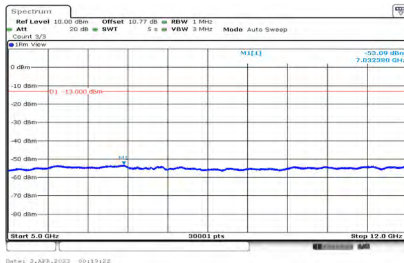
Band5-10MHz-QPSK-20600-1-0-High-5000-12000--53.09-PASS
