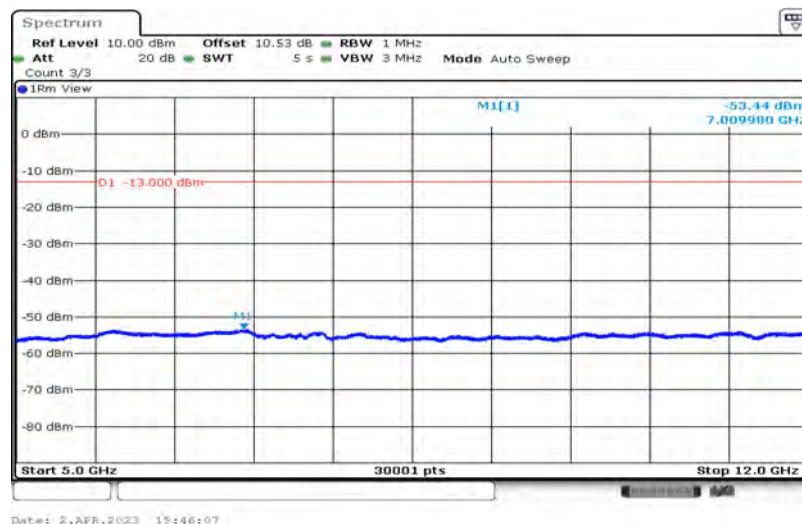
Band12-1.4MHz-16QAM-23095-1-0-Low-5000-12000--53.44-PASS
