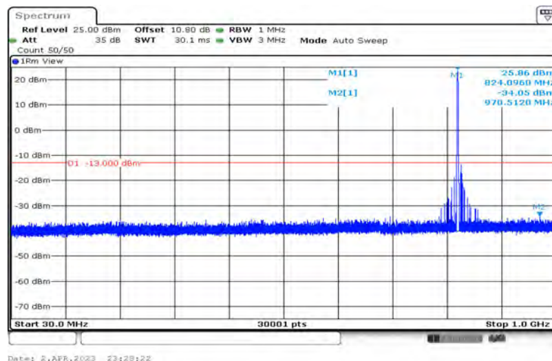
Band5-1.4MHz-QPSK-20407-1-0-Low-30-1000--34.05-PASS
