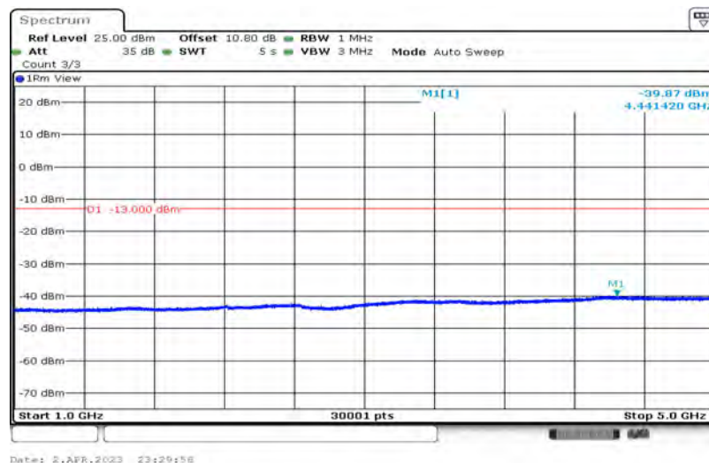
Band5-1.4MHz-16QAM-20407-1-0-Low-1000-5000--39.87-PASS
