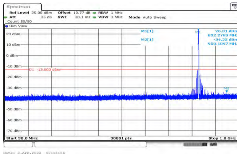
Band5-10MHz-QPSK-20525-1-0-Low-30-1000--34.25-PASS
