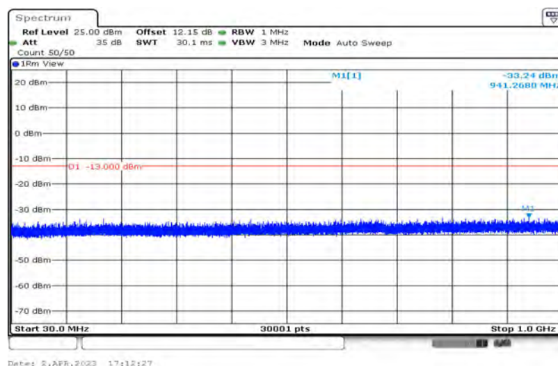
Band25-3MHz-QPSK-26055-1-0-Low-30-1000--33.24-PASS
