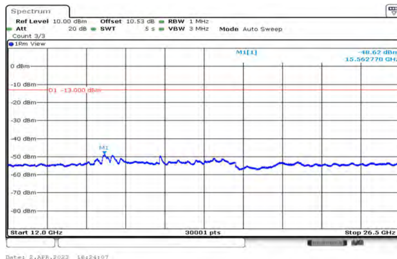
Band12-10MHz-16QAM-23060-1-0-Low-12000-26500--48.62-PASS
