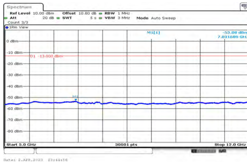
Band5-3MHz-16QAM-20415-1-0-Low-5000-12000--53.08-PASS
