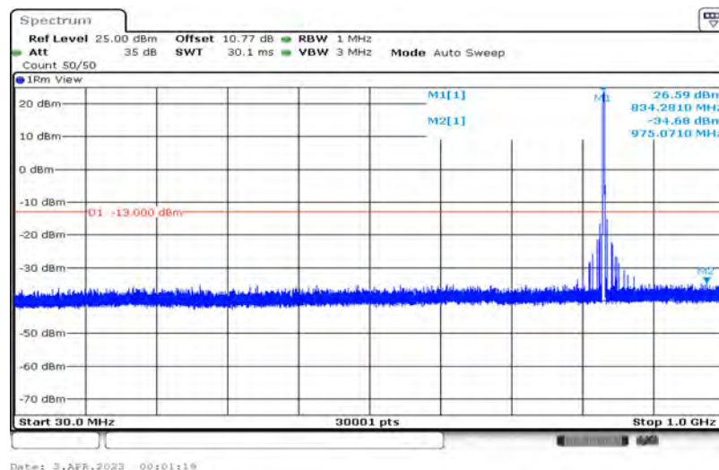
Band5-5MHz-16QAM-20525-1-0-Low-30-1000--34.68-PASS
