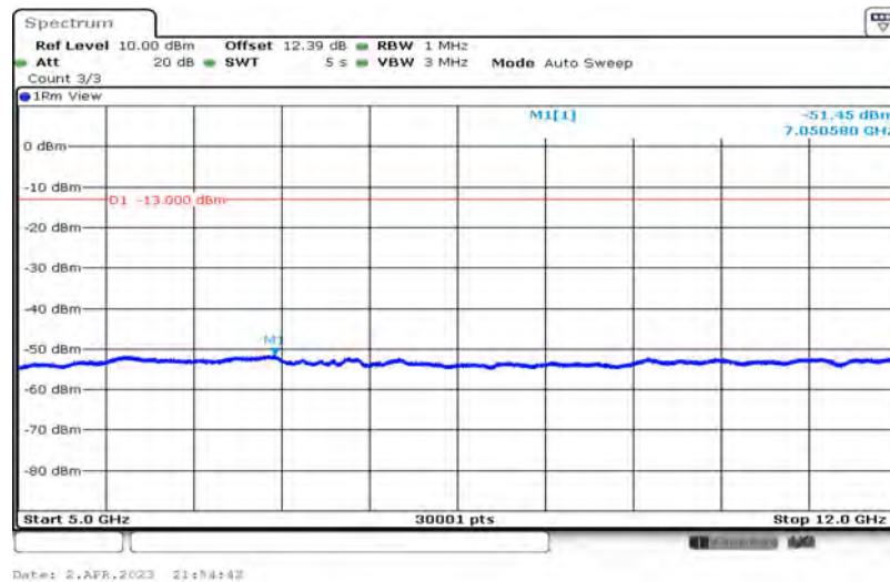
Band4-20MHz-16QAM-20175-1-0-Low-5000-12000--51.45-PASS
