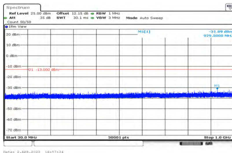
Band25-1.4MHz-16QAM-26047-1-0-Low-30-1000--31.89-PASS
