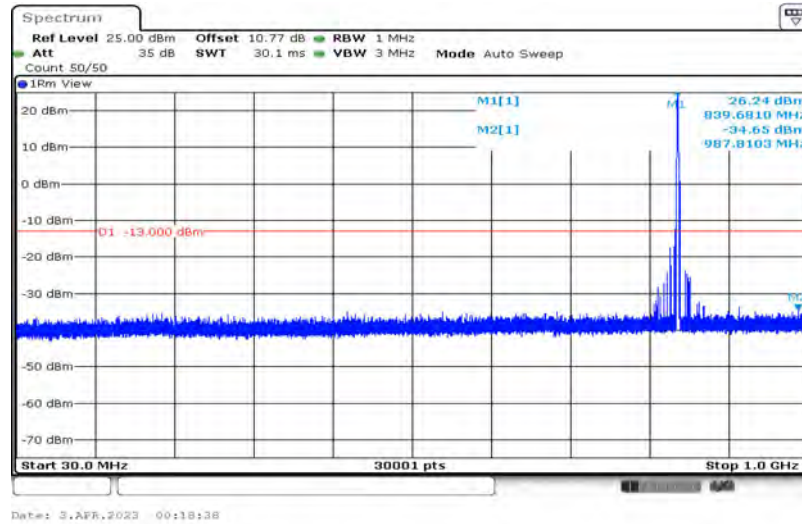
Band5-10MHz-QPSK-20600-1-0-High-1000-5000--39.9-PASS
