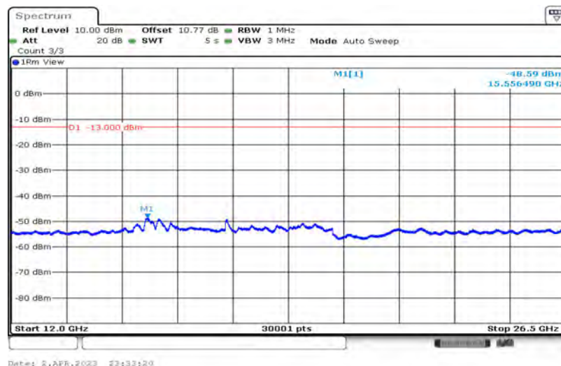
Band5-1.4MHz-16QAM-20525-1-0-Low-12000-26500--48.59-PASS
