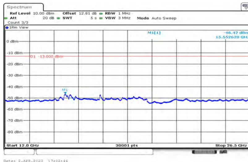
Band25-1.4MHz-QPSK-26683-1-0-High-12000-26500--46.42-PASS
