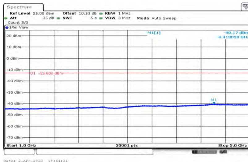
Band12-1.4MHz-QPSK-23095-1-0-Low-1000-5000--40.17-PASS
