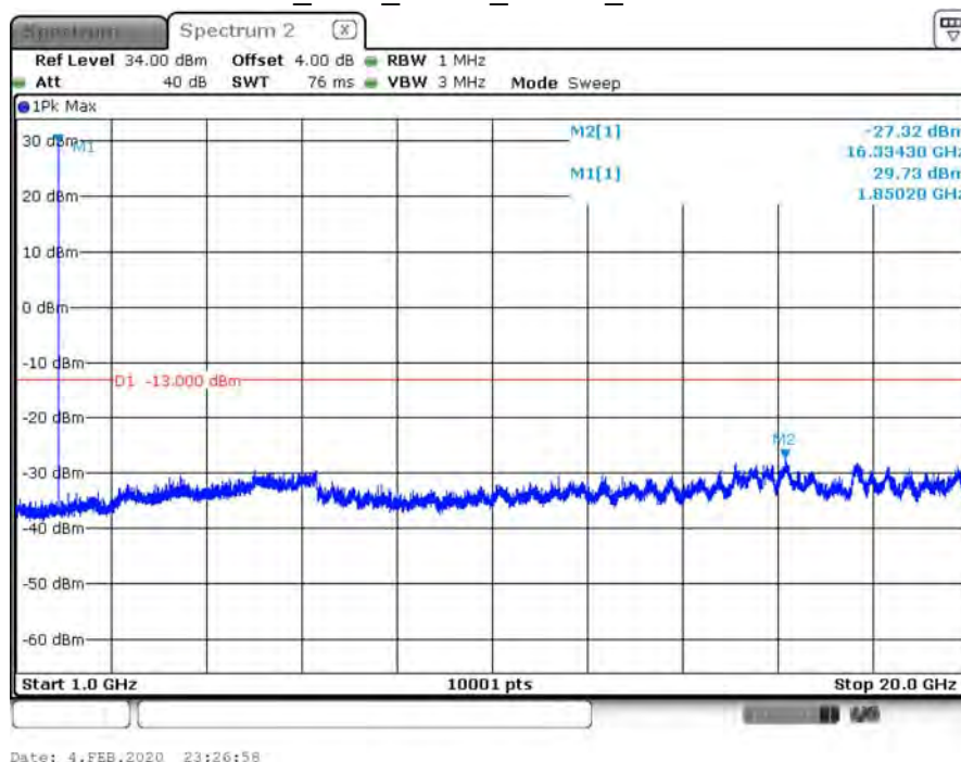
GSM_1900_GPRS_1850.2_above 1G
