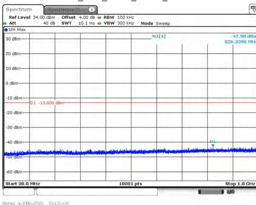
GSM_1900_GPRS_1850.2_under 1G
