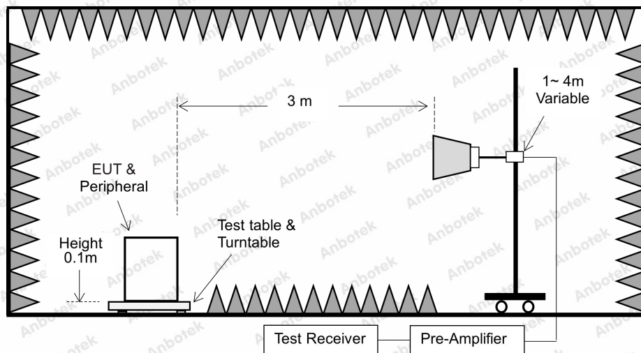
Figure 3. Above 1 GHz
