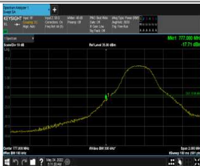
Band13-5MHz-QPSK-23205-1RB#24
