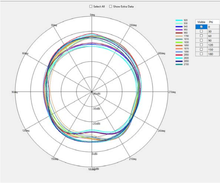
G900/G1800/B3/B7/B8/B41/W8 Phi=0deg
