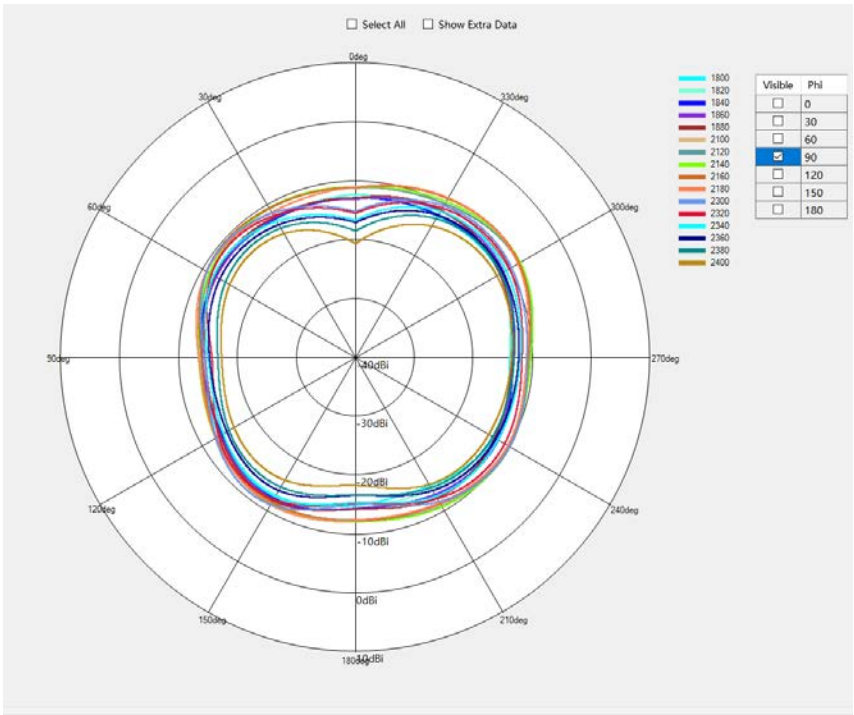
B1/B3/B40 Phi=90deg
