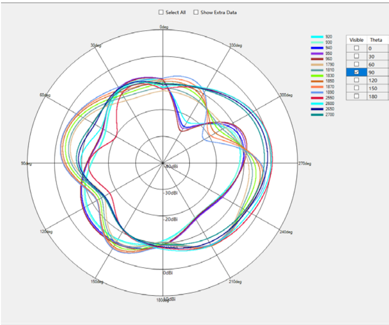
G900/G1800/B3/B7/B8/B41/W8 Theta=90deg
