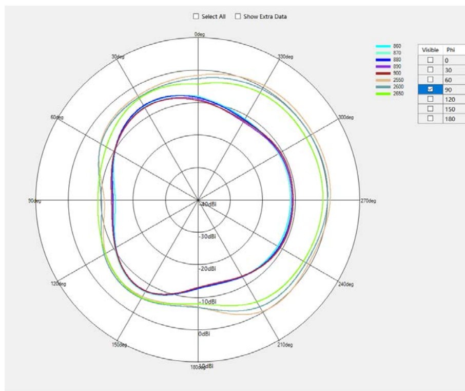
G850/B5/B38/W5 Phi=90deg
