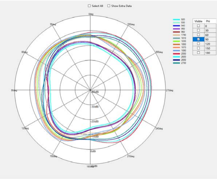
G900/G1800/B3/B7/B8/B41/W8 Phi=90deg
