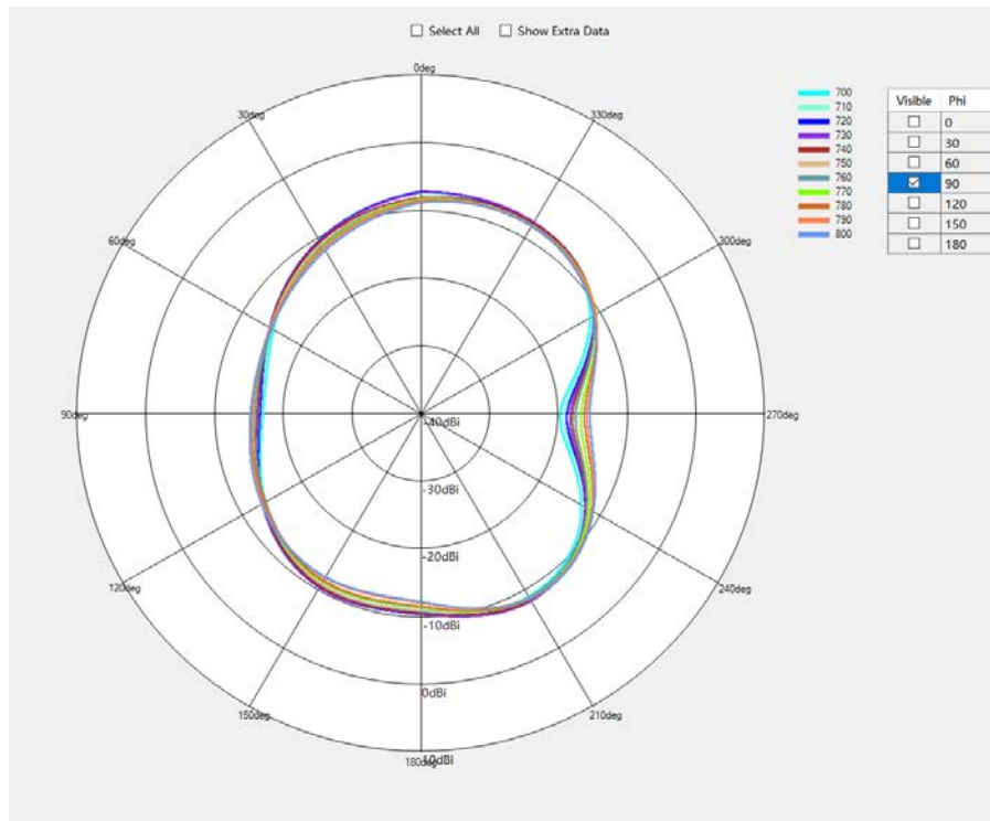
B28A/B28B Phi=90deg
