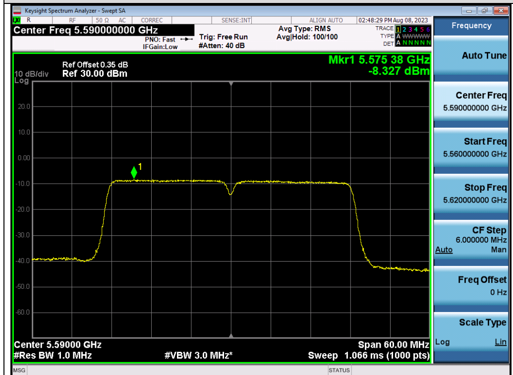
Test_Graph_802.11n40_ANT2_5590_MCS0_PSD
