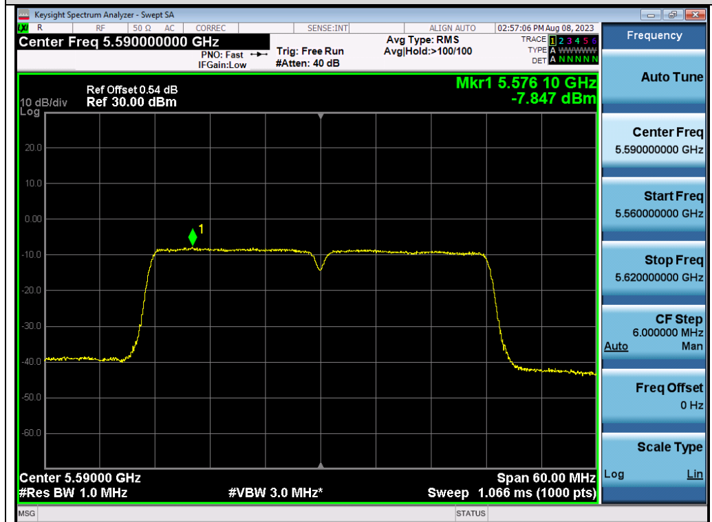
Test_Graph_802.11ac40_ANT2_5590_MCS9_PSD
