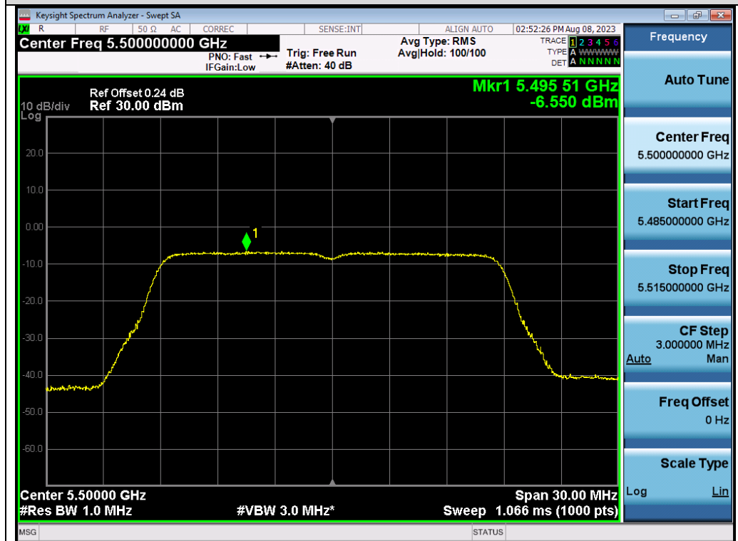
Test_Graph_802.11ac20_ANT2_5500_MCS0_PSD
