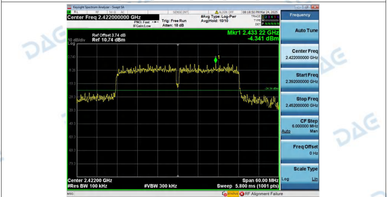
2_Bandedge_NVNT_ANT1_802_11n(HT40)_2422
