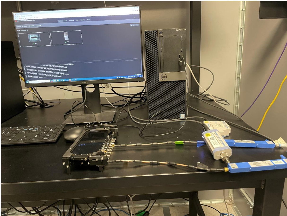
Figure C-3 UXM Conducted power test measurement setup dual port
