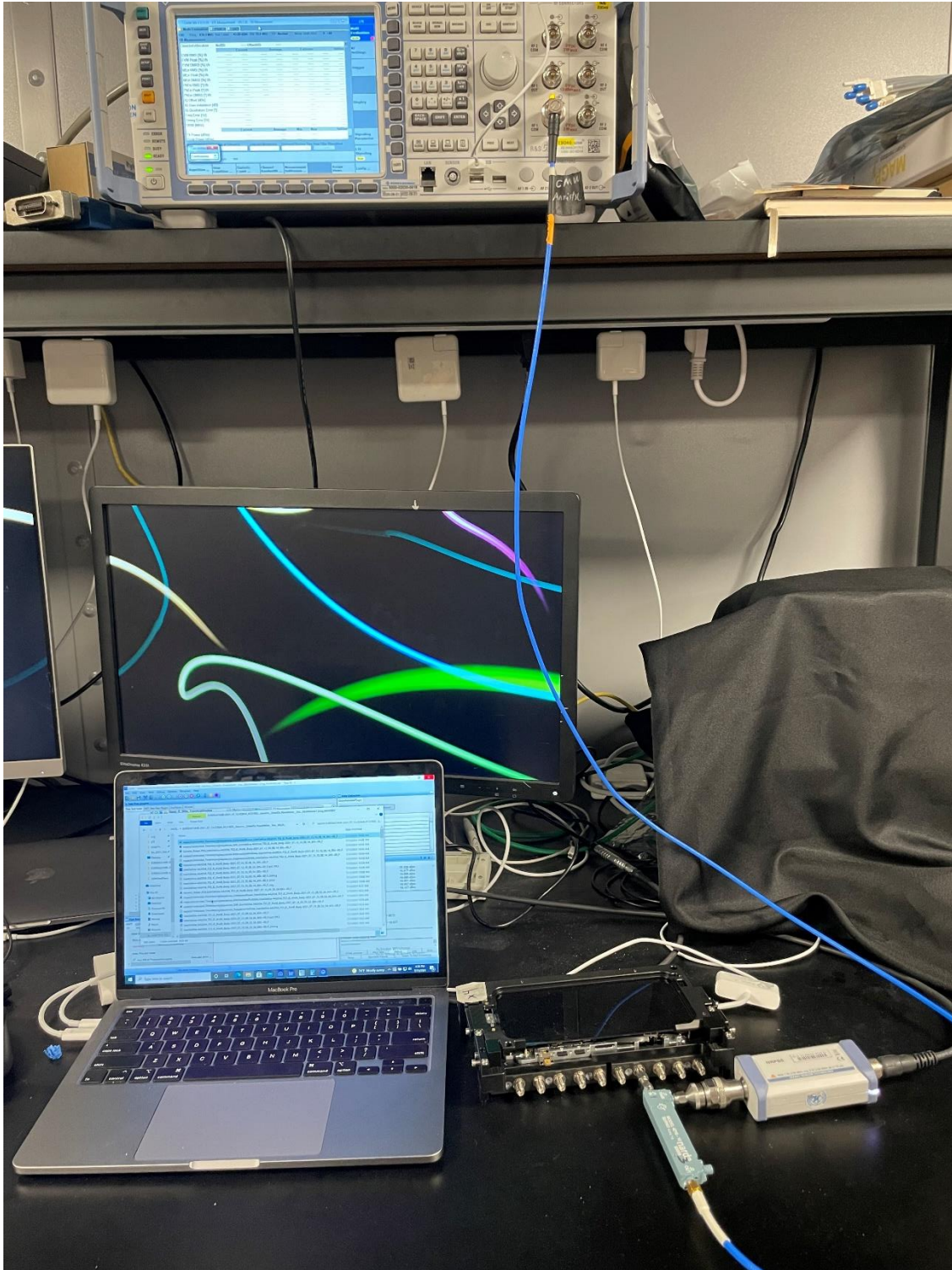
Figure C-1 CMW Conducted power test measurement setup single port
