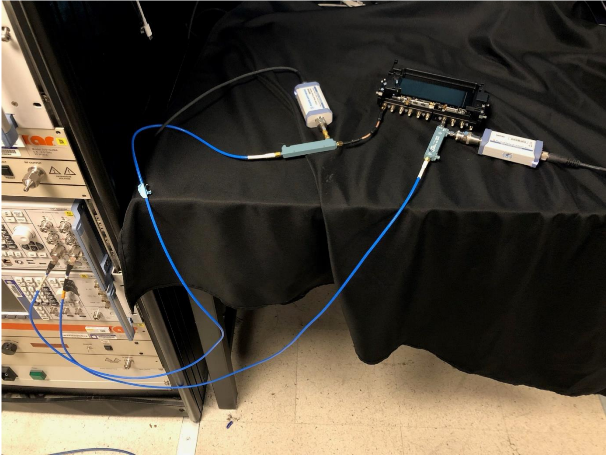
Figure C-2 CMW Conducted power test measurement setup dual port
