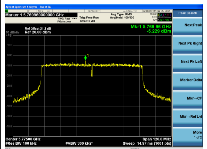
PSD-802.11ac-5775M-chain2
