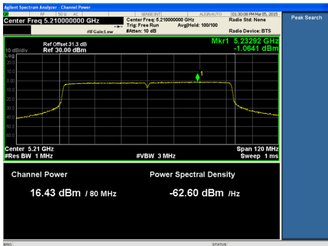
PSD-802.11ac-5210M-chain1
