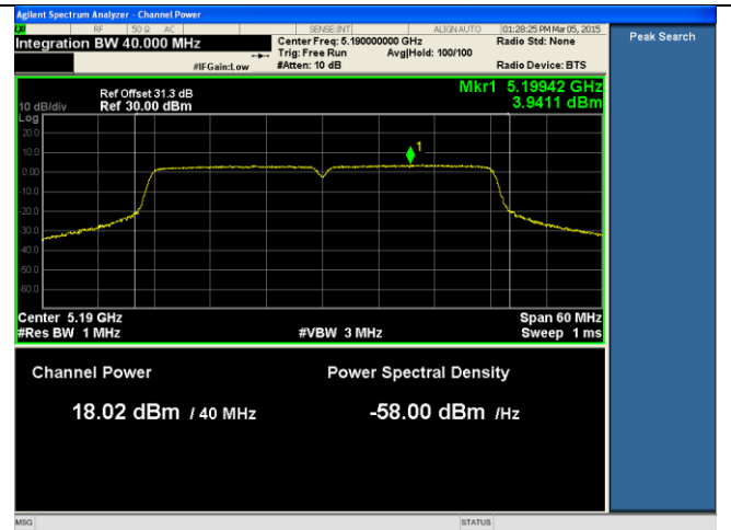
PSD-802.11n HT40-5190M-chain2
