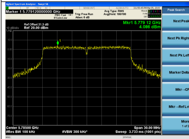
PSD-802.11n HT20-5785M-chain1
