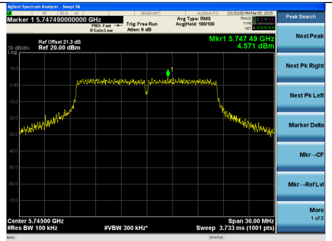
PSD-802.11a-5745M-chain2
