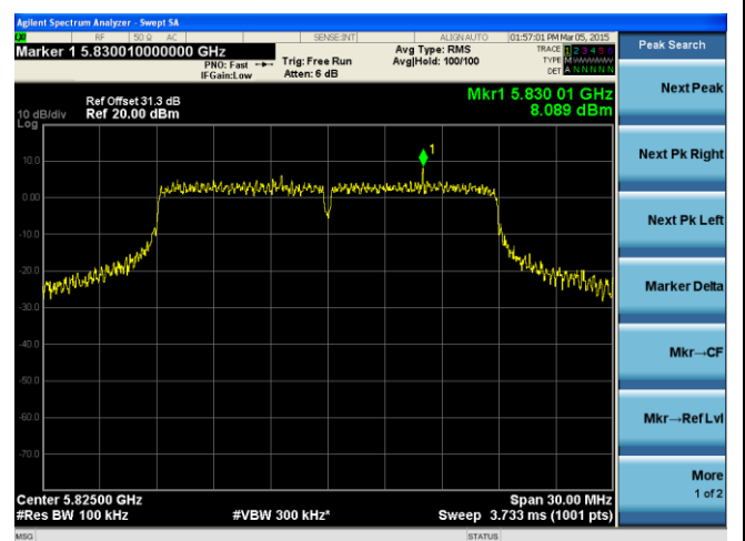
PSD-802.11n HT20-5825M-chain2
