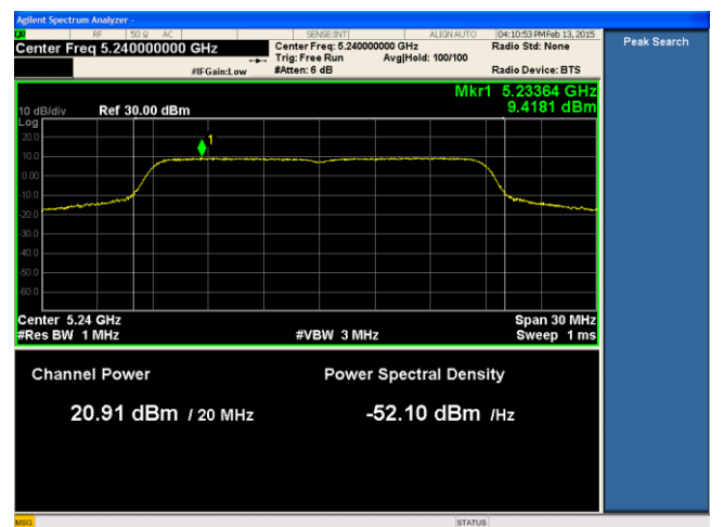
PSD-802.11n HT20-5240M-chain2
