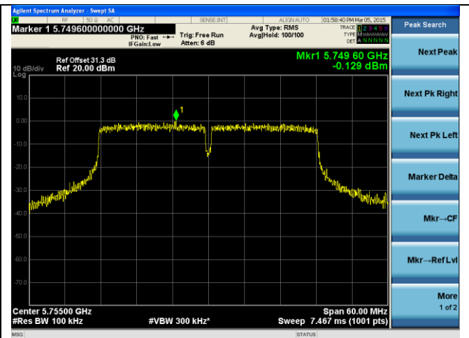
PSD-802.11n HT40-5755M-chain2
