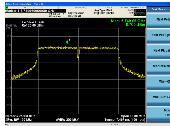
PSD-802.11n HT40-5755M-chain1
