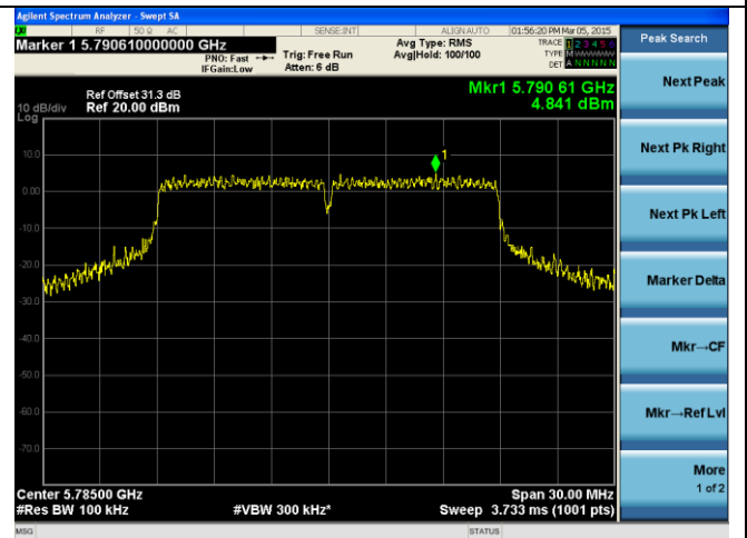
PSD-802.11n HT20-5785M-chain2
