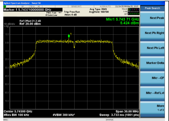
PSD-802.11n HT20-5745M-chain2
