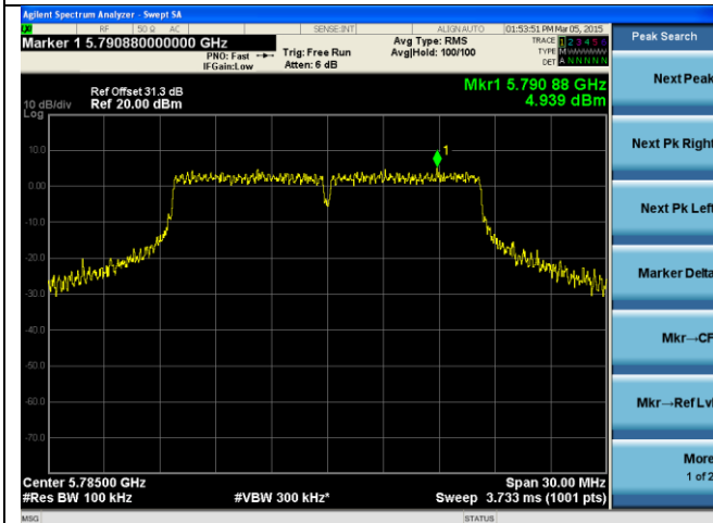
PSD-802.11a-5785M-chain1
