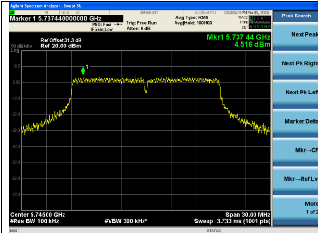
PSD-802.11n HT20-5745M-chain1
