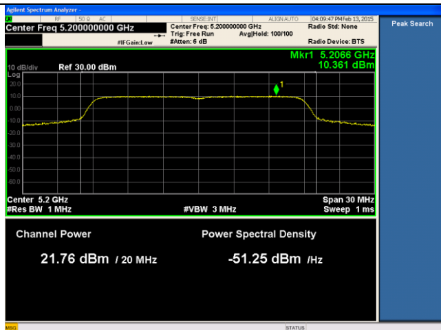
PSD-802.11n HT20-5200M-chain1
