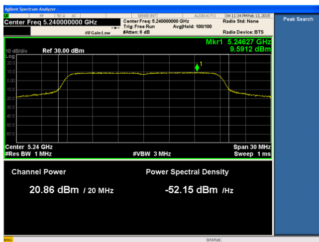
PSD-802.11n HT20-5240M-chain1
