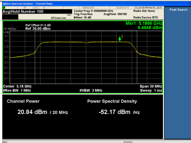
PSD-802.11n HT20-5180M-chain1
