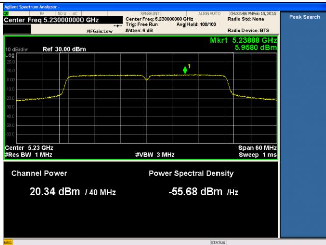
PSD-802.11n HT40-5230M-chain1
