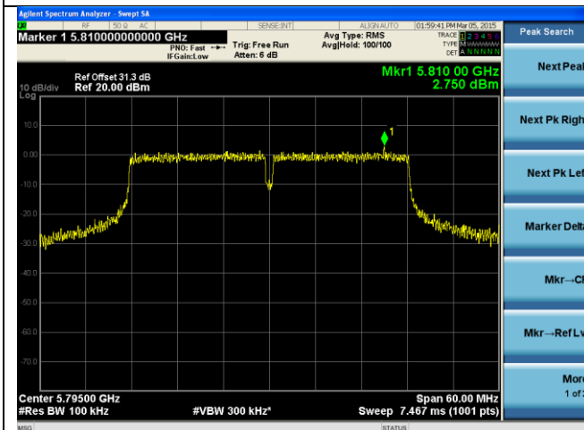
PSD-802.11n HT40-5795M-chain1
