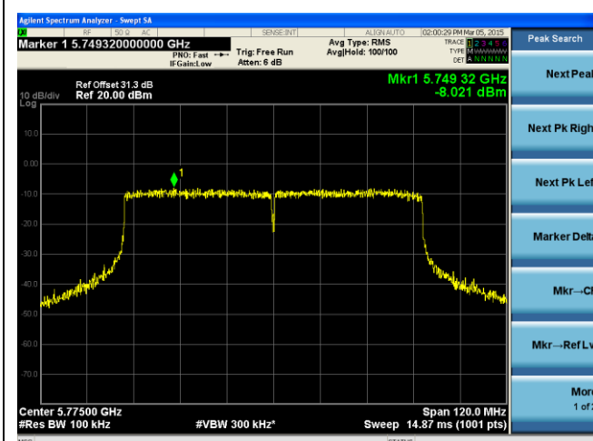
PSD-802.11ac-5775M-chain1
