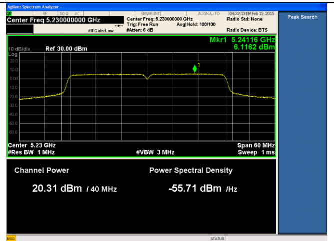
PSD-802.11n HT40-5230M-chain2
