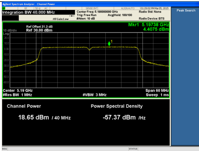
PSD-802.11n HT40-5190M-chain1
