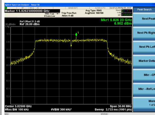
PSD-802.11n HT20-5825M-chain1
