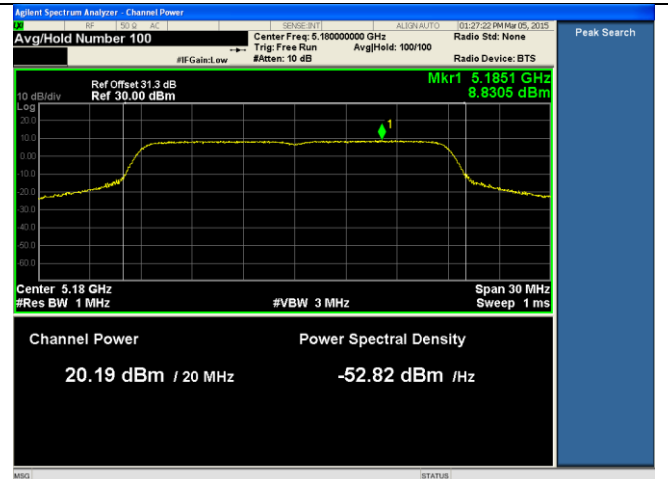
PSD-802.11n HT20-5180M-chain2
