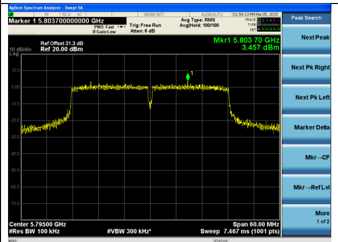
PSD-802.11n HT40-5795M-chain2
