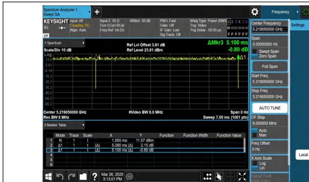
NTVN-11AX20MIMO-Ant1-5220-52Tone-RU39
