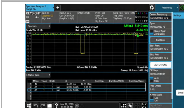
NTVN-11AX20MIMO-Ant1-5260-106Tone-RU53
