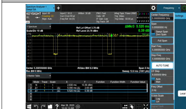
NTVN-11AX20MIMO-Ant1-5300-52Tone-RU39
