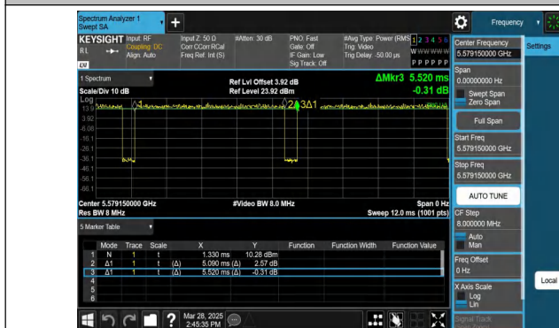
NTVN-11AX20MIMO-Ant1-5580-52Tone-RU39
