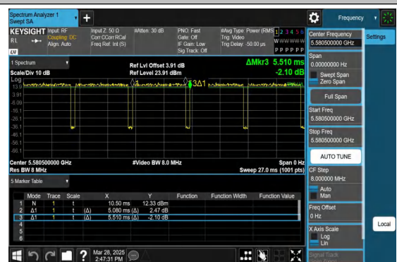
NTVN-11AX20MIMO-Ant2-5580-52Tone-RU39
