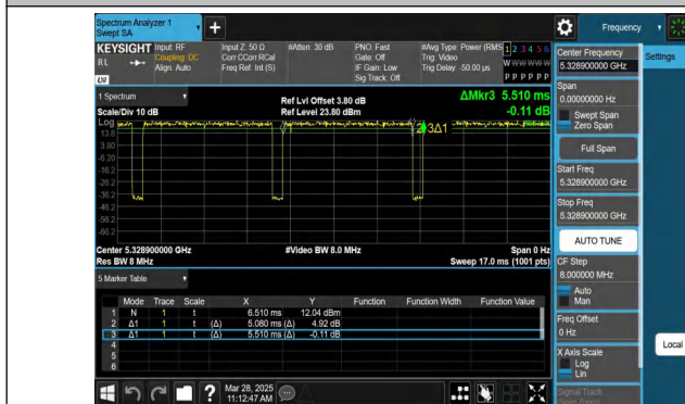
NTVN-11AX20MIMO-Ant1-5320-106Tone-RU54
