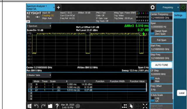
NTVN-11AX20MIMO-Ant2-5220-106Tone-RU53
