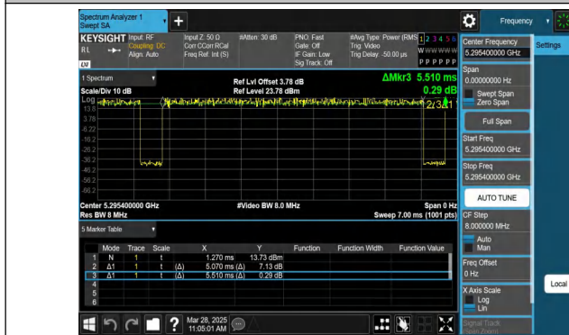
NTVN-11AX20MIMO-Ant1-5300-106Tone-RU53
