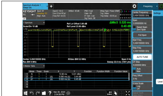
NTVN-11AX20MIMO-Ant1-5500-106Tone-RU53
