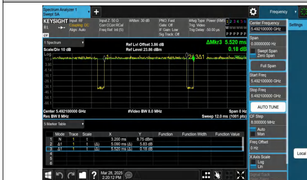
NTVN-11AX20MIMO-Ant1-5500-52Tone-RU37
