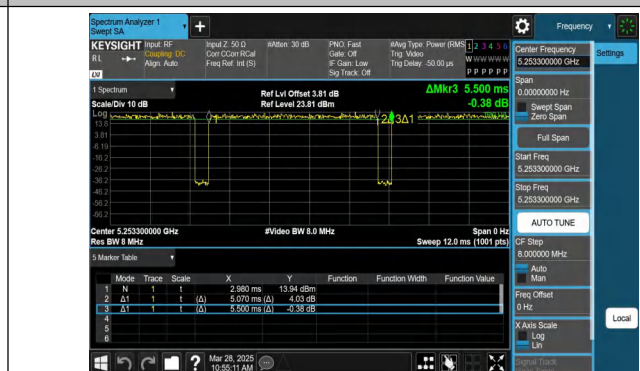
NTVN-11AX20MIMO-Ant2-5260-106Tone-RU53
