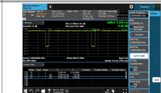
NTVN-11AX20MIMO-Ant2-5300-52Tone-RU39
