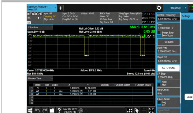
NTVN-11AX20MIMO-Ant1-5580-106Tone-RU53
