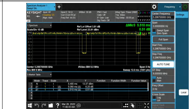
NTVN-11AX20MIMO-Ant2-5300-106Tone-RU53
