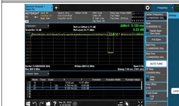
NTVN-11AX20MIMO-Ant1-5260-26Tone-RU0
