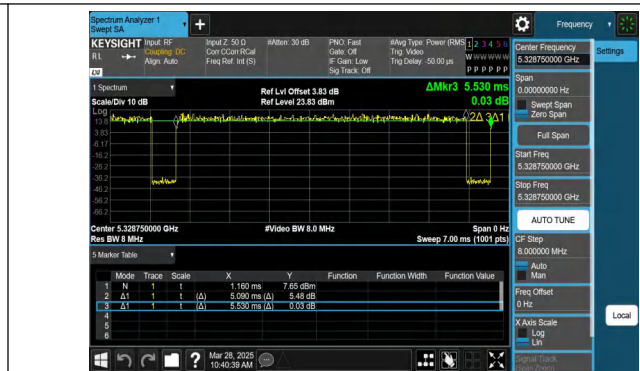
NTVN-11AX20MIMO-Ant2-5320-52Tone-RU40
