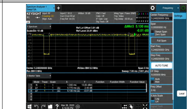
NTVN-11AX20MIMO-Ant2-5260-26Tone-RU0
