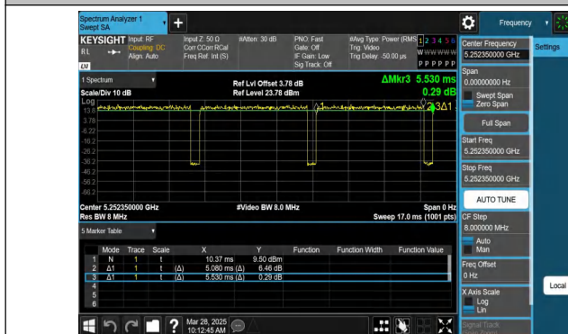
NTVN-11AX20MIMO-Ant1-5260-52Tone-RU37
