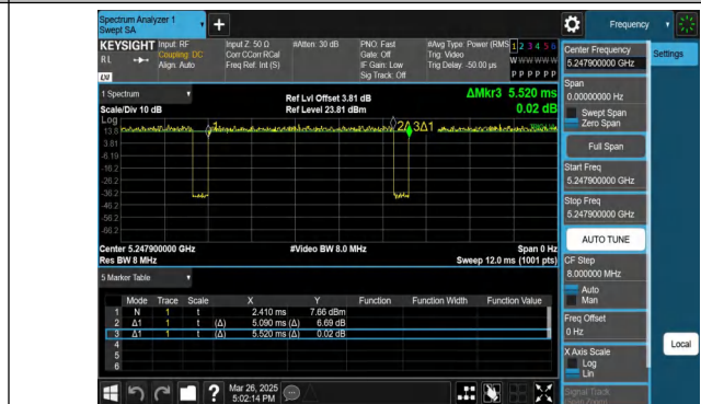
NTVN-11AX20MIMO-Ant2-5240-52Tone-RU40
