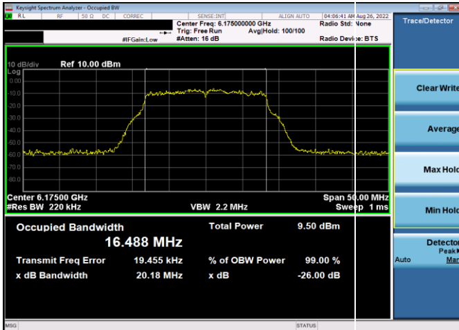
Plot 7-81. 26dB & 99% Bandwidth Plot Antenna WF5t (20MHz 802.11a (UNII Band 5) – Ch. 45, 24Mbps)
