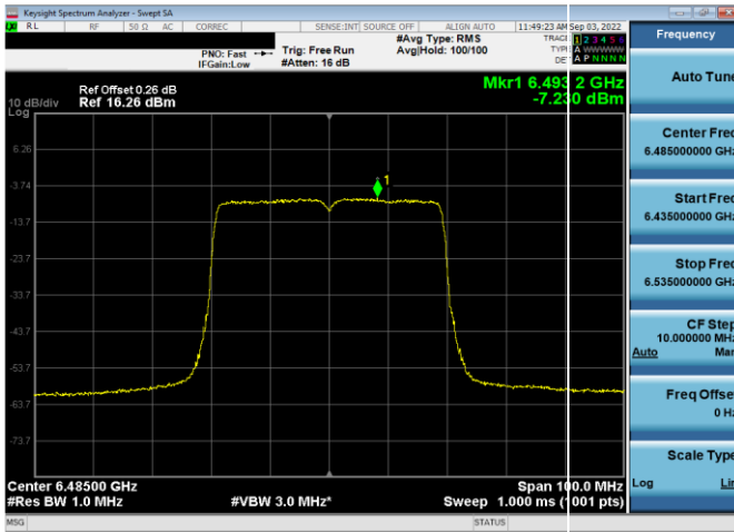
Plot 7-128. Power Spectral Density Plot Antenna WF5t (40MHz 802.11ax (UNII Band 6) – Ch. 107, MCS2)
