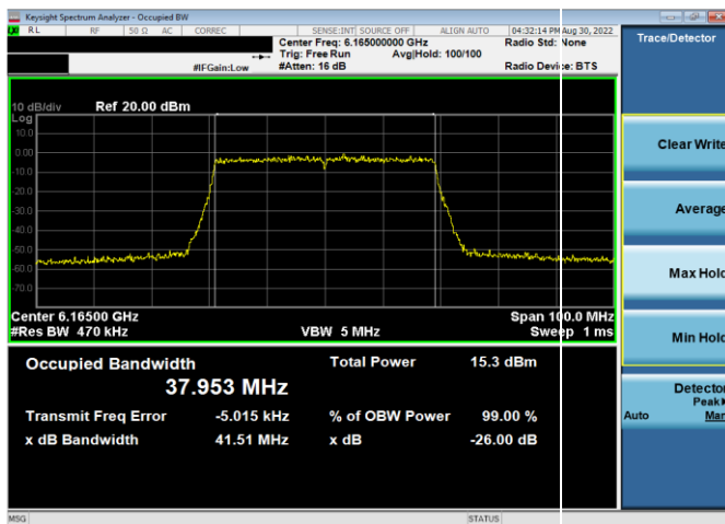
Plot 7-83. 26dB & 99% Bandwidth Plot Antenna WF5t (40MHz 802.11ax (UNII Band 5) – Ch. 43, MCS4)
