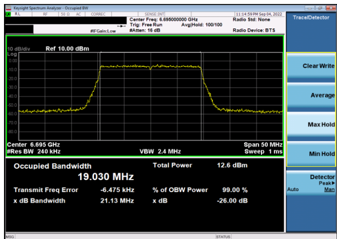
Plot 7-72. 26dB & 99% Bandwidth Plot Antenna WF5t (20MHz 802.11ax (UNII Band 7) – Ch. 149, MCS2)
