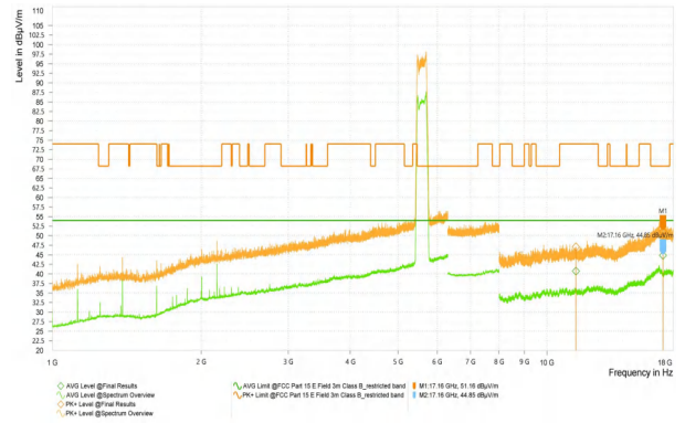
Wi-Fi 5G_11A_5785_High
