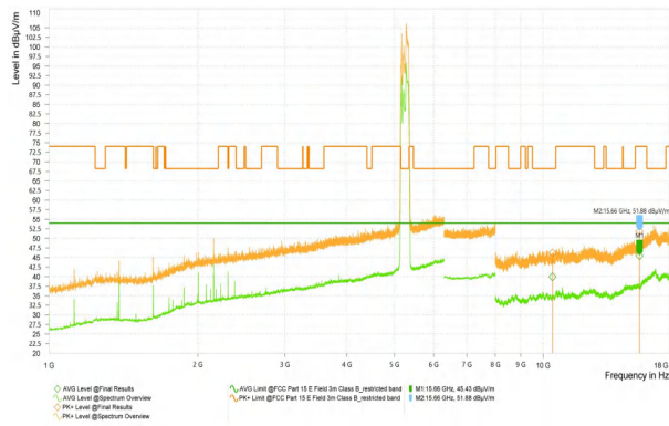
Wi-Fi 5G_11N20_5260_High
