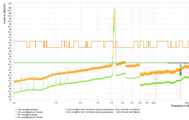
Wi-Fi 5G_11AC80_5530_High
