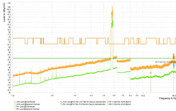
Wi-Fi 5G_11AC80_5210_High
