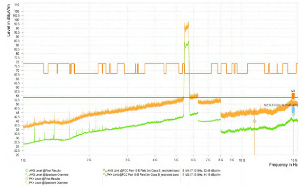
Wi-Fi 5G_11N40_5795_High
