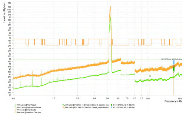
Wi-Fi 5G_11N40_5270_High
