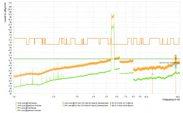
Wi-Fi 5G_11A_5720_High
