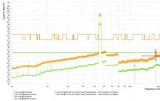
Wi-Fi 5G_11N40_5670_High
