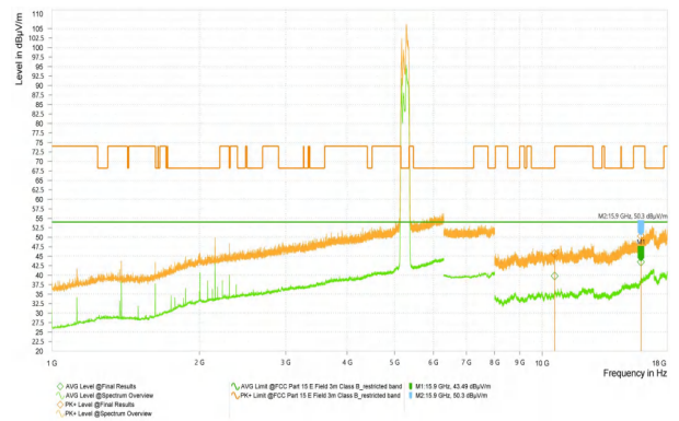
Wi-Fi 5G_11N20_5500_High
