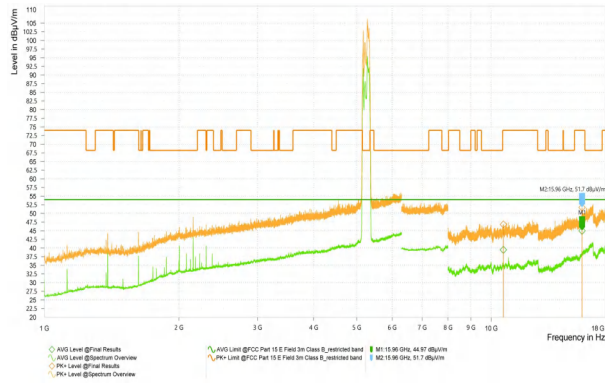
Wi-Fi 5G_11N20_5580_High
