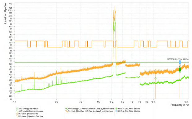
Wi-Fi 5G_11N20_5240_High
