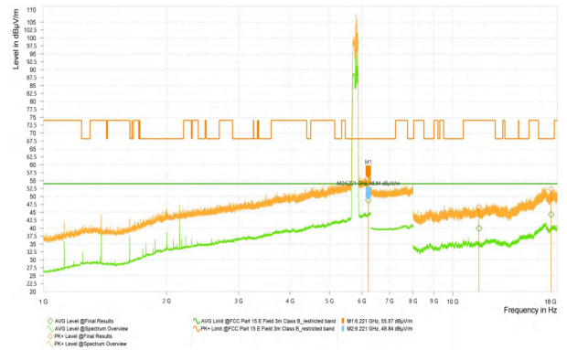
Wi-Fi 5G_11AC80_5290_High
