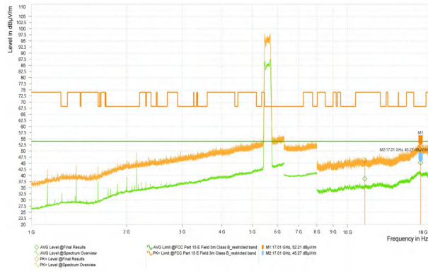
Wi-Fi 5G_11N40_5755_High
