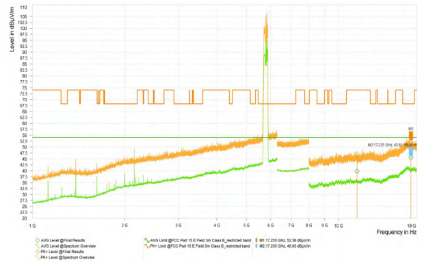
Wi-Fi 5G_11N20_5825_High
