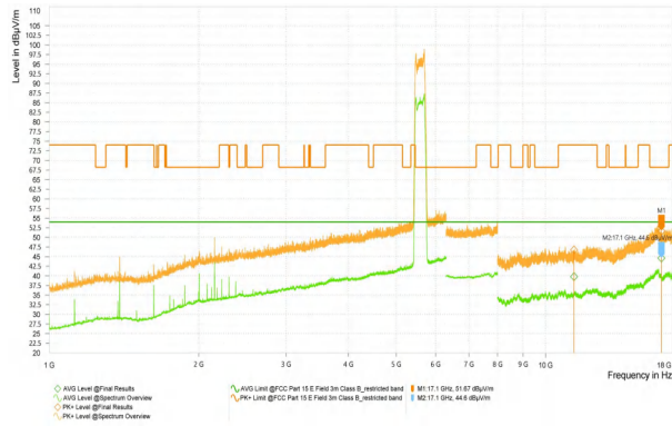
Wi-Fi 5G_11A_5745_High
