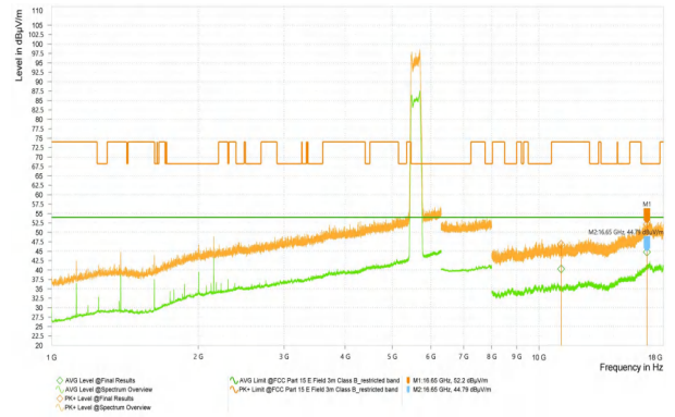
Wi-Fi 5G_11N40_5710_High
