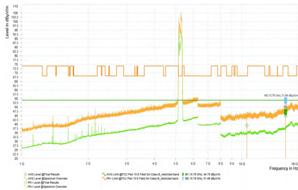
Wi-Fi 5G_11N20_5320_High
