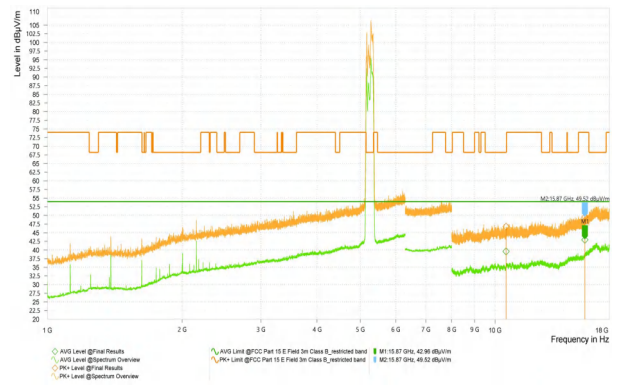
Wi-Fi 5G_11AC80_5610_High
