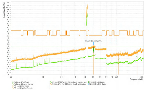
Wi-Fi 5G_11N40_5310_High
