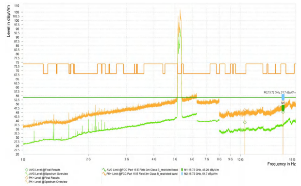
Wi-Fi 5G_11N20_5300_High
