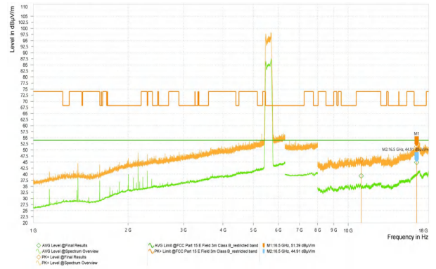
Wi-Fi 5G_11N20_5700_High
