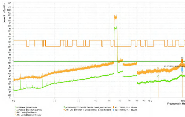
Wi-Fi 5G_11N20_5785_High
