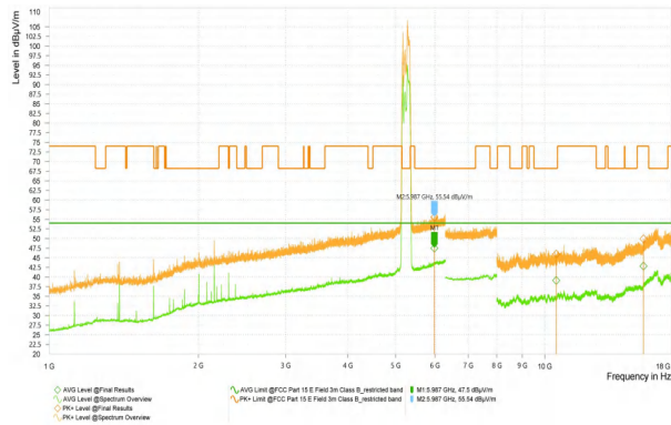
Wi-Fi 5G_11N40_5510_High
