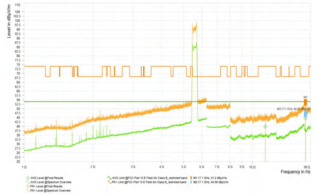
Wi-Fi 5G_11N20_5745_High
