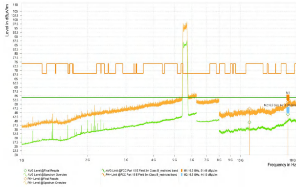
Wi-Fi 5G_11A_5700_High
