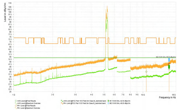
Wi-Fi 5G_11N40_5550_High
