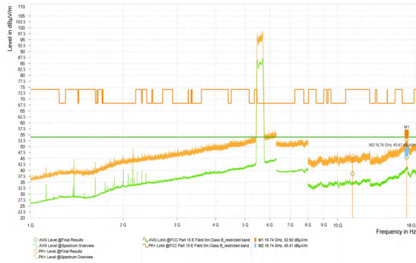
Wi-Fi 5G_11N20_5720_High
