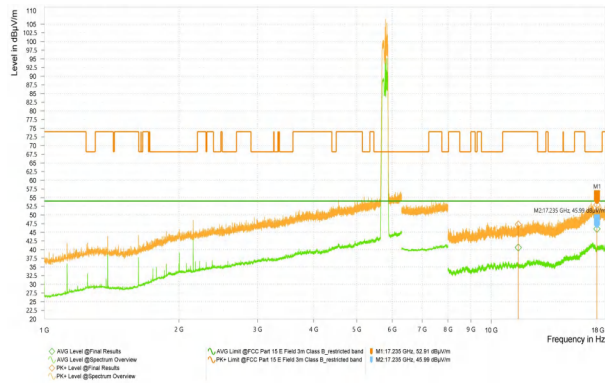
Wi-Fi 5G_11A_5825_High
