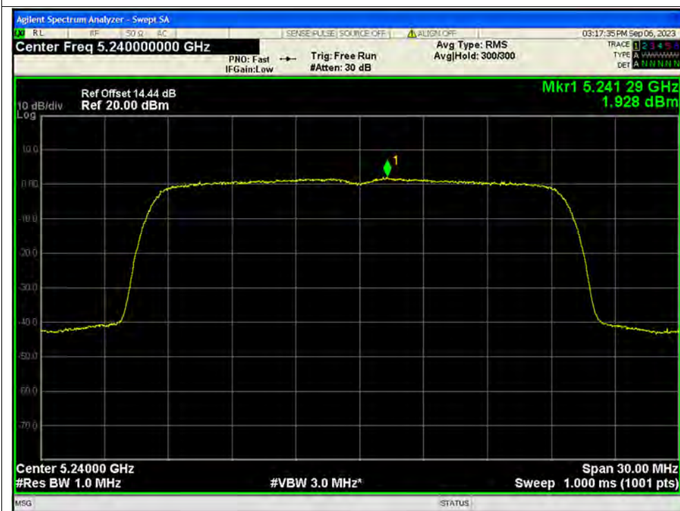
PSD NVNT ax20 5240MHz Ant2 MIMO
