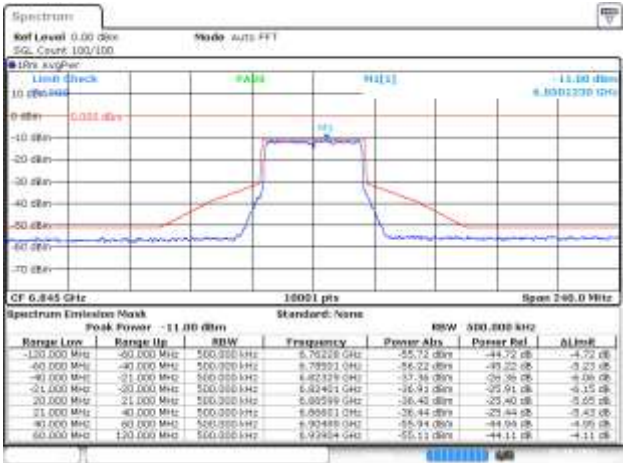
MIMO B-802.11ax/be-40MHz-Ch179-MCS0
