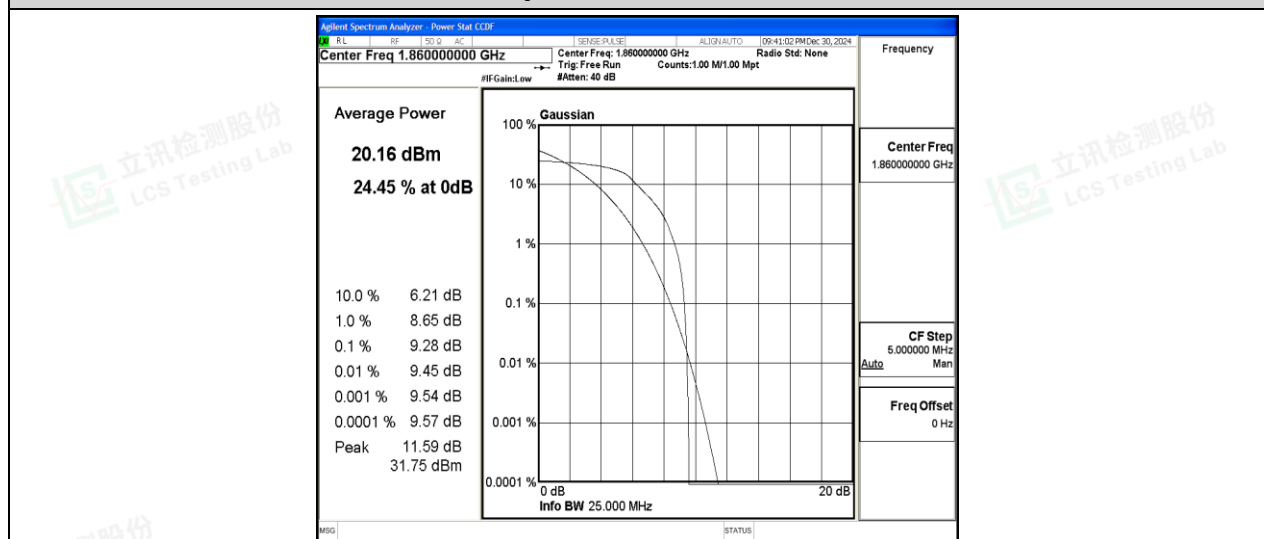
Band2-20MHz-16QAM-18700-6-0-Low-9.28-&lt;=13-PASS
