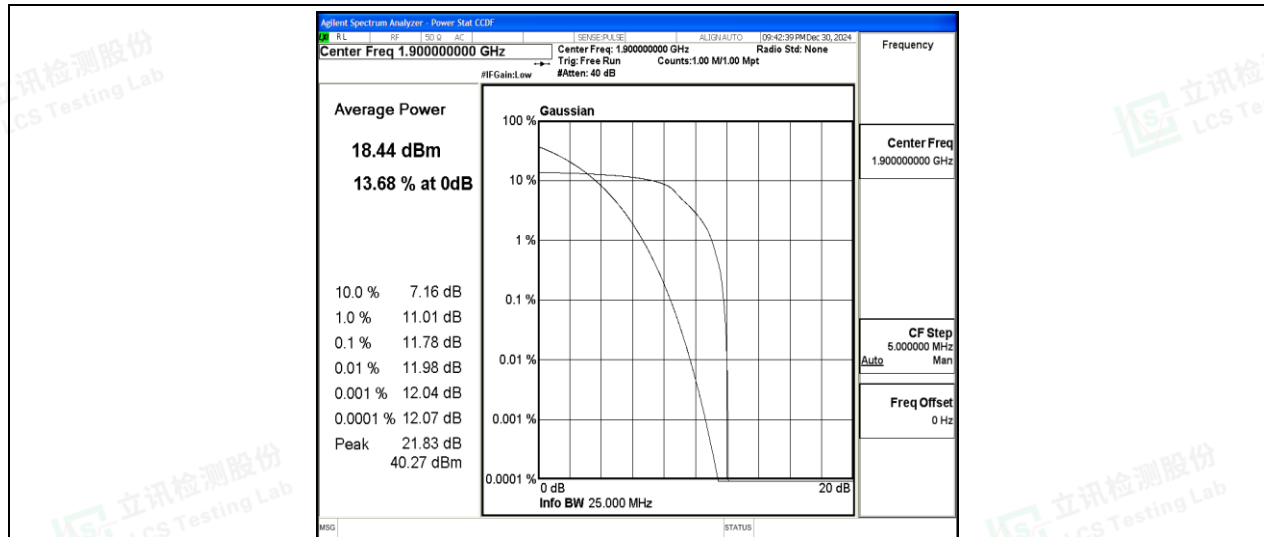
Band2-20MHz-QPSK-19100-6-0-High-11.78-&lt;=13-PASS
