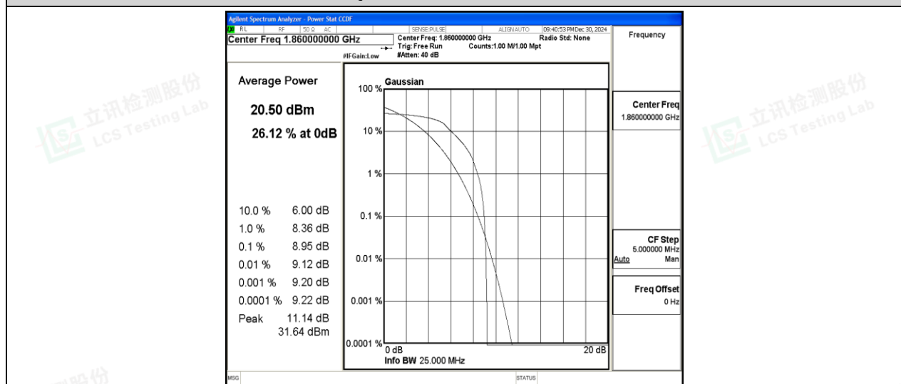
Band2-20MHz-QPSK-18700-6-0-Low-8.95-&lt;=13-PASS
