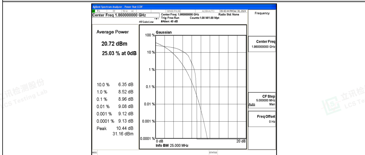
Band2-20MHz-16QAM-18700-1-0-Low-8.96-&lt;=13-PASS
