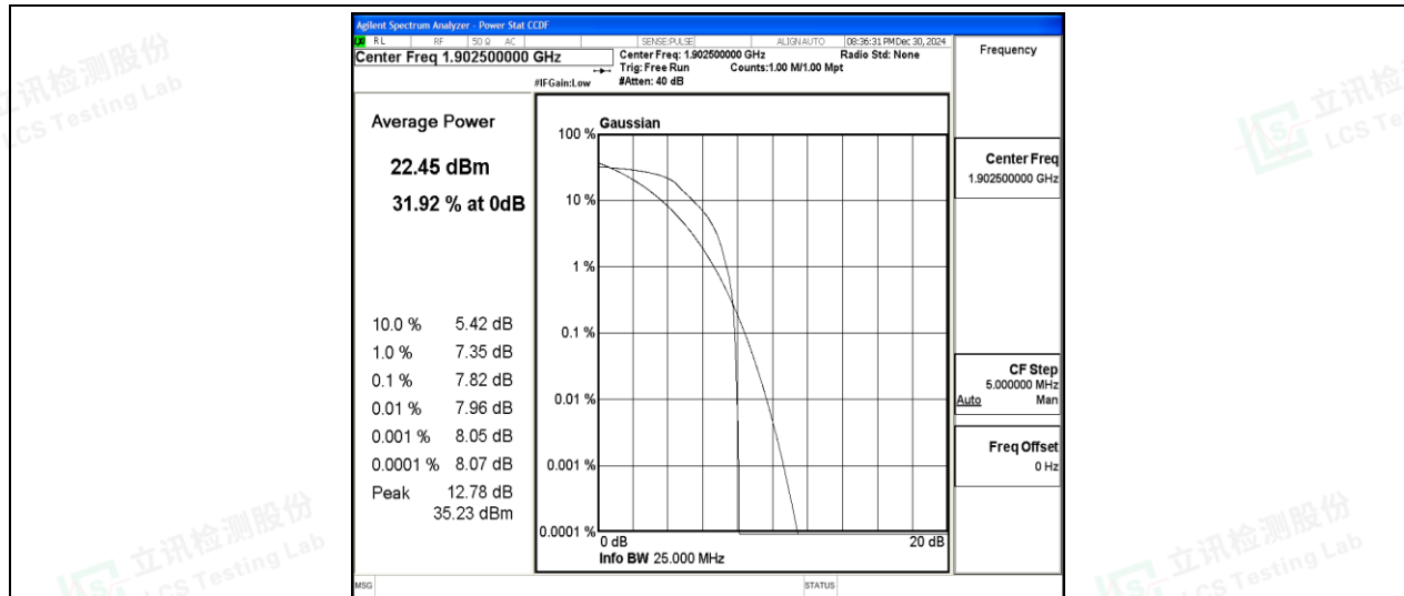
Band2-15MHz-16QAM-19125-6-0-High-7.82-&lt;=13-PASS
