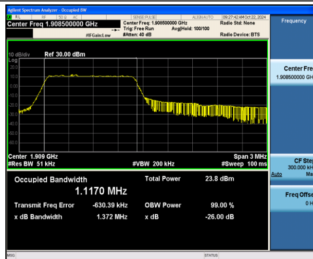
Band2-3MHz-QPSK-19185-6-0-Low-1.1170-1.372-PASS
