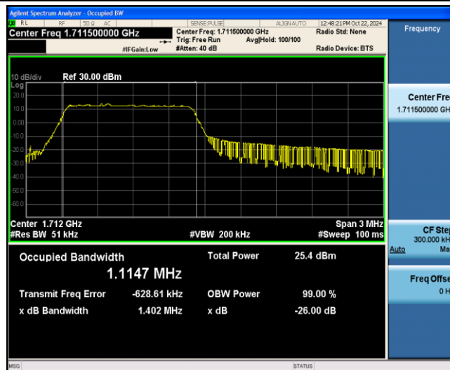
Band4-3MHz-QPSK-19965-6-0-Low-1.1147-1.402-PASS
