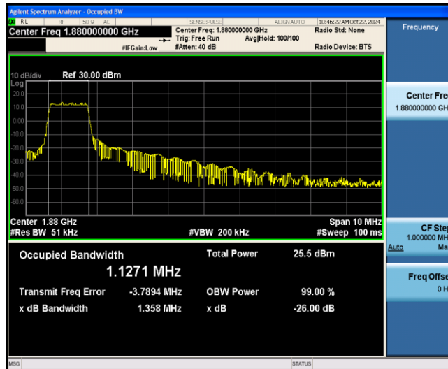
Band2-10MHz-16QAM-18900-6-0-Low-1.1271-1.358-PASS
