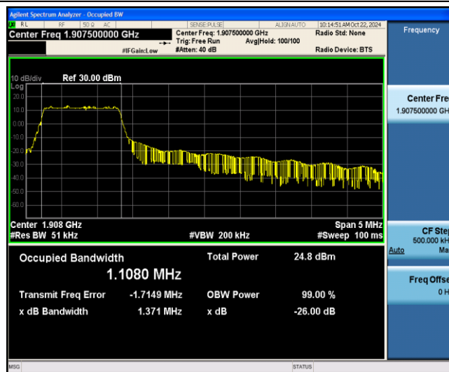
Band2-5MHz-QPSK-19175-6-0-Low-1.1080-1.371-PASS
