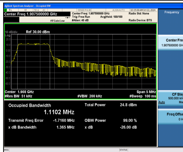
Band2-5MHz-16QAM-19175-6-0-Low-1.1102-1.365-PASS
