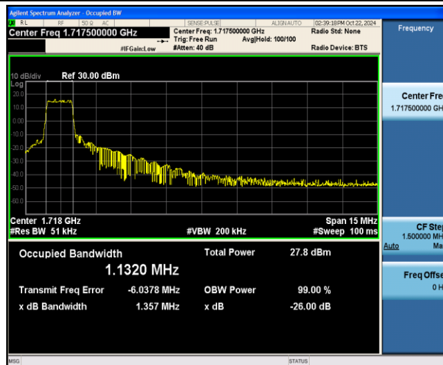
Band4-15MHz-QPSK-20025-6-0-Low-1.1320-1.357-PASS
