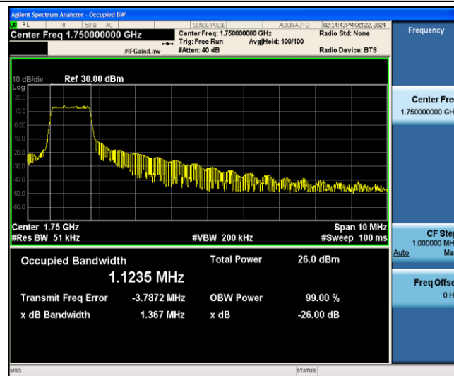
Band4-10MHz-QPSK-20350-6-0-Low-1.1235-1.367-PASS
