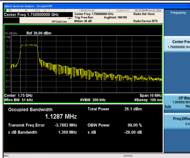
Band4-10MHz-16QAM-20350-6-0-Low-1.1287-1.369-PASS
