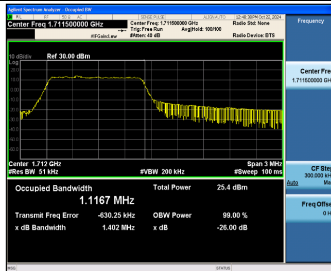
Band4-3MHz-16QAM-19965-6-0-Low-1.1167-1.402-PASS
