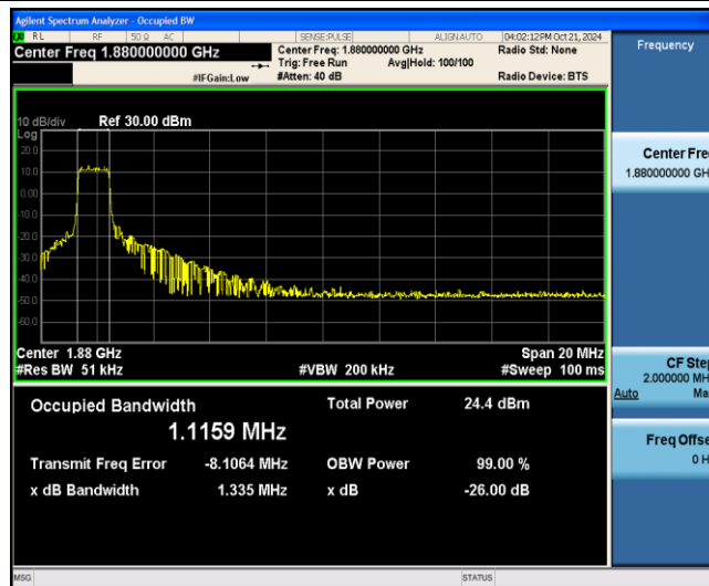
Band2-20MHz-16QAM-18900-6-0-Low-1.1159-1.335-PASS
