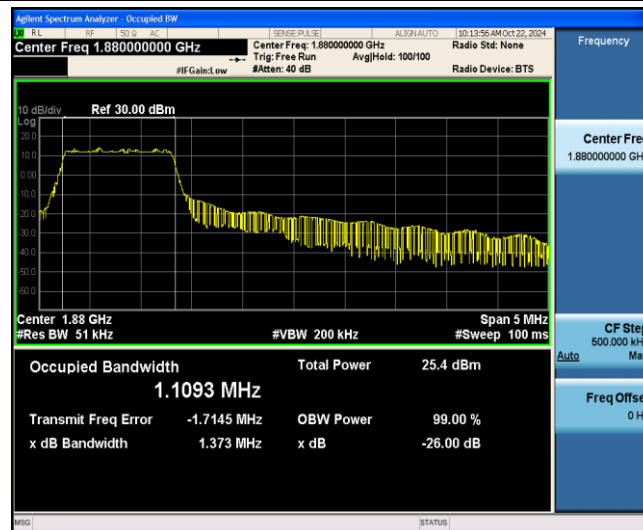
Band2-5MHz-16QAM-18900-6-0-Low-1.1093-1.373-PASS
