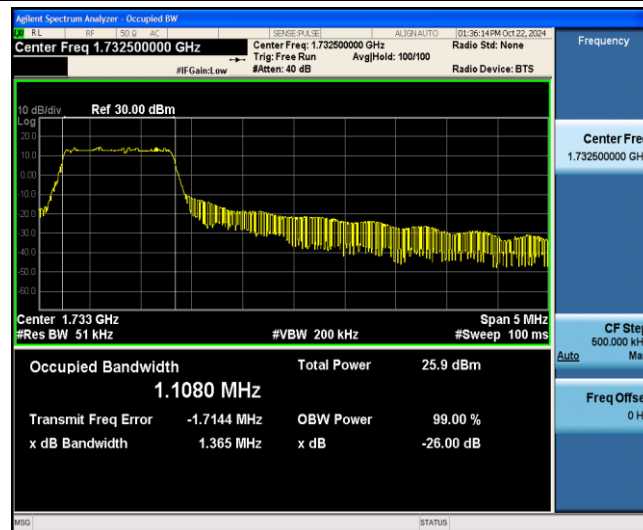
Band4-5MHz-QPSK-20175-6-0-Low-1.1080-1.365-PASS
