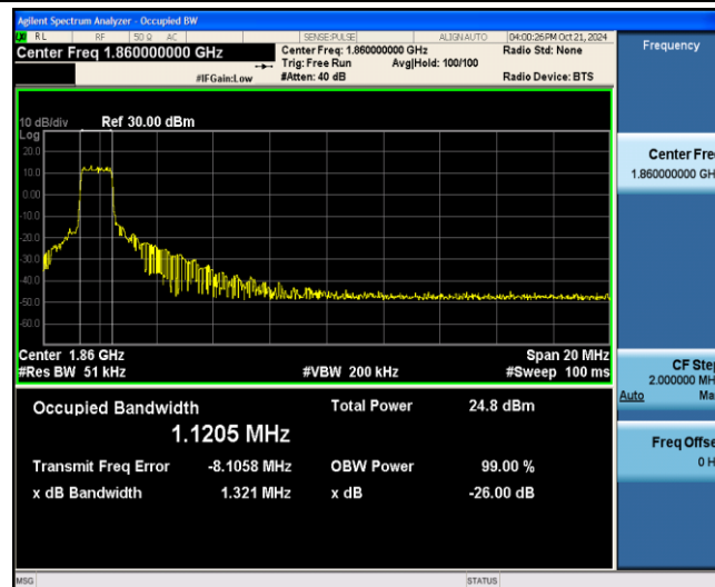
Band2-20MHz-QPSK-18700-6-0-Low-1.1205-1.321-PASS
