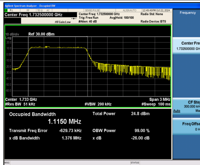
Band4-3MHz-16QAM-20175-6-0-Low-1.1150-1.376-PASS
