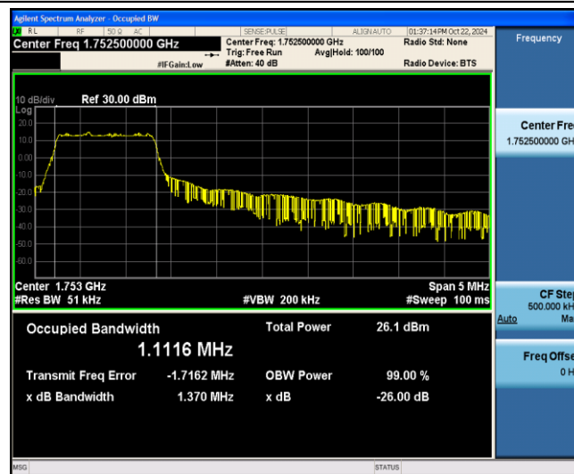
Band4-5MHz-QPSK-20375-6-0-Low-1.1116-1.370-PASS
