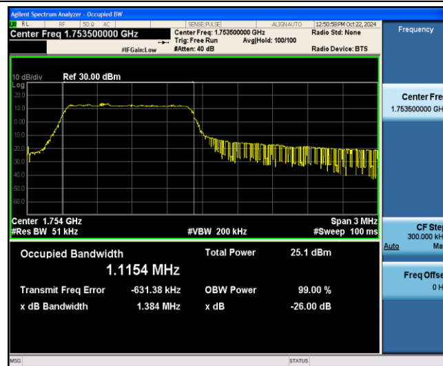
Band4-3MHz-16QAM-20385-6-0-Low-1.1154-1.384-PASS
