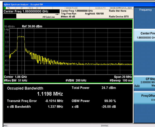
Band2-20MHz-16QAM-18700-6-0-Low-1.1198-1.337-PASS
