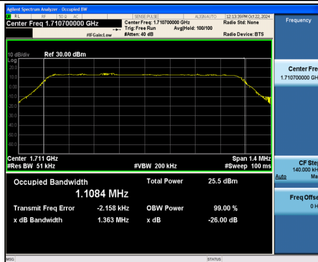
Band4-1.4MHz-QPSK-19957-6-0-Low-1.1084-1.363-PASS
