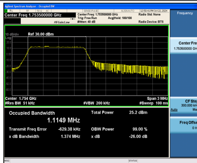
Band4-3MHz-QPSK-20385-6-0-Low-1.1149-1.374-PASS
