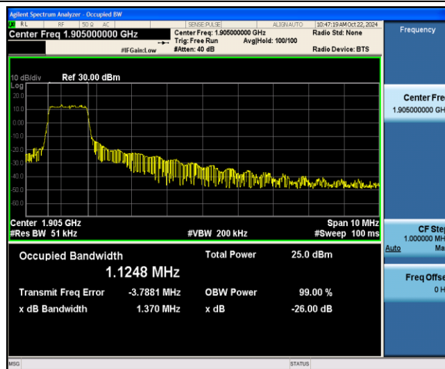
Band2-10MHz-16QAM-19150-6-0-Low-1.1248-1.370-PASS
