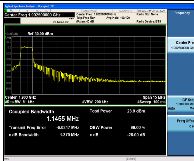
Band2-15MHz-QPSK-19125-6-0-Low-1.1455-1.370-PASS
