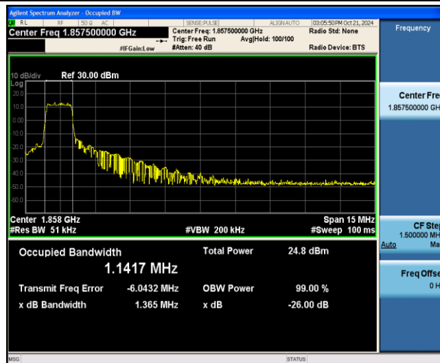
Band2-15MHz-QPSK-18675-6-0-Low-1.1417-1.365-PASS
