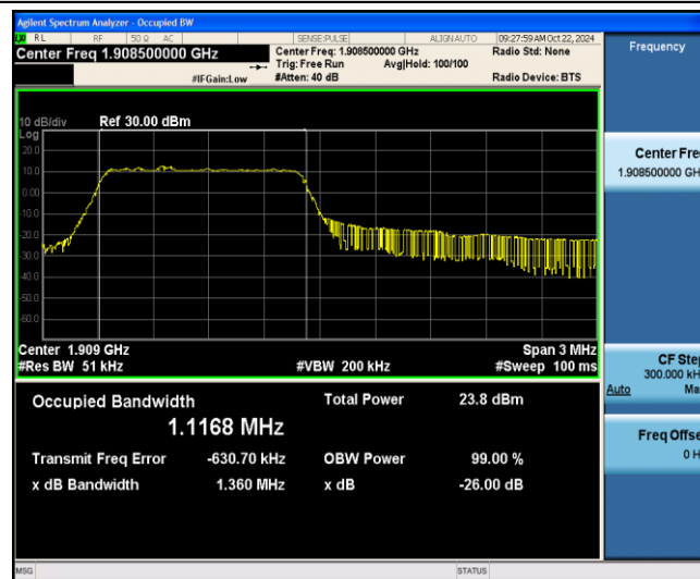
Band2-3MHz-16QAM-19185-6-0-Low-1.1168-1.360-PASS
