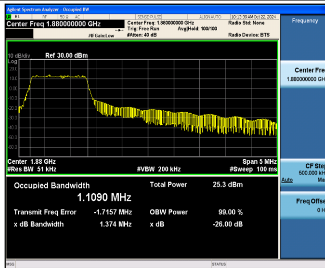
Band2-5MHz-QPSK-18900-6-0-Low-1.1090-1.374-PASS
