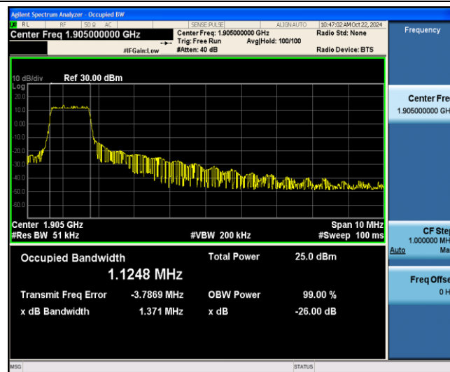
Band2-10MHz-QPSK-19150-6-0-Low-1.1248-1.371-PASS
