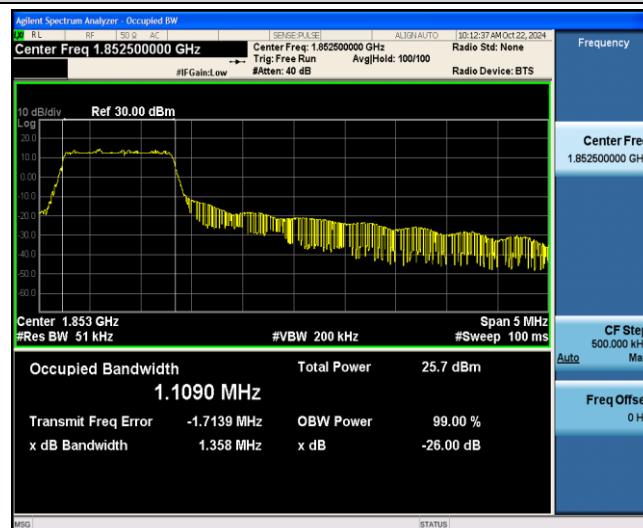
Band2-5MHz-QPSK-18625-6-0-Low-1.1090-1.358-PASS
