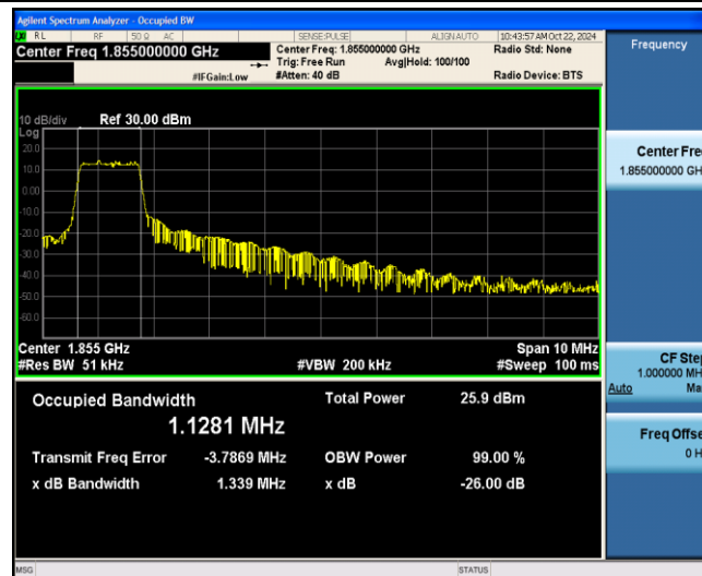
Band2-10MHz-16QAM-18650-6-0-Low-1.1281-1.339-PASS
