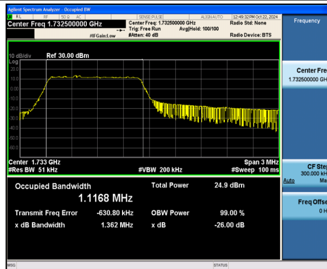
Band4-3MHz-QPSK-20175-6-0-Low-1.1168-1.362-PASS
