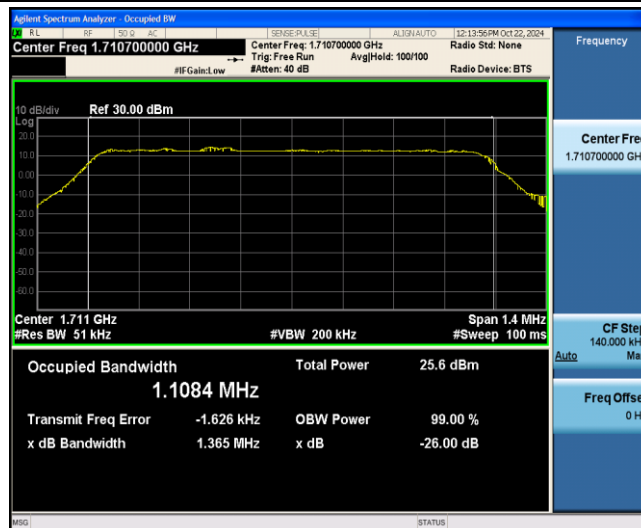
Band4-1.4MHz-16QAM-19957-6-0-Low-1.1084-1.365-PASS
