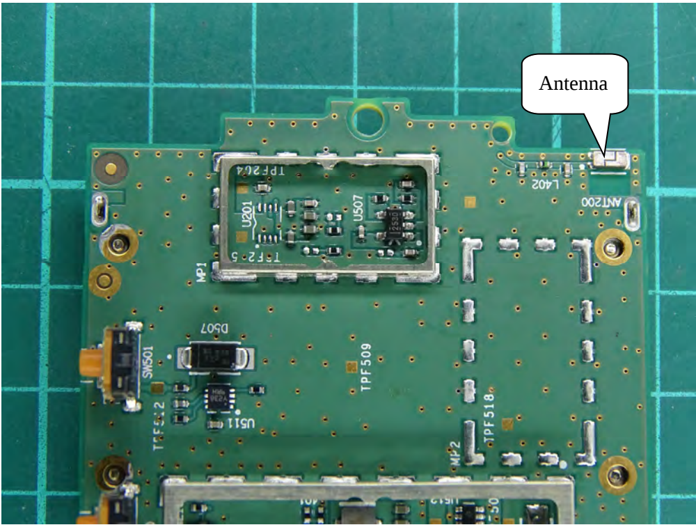
(22) EUT Photo
