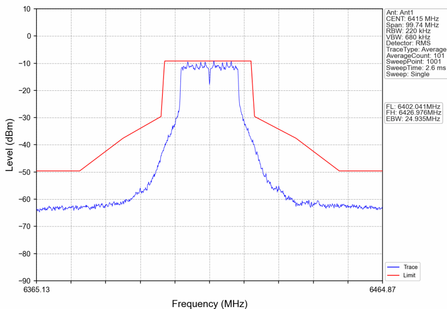
802.11ax(HEW20)_HCH_6415MHz_RU242_Left_Ant1_NTNV
