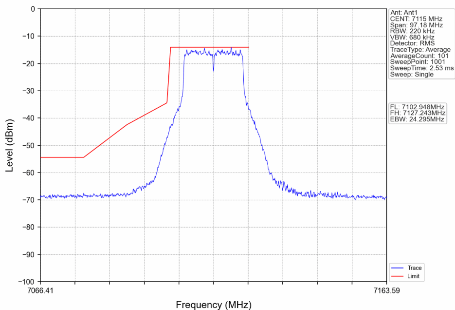
802.11ax(HEW20)_HCH_7115MHz_RU242_Left_Ant1_NTNV
