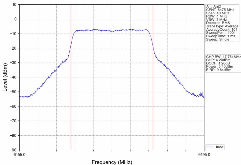
802.11ax(HEW20)_MCH_6475MHz_RU242_Left_Ant2_NTNV
