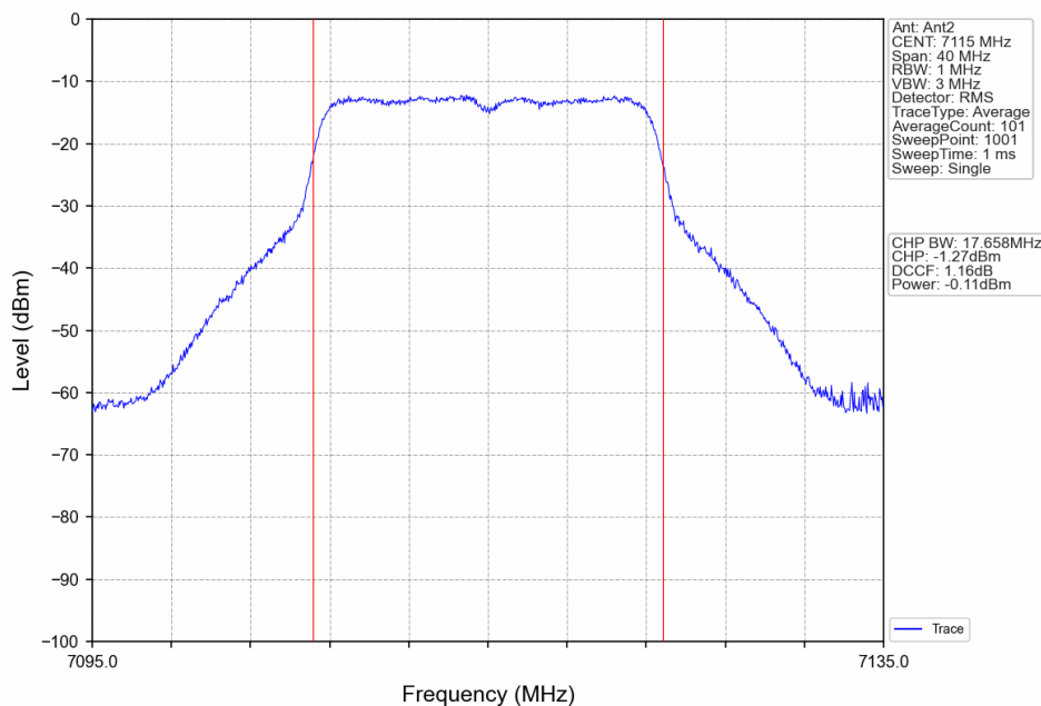
802.11ax(HEW20)_HCH_7115MHz_RU242_Left_Ant2_NTNV
