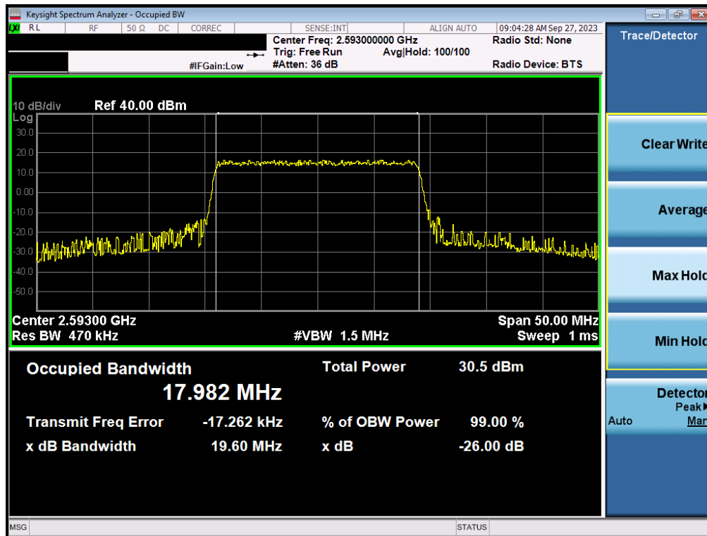
Plot 7-25. Occupied Bandwidth Plot (LTE Band 41(PC3)/38 - 20MHz 16-QAM - Full RB)
