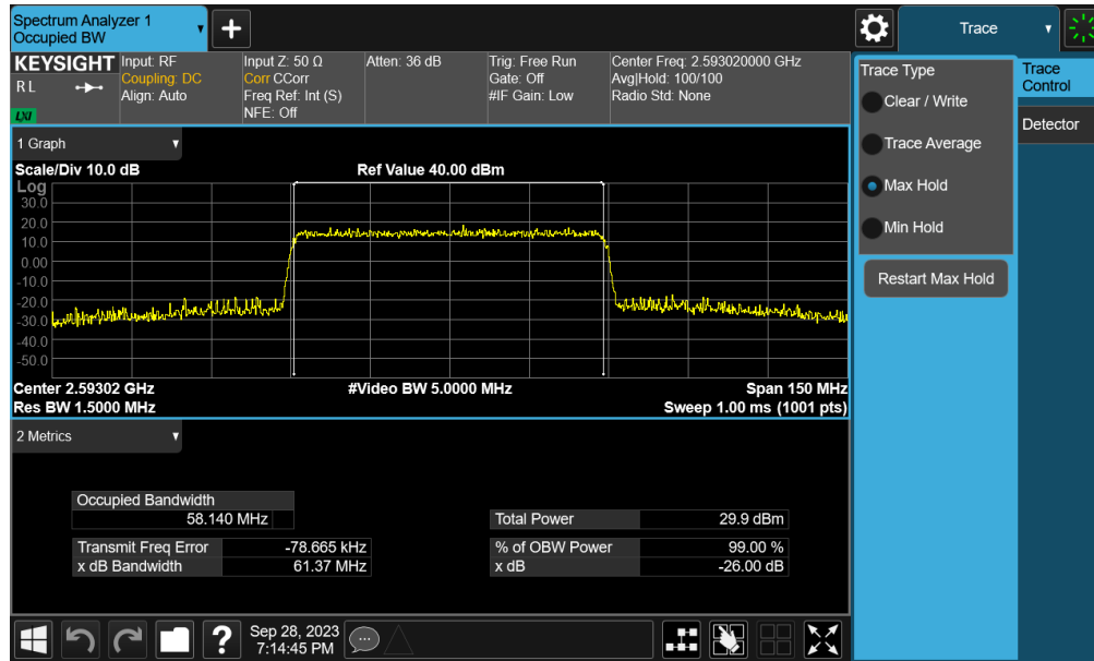
Plot 7-46. Occupied Bandwidth Plot (NR Band n41 - 60MHz 16-QAM - Full RB)
