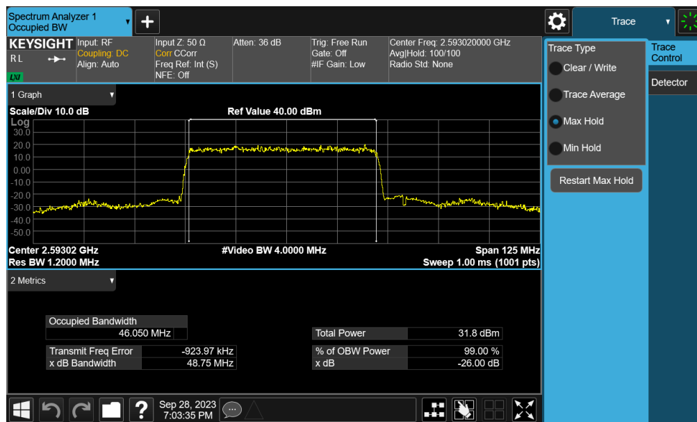
Plot 7-47. Occupied Bandwidth Plot (NR Band n41 - 50MHz \pi/2 BPSK - Full RB)
