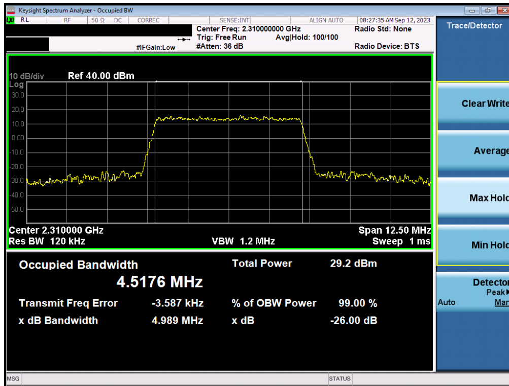
Plot 7-7. Occupied Bandwidth Plot (LTE Band 30 - 5MHz 16-QAM - Full RB)
