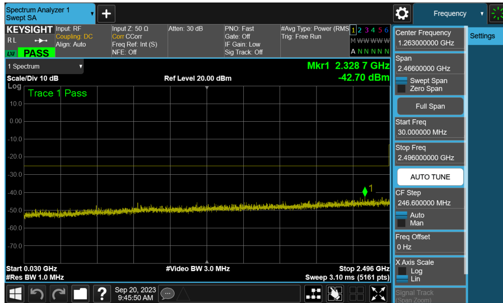
Plot 7-78. Conducted Spurious Plot (ULCA LTE B41(PC3) - 20MHz QPSK - RB Size 1, RB Offset 0 - High Channel Ant1)
