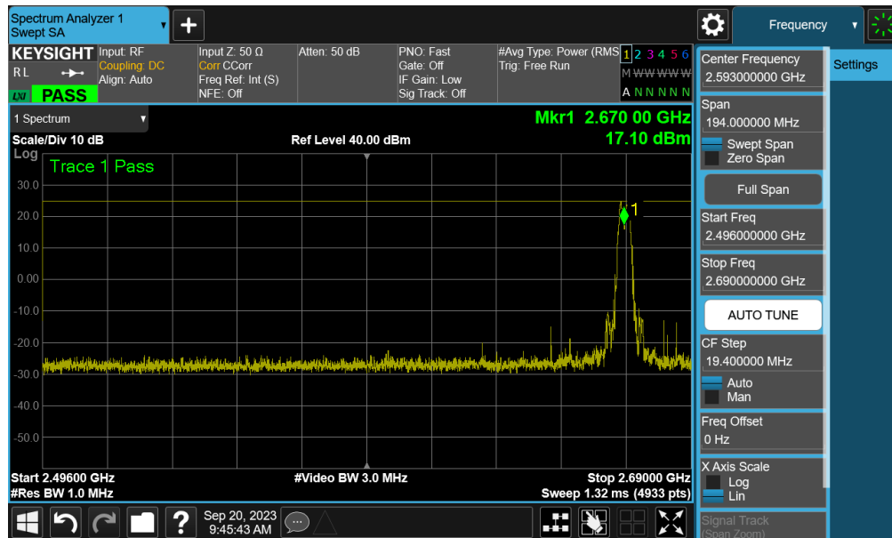
Plot 7-79. Conducted Spurious Plot (ULCA LTE B41(PC3) - 20MHz QPSK - RB Size 1, RB Offset 0 - High Channel Ant1)
