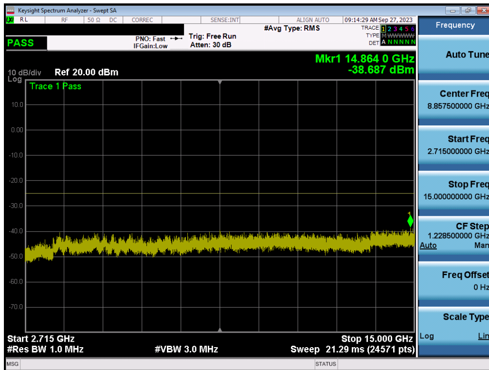
Plot 7-76. Conducted Spurious Plot (LTE Band 41(PC3)/38 - 20MHz QPSK - RB Size 1, RB Offset 0 - High Channel)
