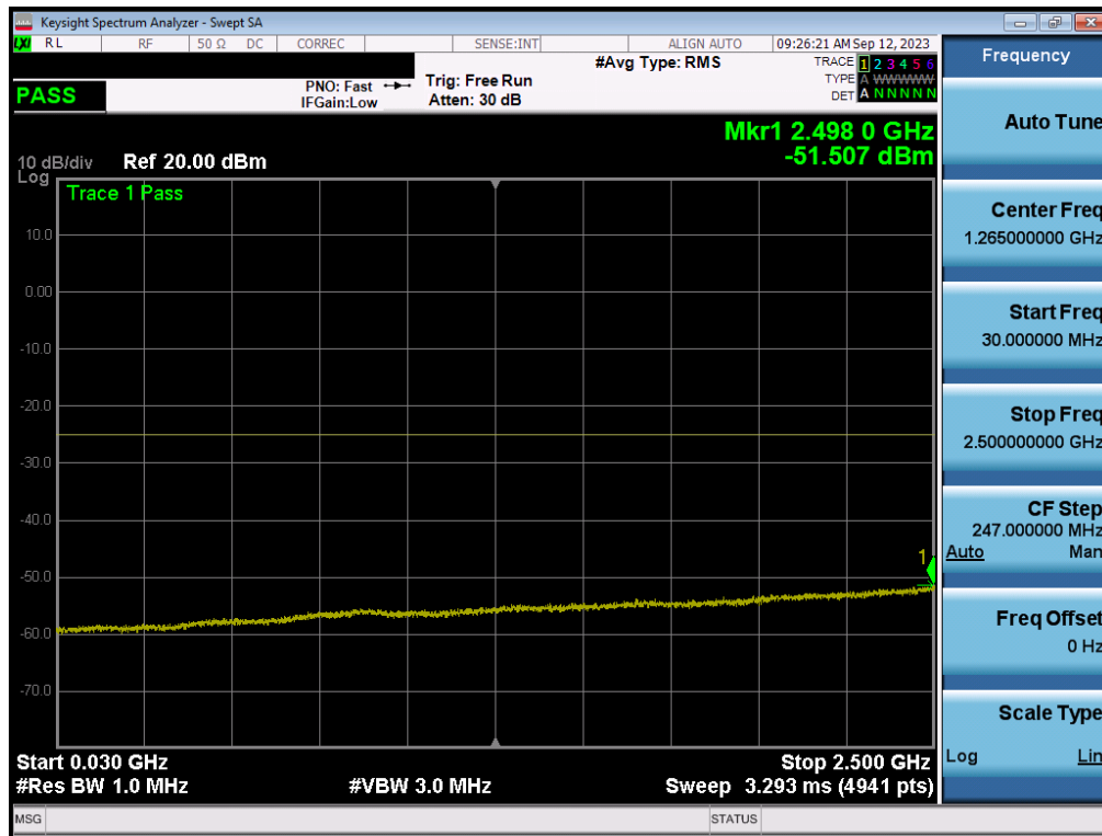
Plot 7-69. Conducted Spurious Plot (LTE Band 7 - 20MHz QPSK - RB Size 1, RB Offset 0 - High Channel)
