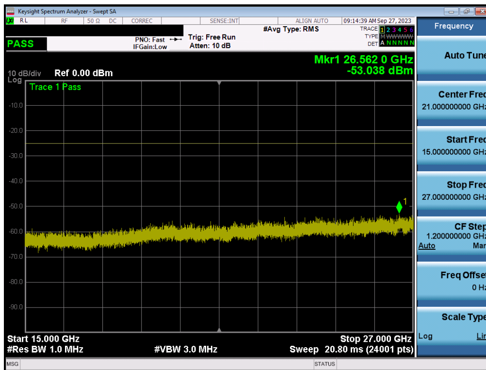
Plot 7-77. Conducted Spurious Plot (LTE Band 41(PC3)/38 - 20MHz QPSK - RB Size 1, RB Offset 0 - High Channel)
