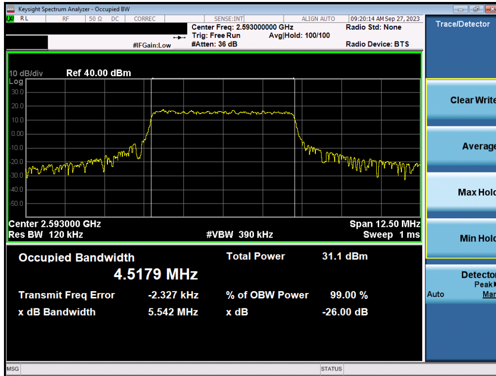
Plot 7-30. Occupied Bandwidth Plot (LTE Band 41(PC3)/38 - 5MHz QPSK - Full RB)
