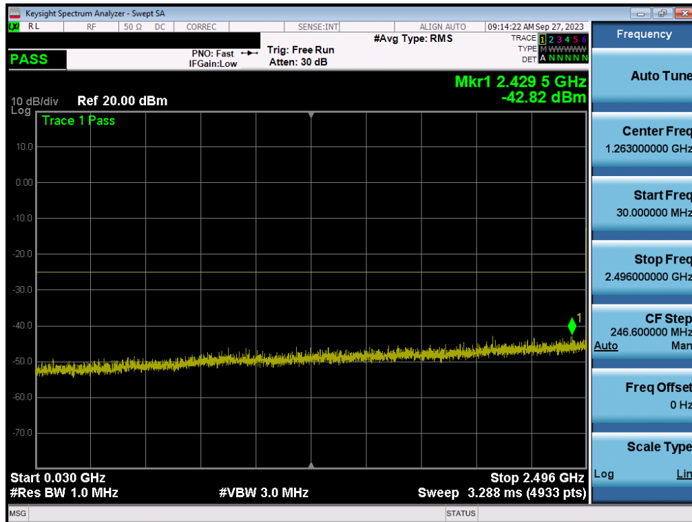
Plot 7-75. Conducted Spurious Plot (LTE Band 41(PC3)/38 - 20MHz QPSK - RB Size 1, RB Offset 0 - High Channel)
