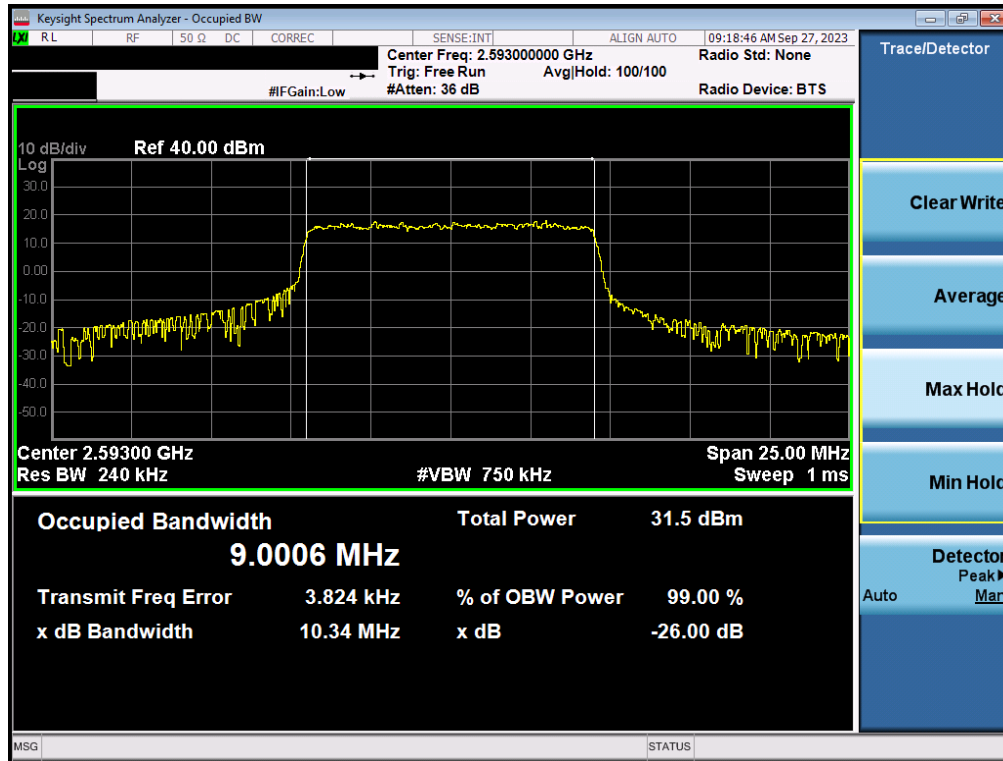
Plot 7-28. Occupied Bandwidth Plot (LTE Band 41(PC3)/38 - 10MHz QPSK - Full RB)
