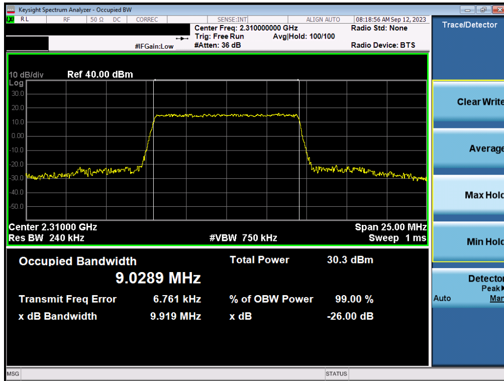
Plot 7-4. Occupied Bandwidth Plot (LTE Band 30 - 10MHz QPSK - Full RB)
