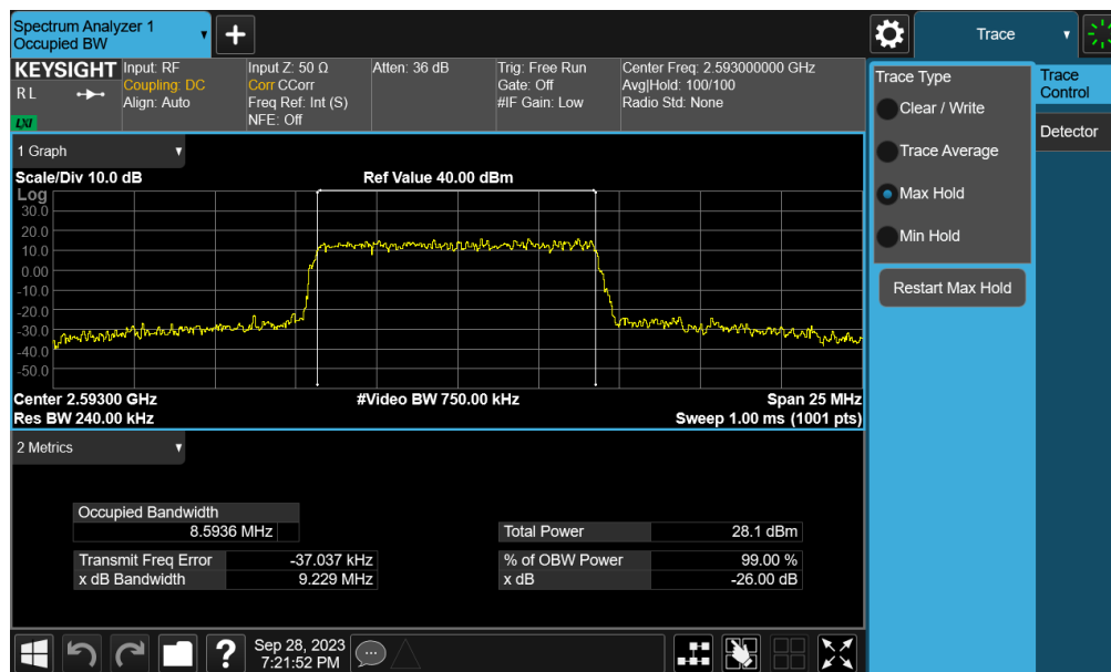
Plot 7-64. Occupied Bandwidth Plot (NR Band n41 - 10MHz 16-QAM - Full RB)
