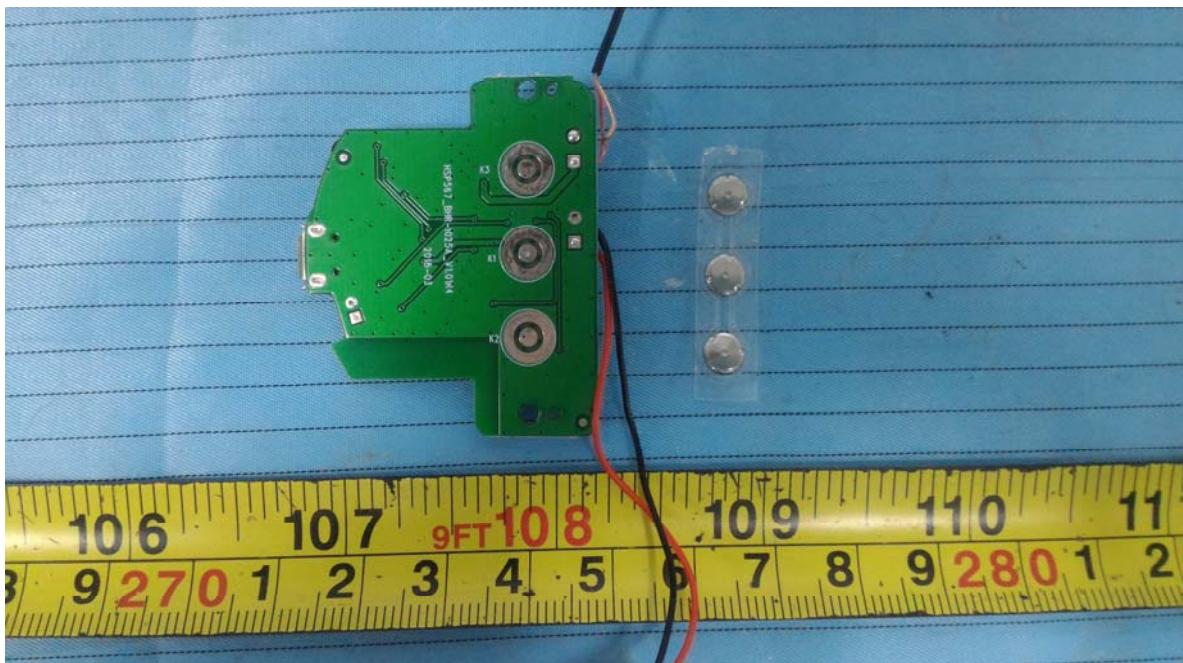
EUT – Mainboard Cover off View
