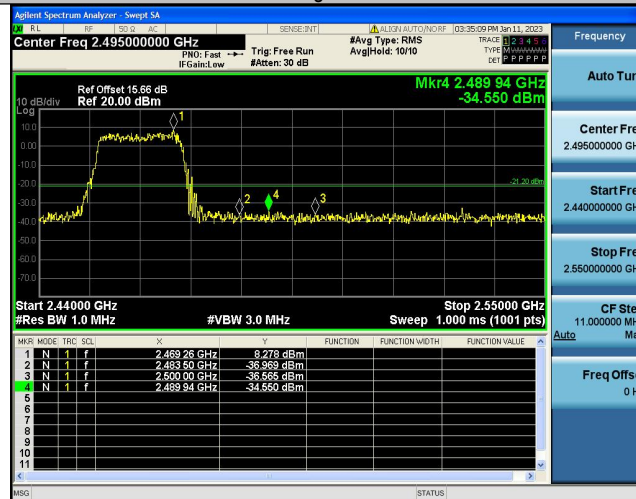
11N20SISO-Ant1-High-2462-AV-2483.500
