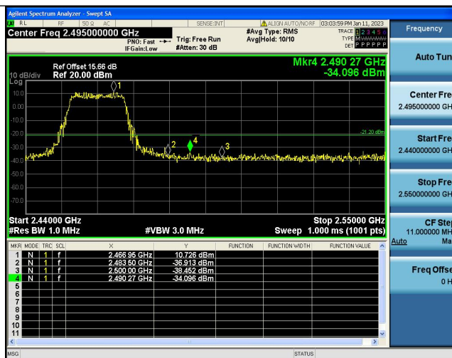
11G-Ant1-High-2462-AV-2483.500
