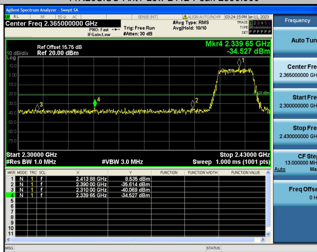
11N20SISO-Ant1-Low-2412-AV-2390.000
