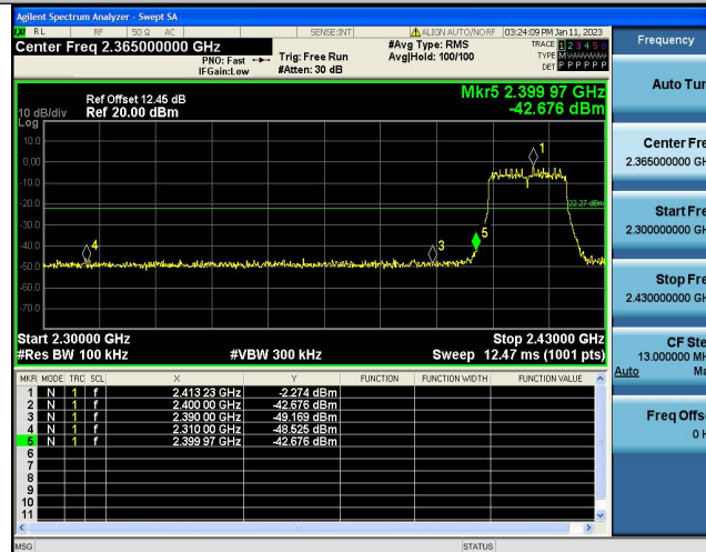
11N20SISO-Ant1-Low-2412--2.27
