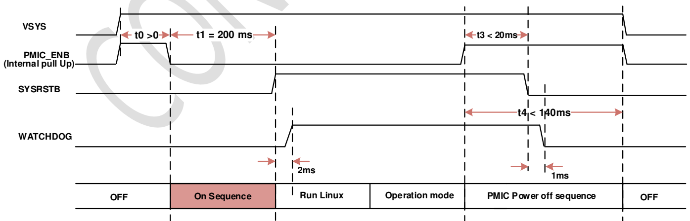
NAD Power On/Off Sequence
