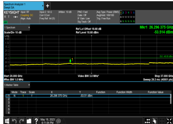
N48(20M)_CP- OFDM_QPSK_Edge_1RB_Left_High_CH
