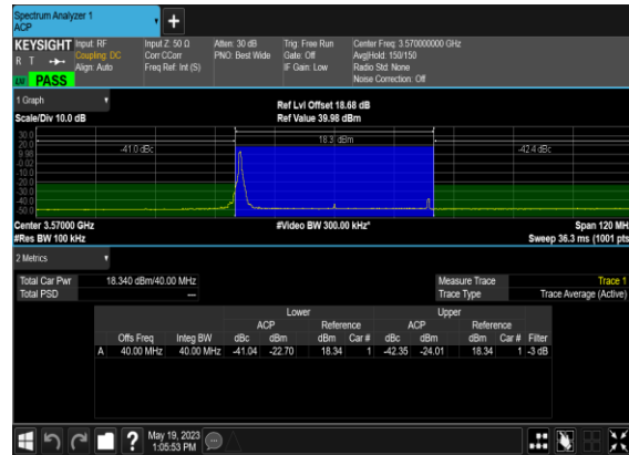
N48(40M)_CP-s- OFDM_QPSK_Edge_1RB_Left_Low_CH
