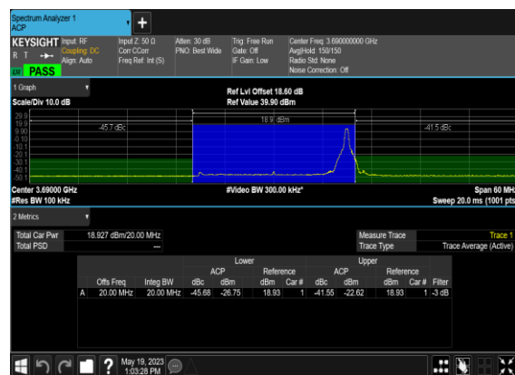
N48(20M)_CP-s- OFDM_QPSK_Edge_1RB_Right_High_C H
