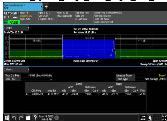
N48(40M)_CP-s- OFDM_QPSK_Edge_1RB_Right_Mid_CH
