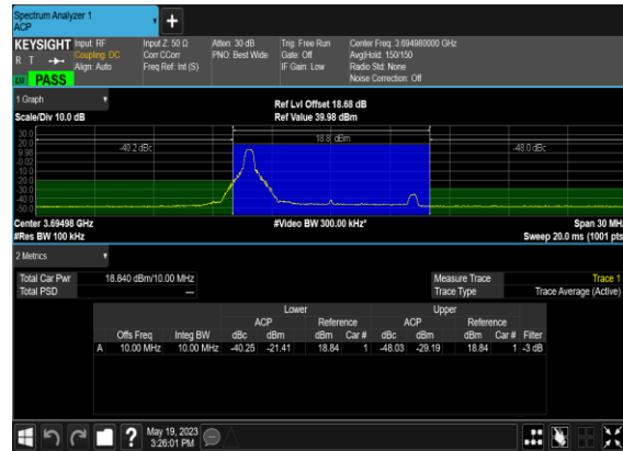
N48(10M)_CP-s- OFDM_QPSK_Edge_1RB_Left_High_CH
