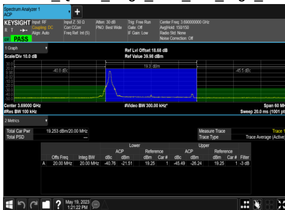
N48(20M)_CP-s- OFDM_QPSK_Edge_1RB_Left_High_CH
