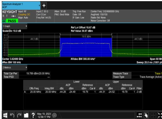
N48(20M)_CP-s- OFDM_QPSK_Outer_Full_Mid_CH
