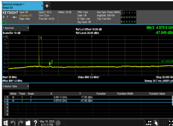
N48(20M)_CP- OFDM_QPSK_Edge_1RB_Left_High_CH
