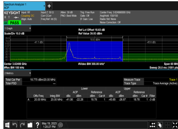
N48(20M)_CP-s- OFDM_QPSK_Edge_1RB_Left_Mid_CH
