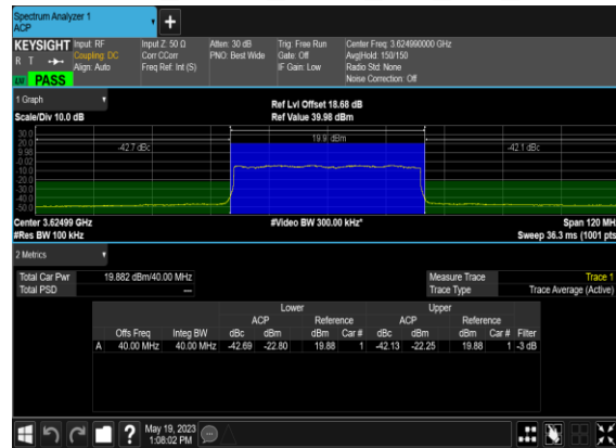
N48(40M)_CP-s- OFDM_QPSK_Outer_Full_Mid_CH
