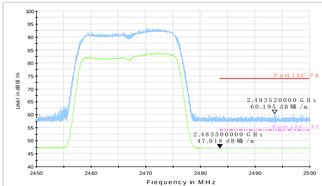
Fig.A.6.2.11 Transmitter Spurious Emission - Radiated (Power): 802.11n-HT20, ch12, 2.45 GHz - 2.50GHz
