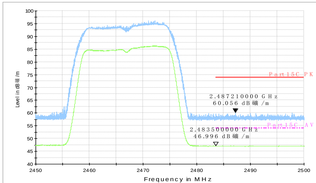
Fig.A.6.2.7 Transmitter Spurious Emission - Radiated (Power): 802.11g, ch12, 2.45 GHz - 2.50GHz
