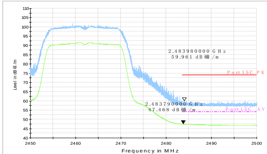
Fig.A.6.2.6 Transmitter Spurious Emission - Radiated (Power): 802.11g, ch11, 2.45 GHz - 2.50GHz
