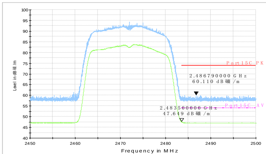
Fig.A.6.2.12 Transmitter Spurious Emission - Radiated (Power): 802.11n-HT20, ch13, 2.45 GHz - 2.50GHz
