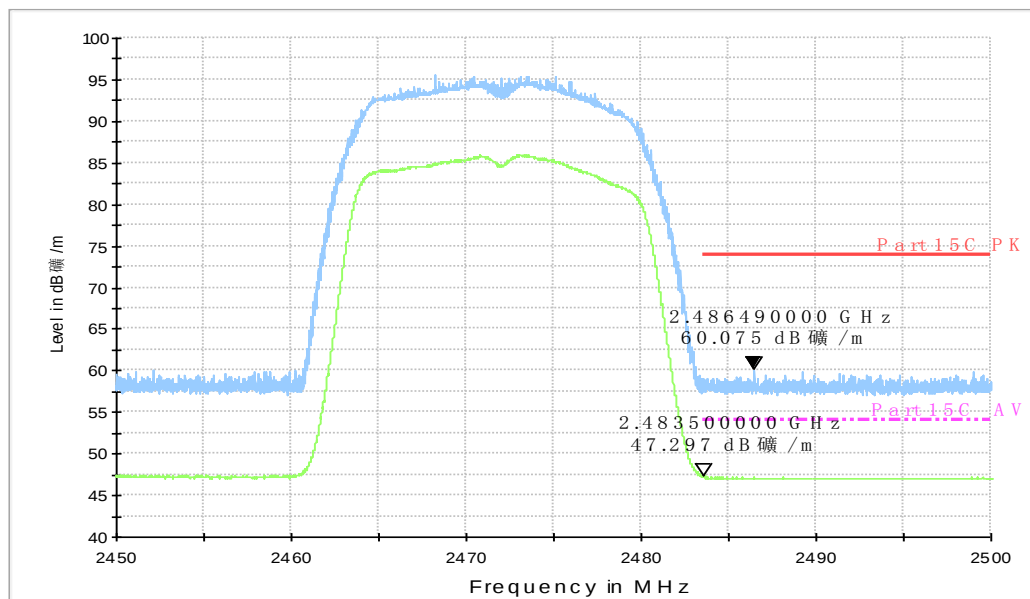
Fig.A.6.2.8 Transmitter Spurious Emission - Radiated (Power): 802.11g, ch13, 2.45 GHz - 2.50GHz
