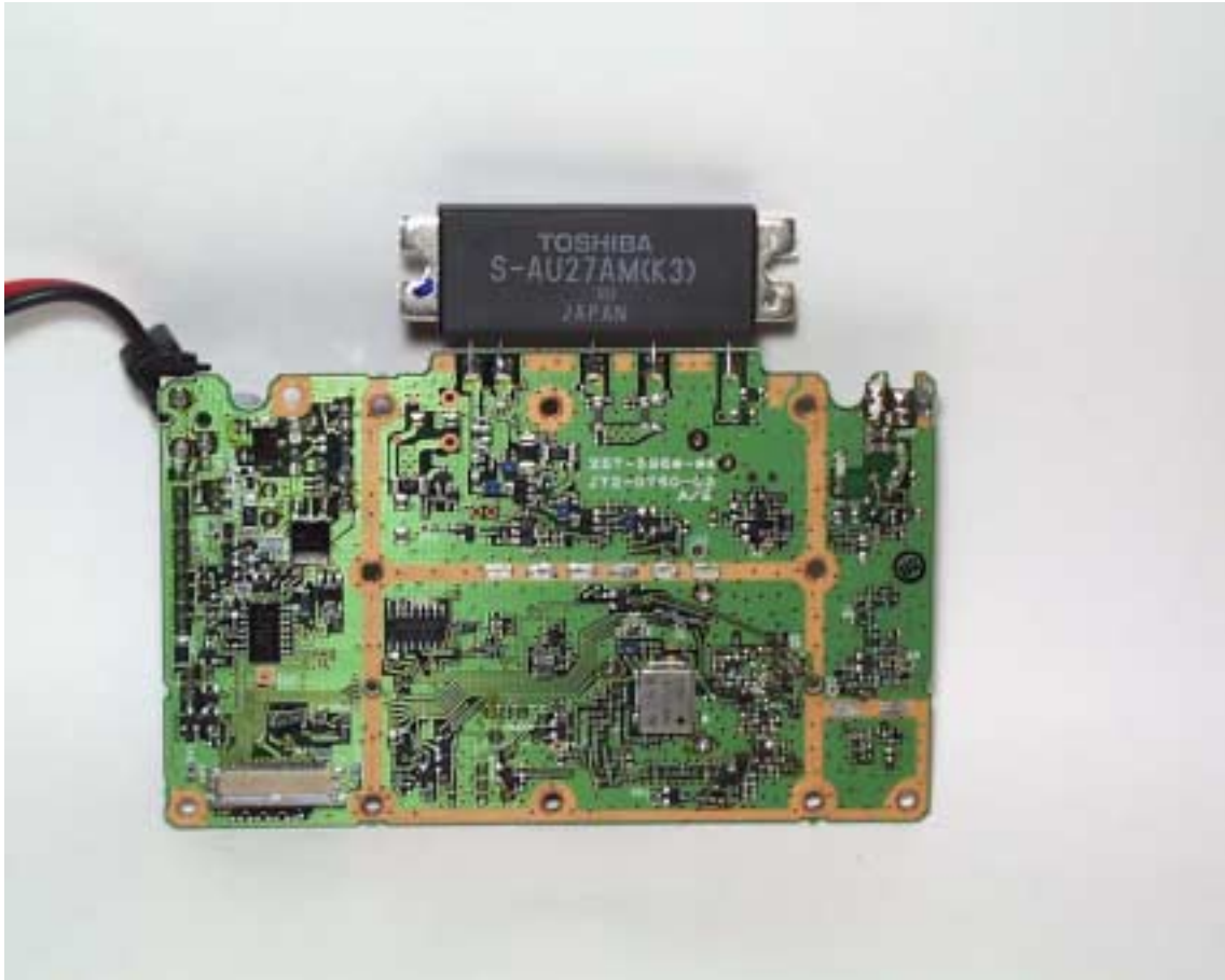
PC BOARD (TX/RX UNIT BOTTOM VIEW) MODEL NAME:TK-860HGK FCC ID:ALH29383210
