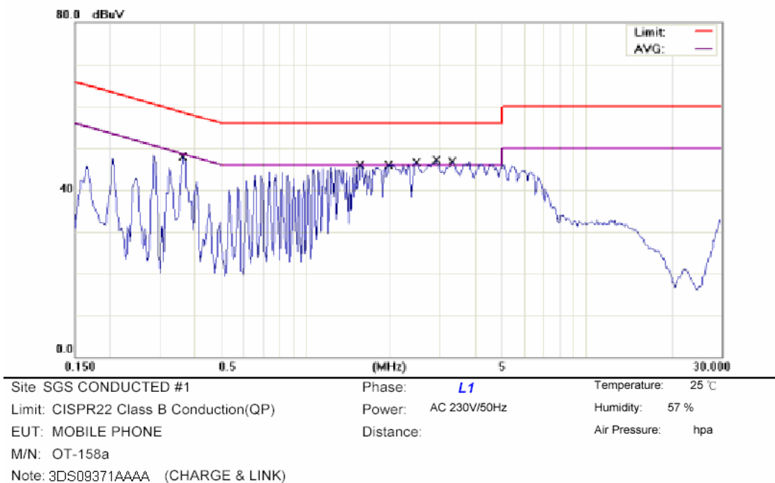
Conducted Emission Measurement
