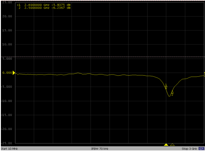
Return loss
