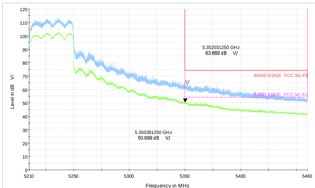
Wi-Fi 5G_ax40 CH46_5.21-5.46GHz_MCS0_MIMO_V_TP24
