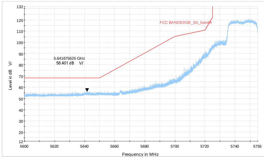
Wi-Fi 5G_ax20 CH149_5.6-5.755GHz_MCS0_MIMO_V_TP24
