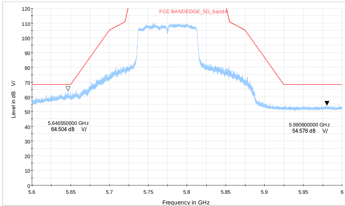
Wi-Fi 5G_ac80 CH155_5.6-6GHz_MCS0_MIMO_V_TP21
