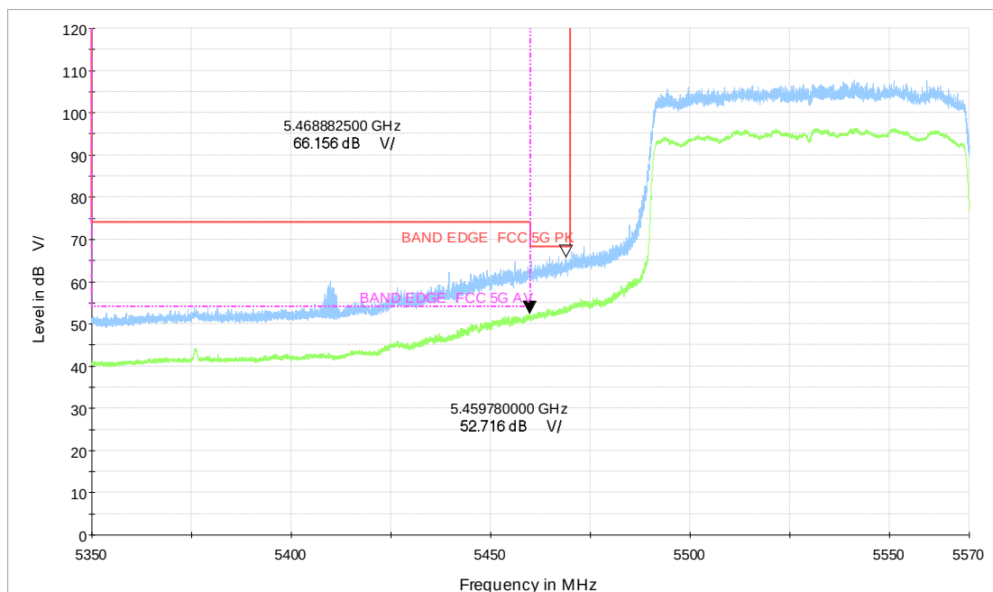
Wi-Fi 5G_ax80 CH106_5.35-5.57GHz_MCS0_MIMO_V_TP15
