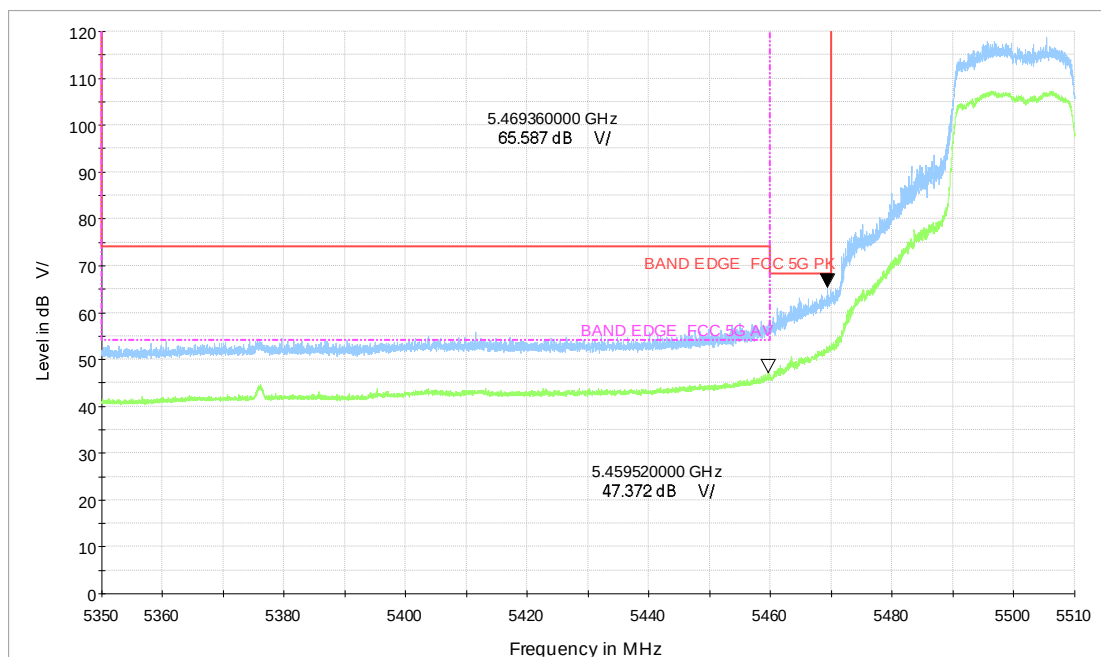
Wi-Fi 5G_ax20 CH100_5.35-5.51GHz_MCS0_MIMO_V_TP22
