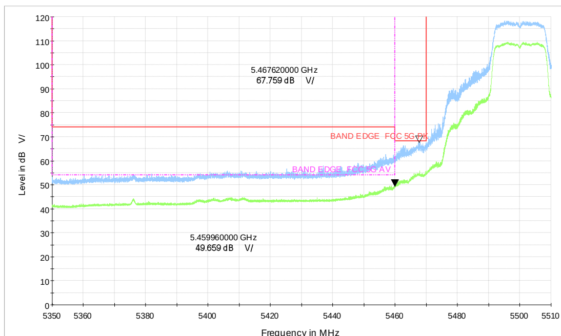
Wi-Fi 5G_a CH100_5.35-5.51GHz_6M_MIMO_V_TP23
