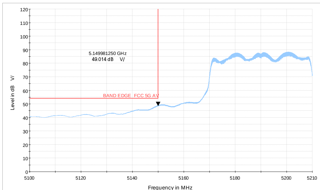
Wi-Fi 5G_ax40 CH38_5.1-5.21GHz_MCS0_MIMO_V_TP21_AV
