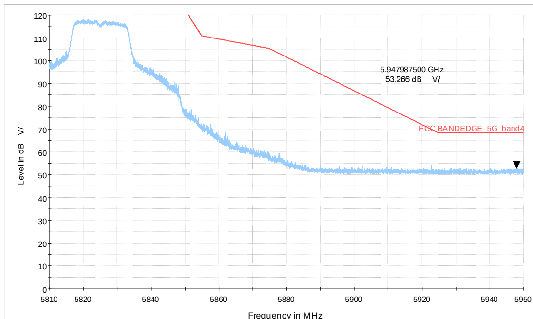
Wi-Fi 5G_a CH165_5.81-5.95GHz_6M_MIMO_V_TP24
