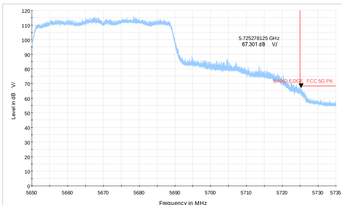
Wi-Fi 5G_ax40 CH134_5.65-5.735GHz_MCS0_MIMO_V_TP20
