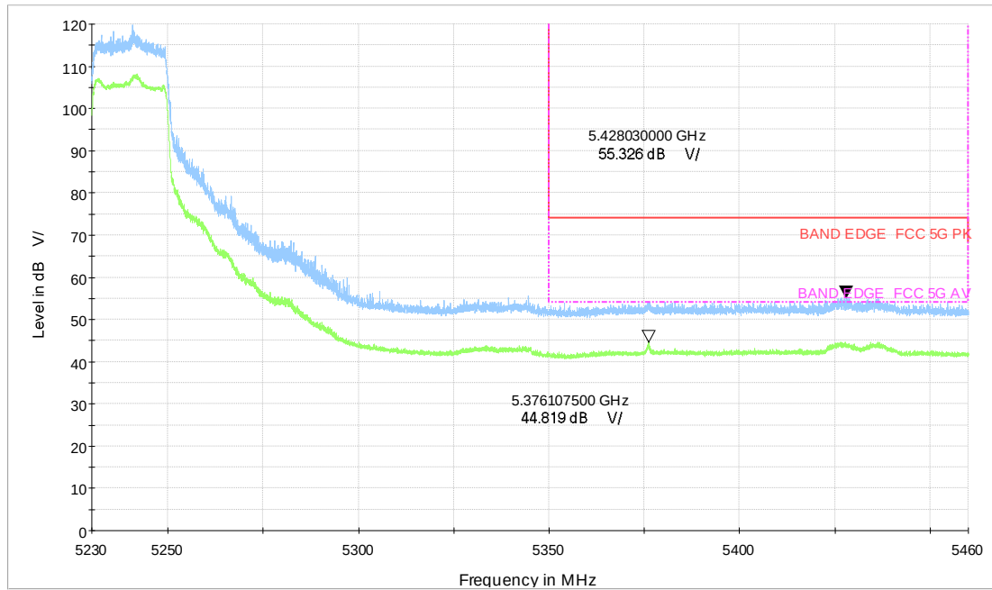
Wi-Fi 5G_ax20 CH48_5.23-5.46GHz_MCS0_MIMO_V_TP24
