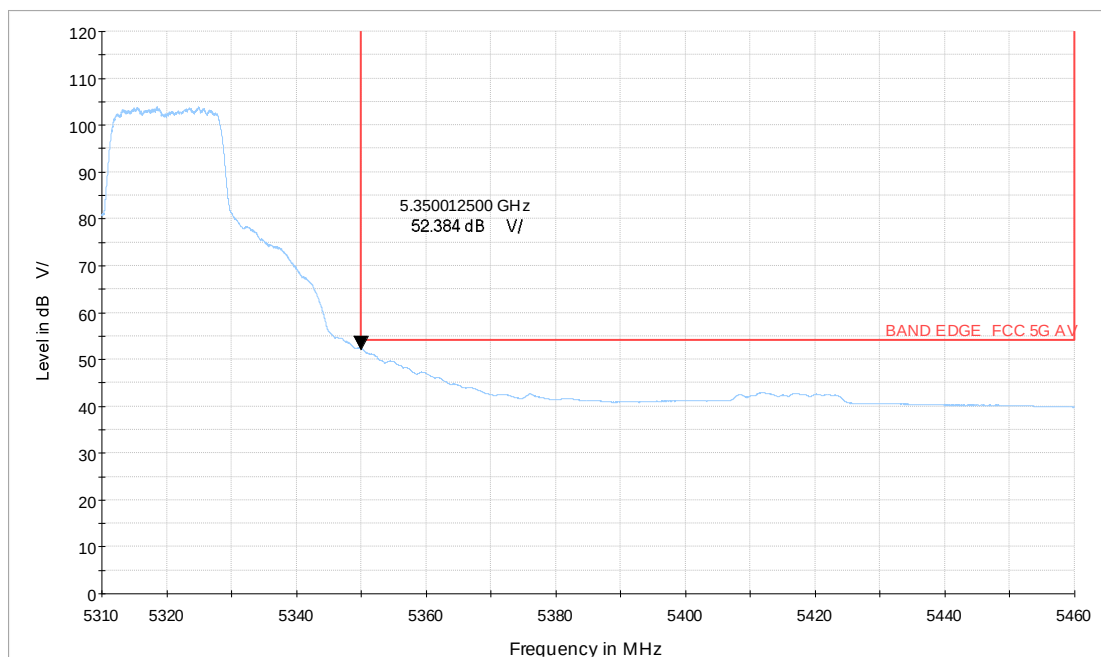
Wi-Fi 5G_a CH64_5.31-5.46GHz_6M_MIMO_V_TP23_AV
