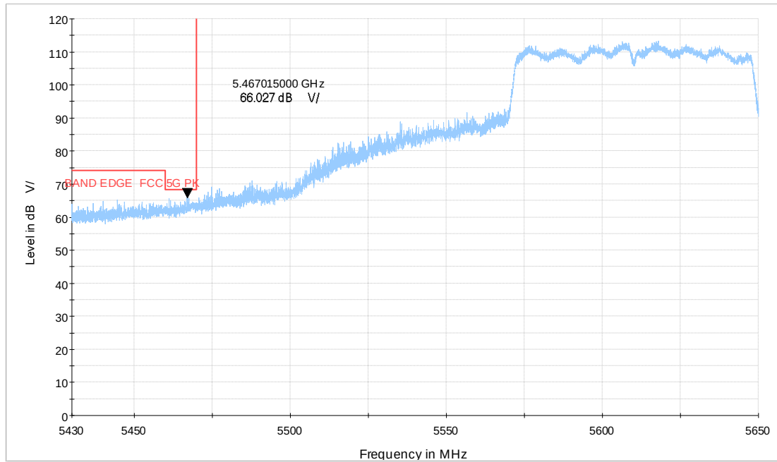
Wi-Fi 5G_ac80 CH122_5.43-5.65GHz_MCS0_MIMO_V_TP23
