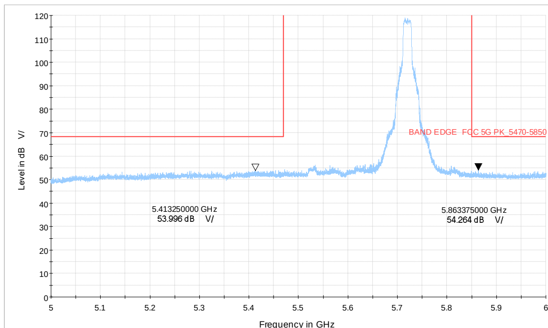
Wi-Fi 5G_a CH144_5-6GHz_6M_MIMO_V_TP24
