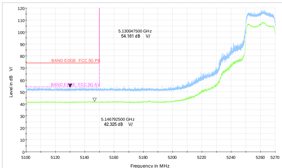
Wi-Fi 5G_ax20 CH52_5.1-5.27GHz_MCS0_MIMO_V_TP24
