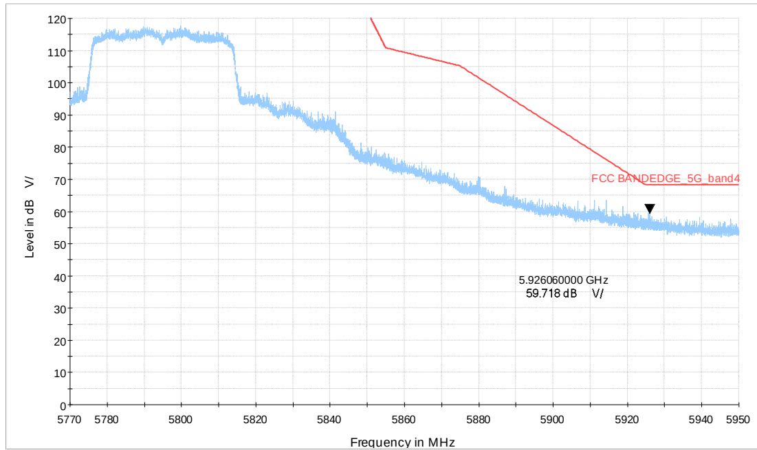
Wi-Fi 5G_ax40 CH159_5.77-5.95GHz_MCS0_MIMO_V_TP24
