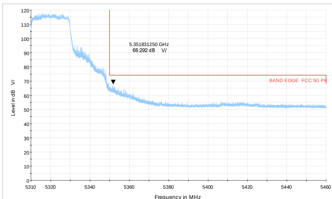
Wi-Fi 5G_ax20 CH64_5.31-5.46GHz_MCS0_MIMO_V_TP24_PK
