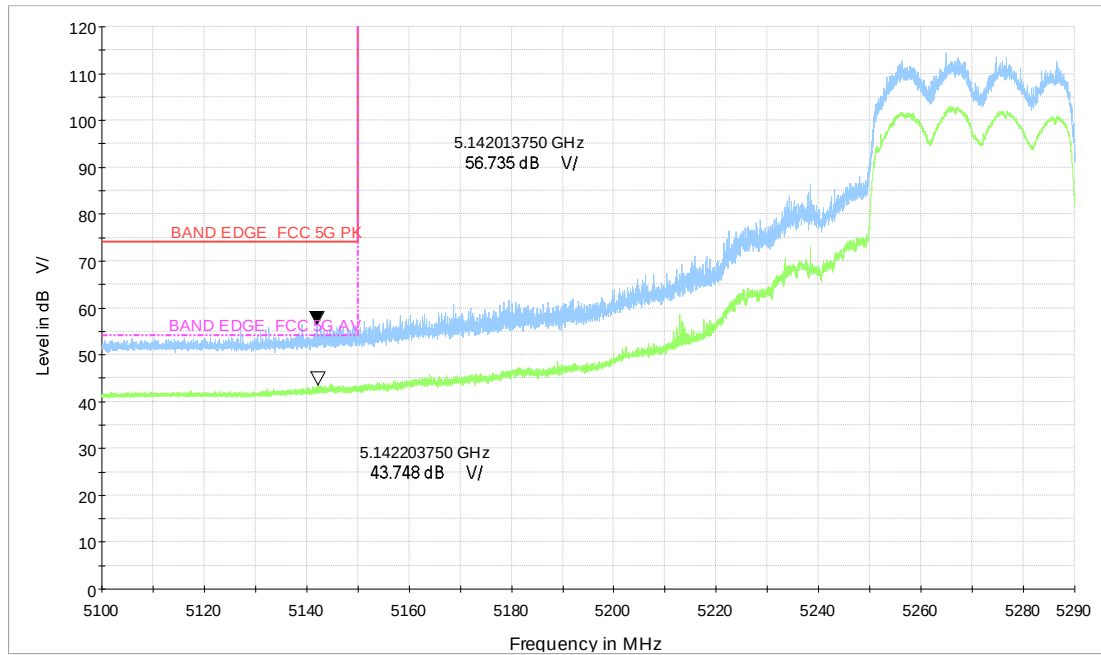
Wi-Fi 5G_ax40 CH54_5.1-5.29GHz_MCS0_MIMO_V_TP24
