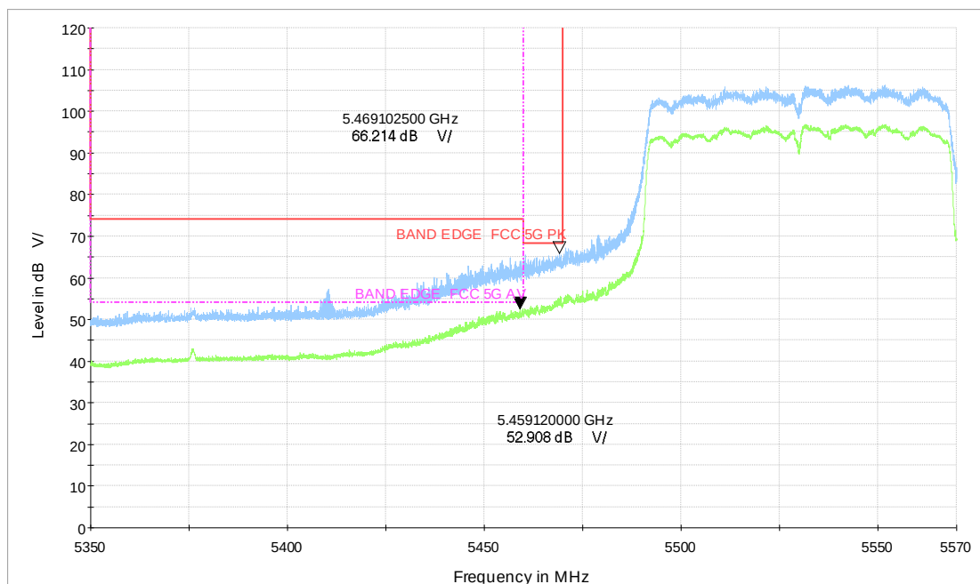
Wi-Fi 5G_ac80 CH106_5.35-5.57GHz_MCS0_MIMO_V_TP15
