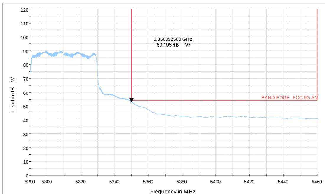
Wi-Fi 5G_ax40 CH62_5.29-5.46GHz_MCS0_MIMO_V_TP22_AV
