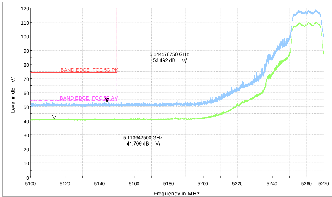
Wi-Fi 5G_a CH52_5.1-5.27GHz_6M_MIMO_V_TP24
