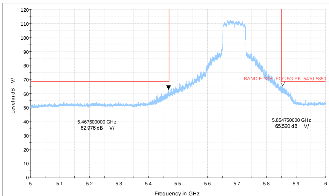
Wi-Fi 5G_ac80 CH138_5-6GHz_MCS0_MIMO_V_TP24
