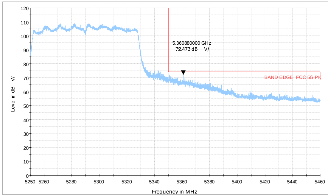
Wi-Fi 5G_ac80 CH58_5.25-5.46GHz_MCS0_MIMO_V_TP19_PK
