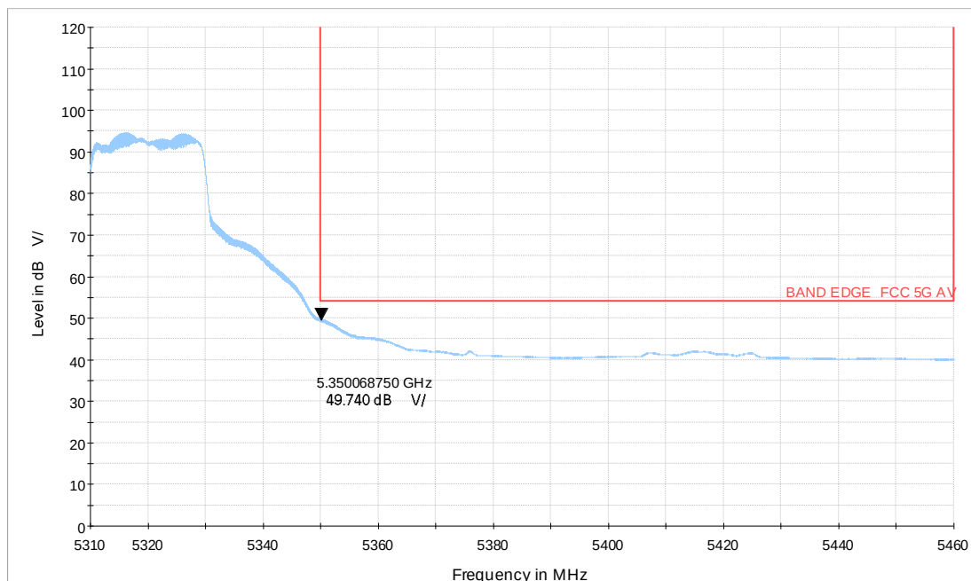
Wi-Fi 5G_ax20 CH64_5.31-5.46GHz_MCS0_MIMO_V_TP24_AV
