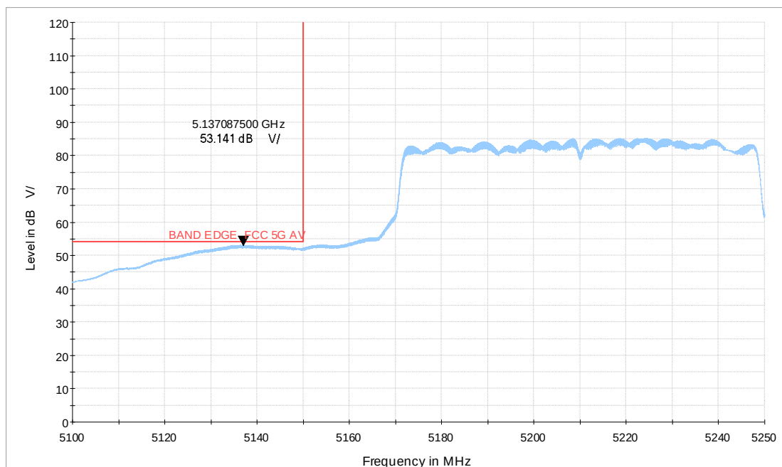
Wi-Fi 5G_ac80 CH42_5.1-5.25GHz_MCS0_MIMO_V_TP19_AV
