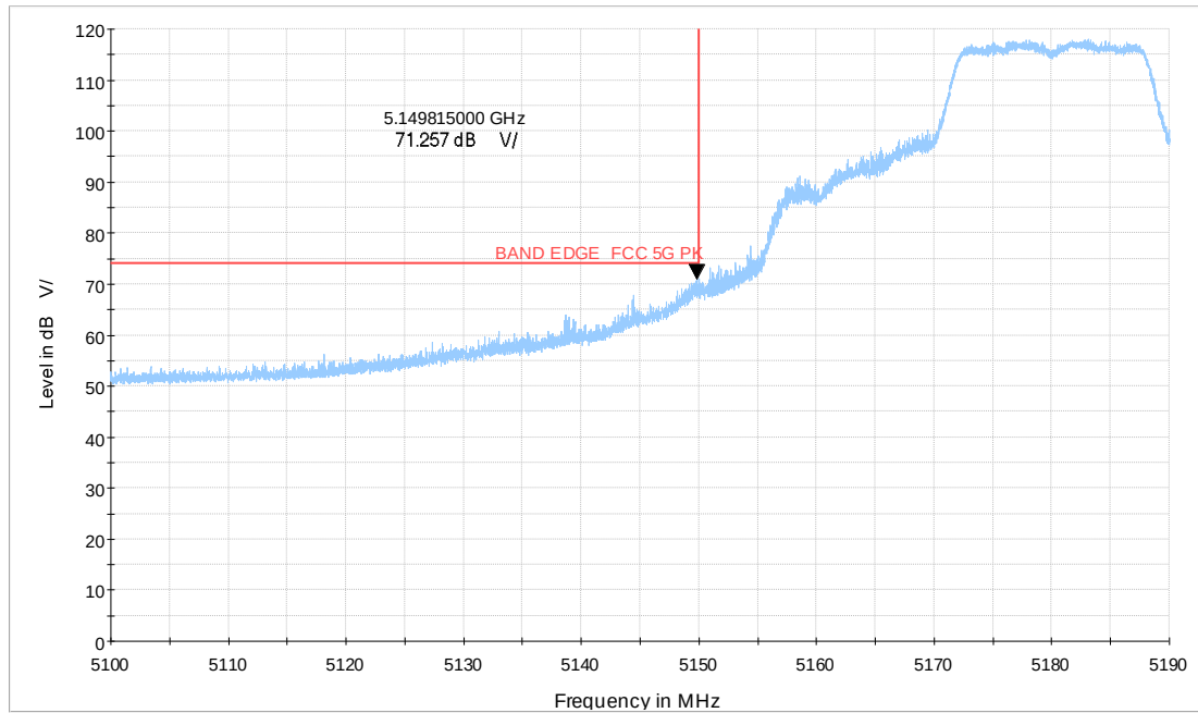
Wi-Fi 5G_a CH36_5.1-5.19GHz_6M_MIMO_V_TP23_PK
