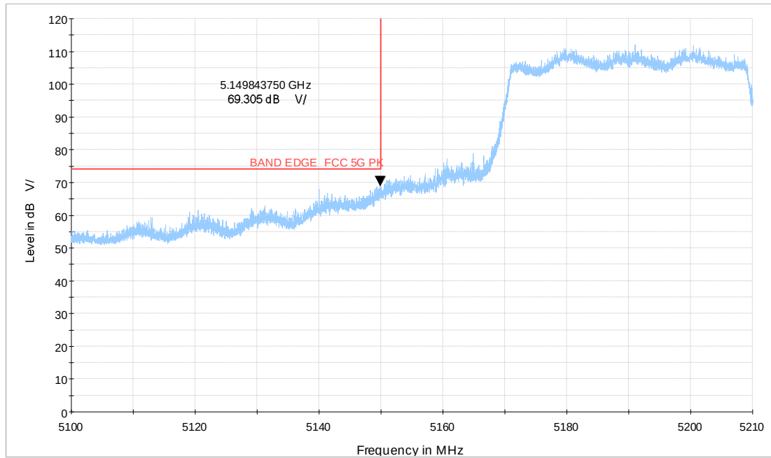
Wi-Fi 5G_ax40 CH38_5.1-5.21GHz_MCS0_MIMO_V_TP21_PK
