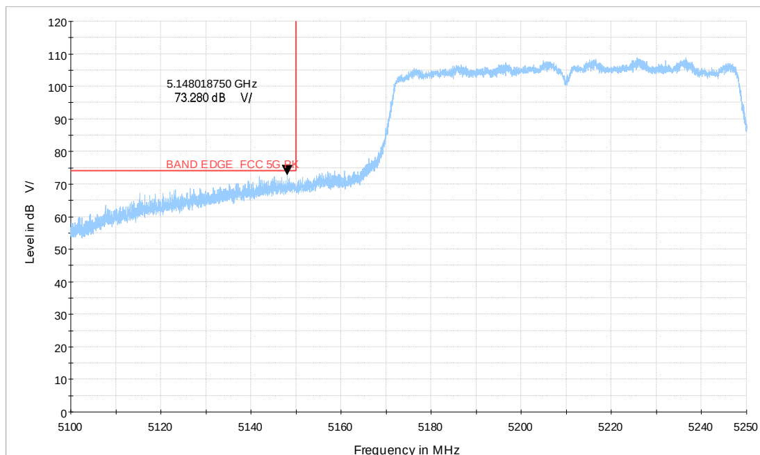
Wi-Fi 5G_ac80 CH42_5.1-5.25GHz_MCS0_MIMO_V_TP19_PK
