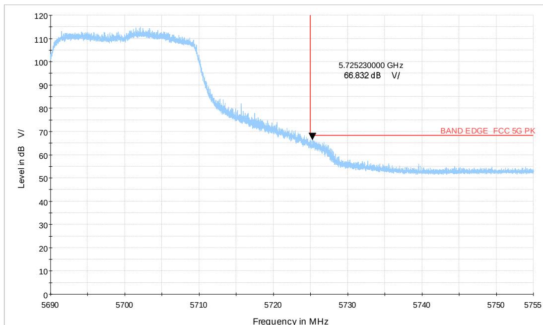
Wi-Fi 5G_ax20 CH140_5.69-5.755GHz_MCS0_MIMO_V_TP17
