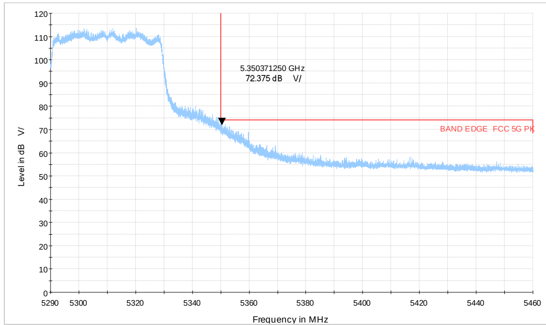
Wi-Fi 5G_ax40 CH62_5.29-5.46GHz_MCS0_MIMO_V_TP22_PK
