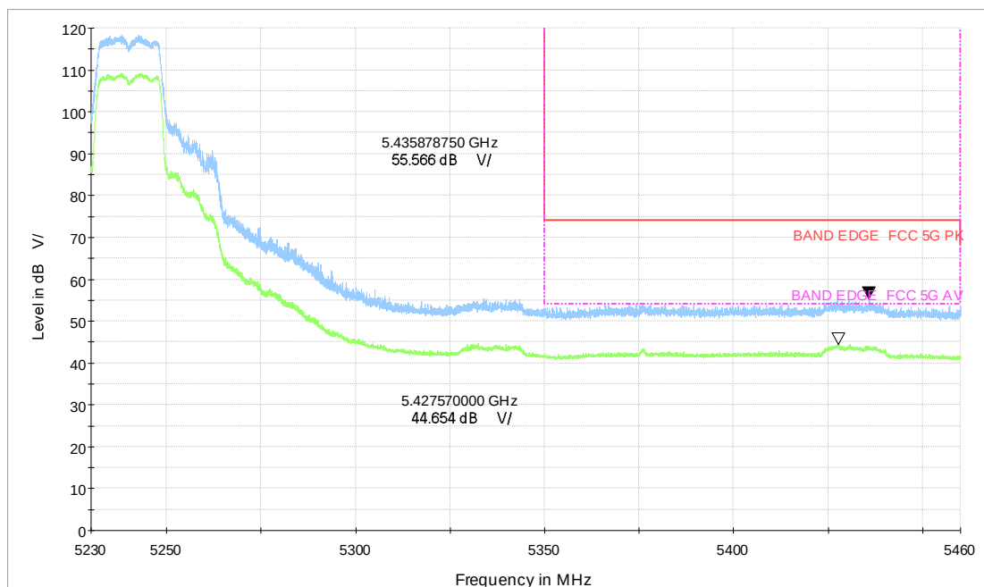
Wi-Fi 5G_a CH48_5.23-5.46GHz_6M_MIMO_V_TP24
