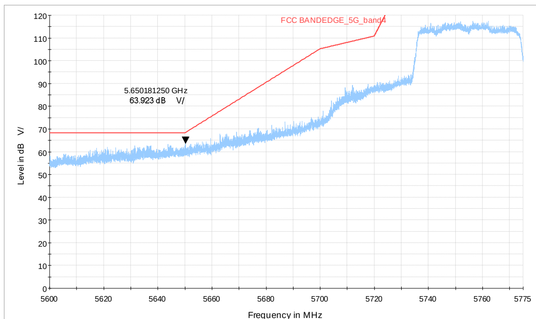
Wi-Fi 5G_ax40 CH151_5.6-5.775GHz_MCS0_MIMO_V_TP23
