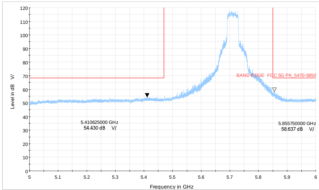
Wi-Fi 5G_ax40 CH142_5-6GHz_MCS0_MIMO_V_TP24
