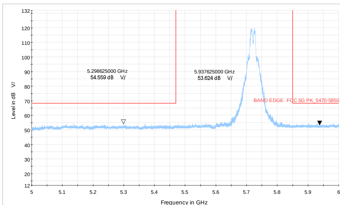
Wi-Fi 5G_ax20 CH144_5-6GHz_MCS0_MIMO_V_TP24
