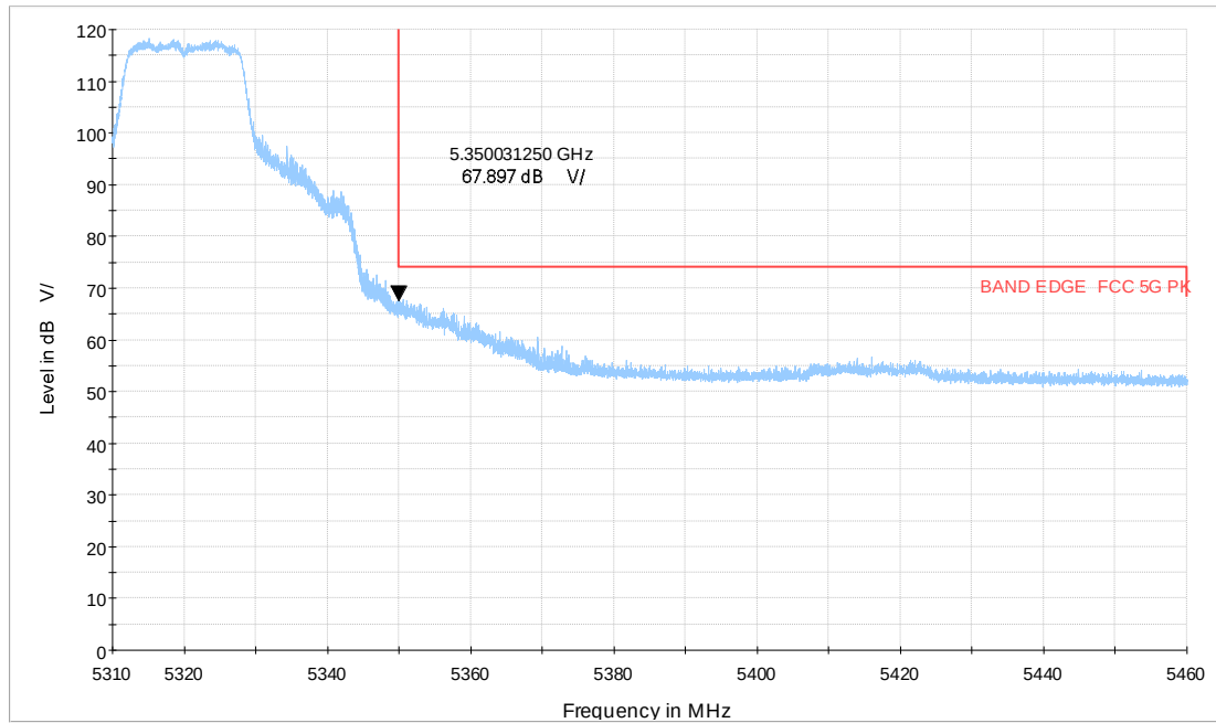
Wi-Fi 5G_a CH64_5.31-5.46GHz_6M_MIMO_V_TP23_PK
