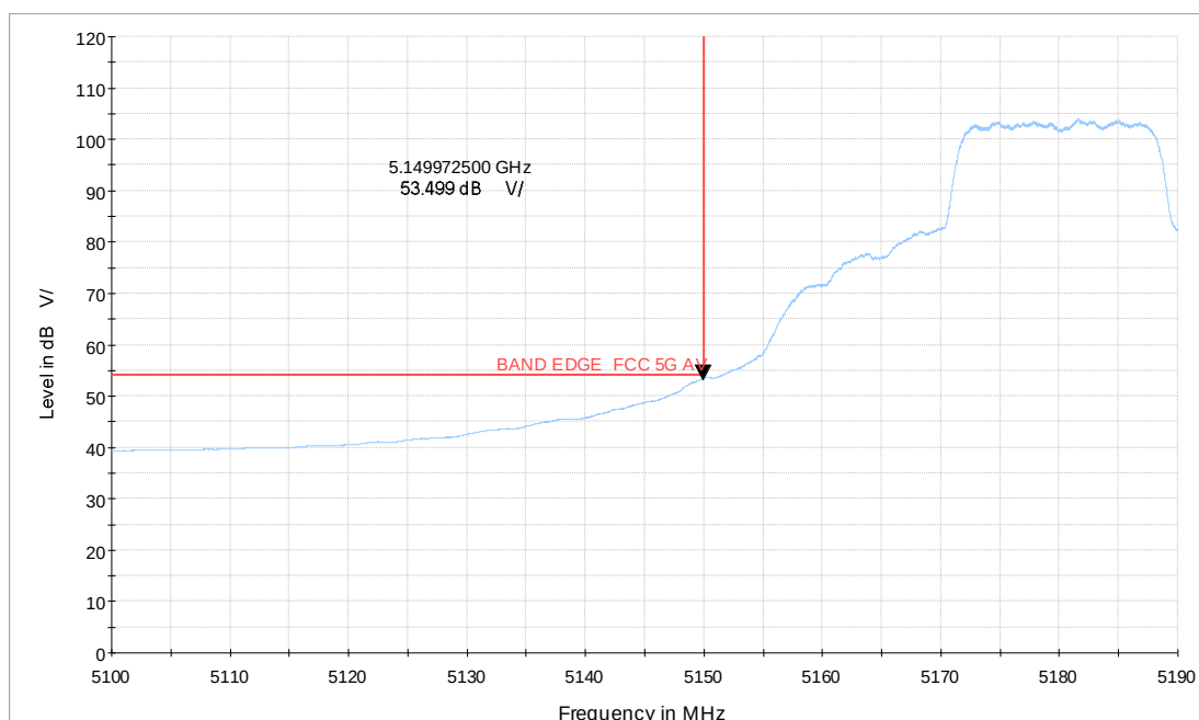
Wi-Fi 5G_a CH36_5.1-5.19GHz_6M_MIMO_V_TP23_AV
