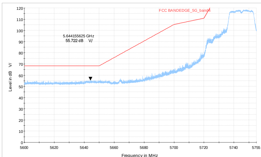
Wi-Fi 5G_a CH149_5.6-5.755GHz_6M_MIMO_V_TP24
