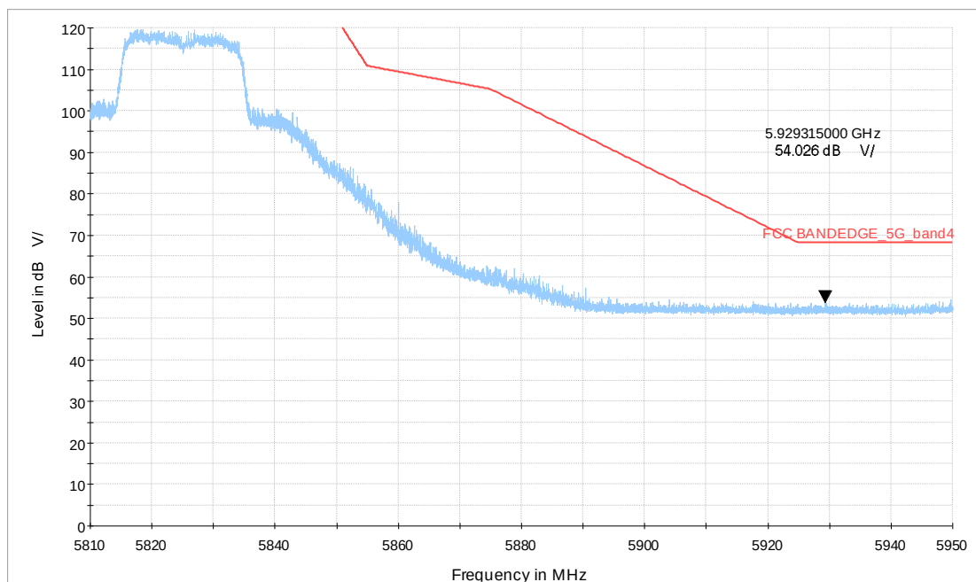
Wi-Fi 5G_ax20 CH165_5.81-5.95GHz_MCS0_MIMO_V_TP24
