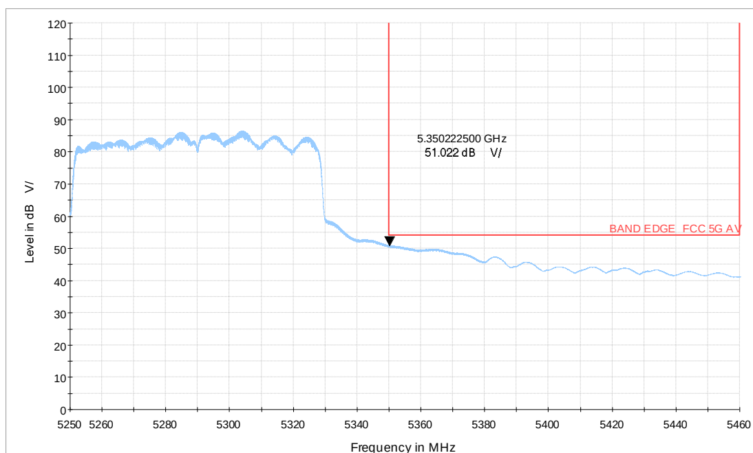
Wi-Fi 5G_ac80 CH58_5.25-5.46GHz_MCS0_MIMO_V_TP19_AV
