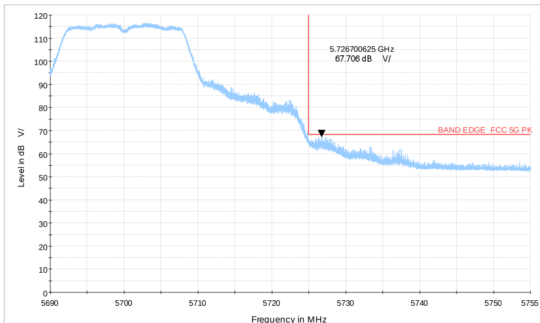
Wi-Fi 5G_a CH140_5.69-5.755GHz_6M_MIMO_V_TP20
