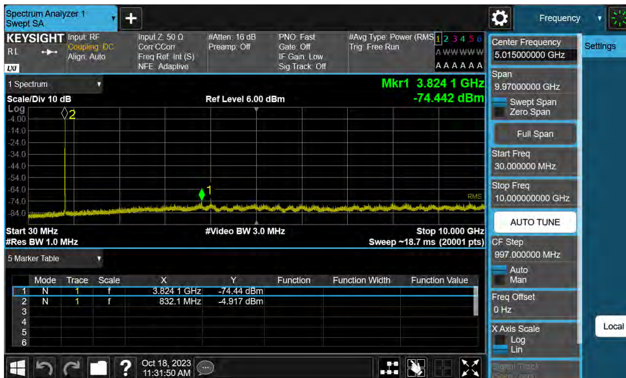
Sub6 n5. Conducted Spurious Plot (167300ch_10 MHz_BPSK_RB 1_1)
