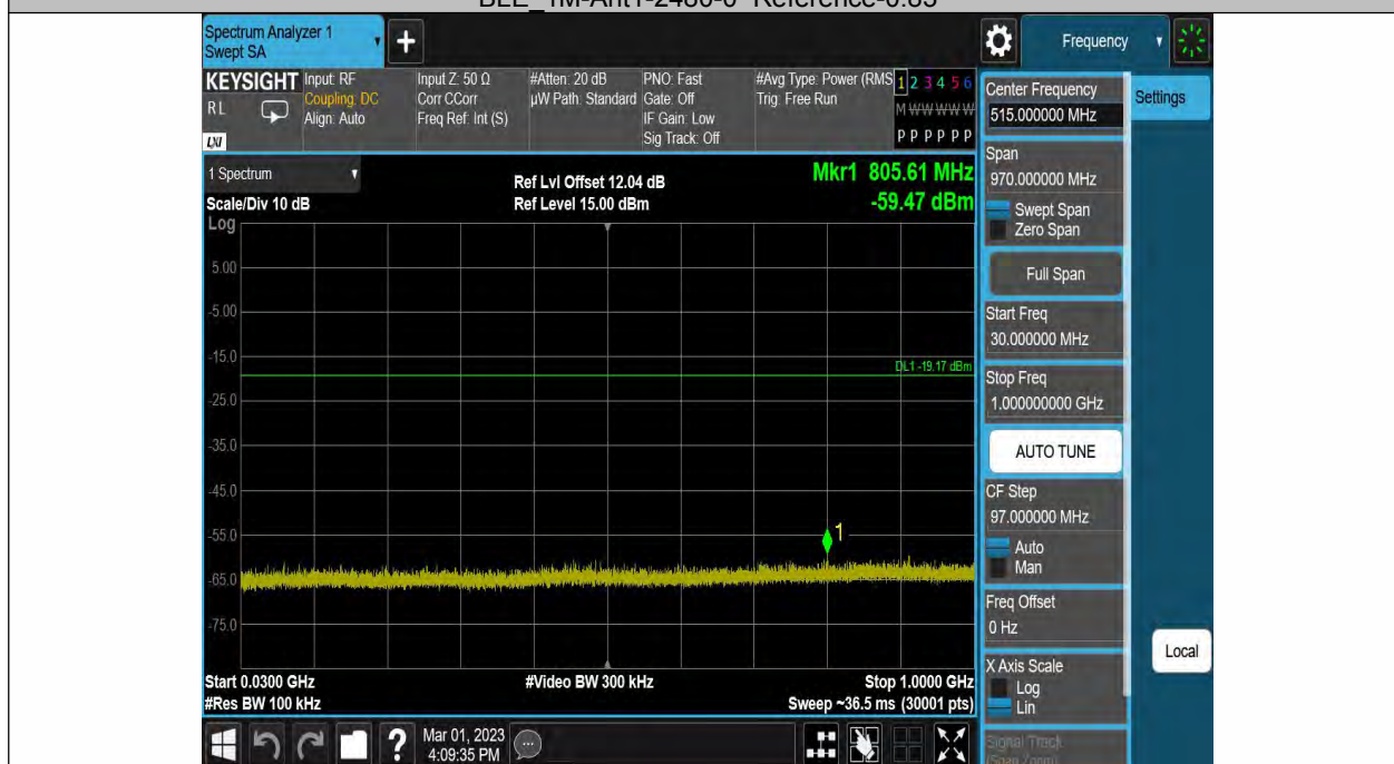
BLE_1M-Ant1-2480-30~1000-0.83
