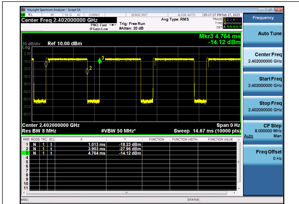
EDR--8DPSK-ANT1-2402
