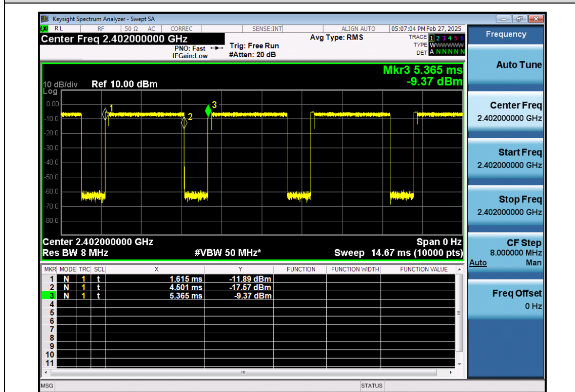
EDR-π /4-DQPSK-ANT1-2402
