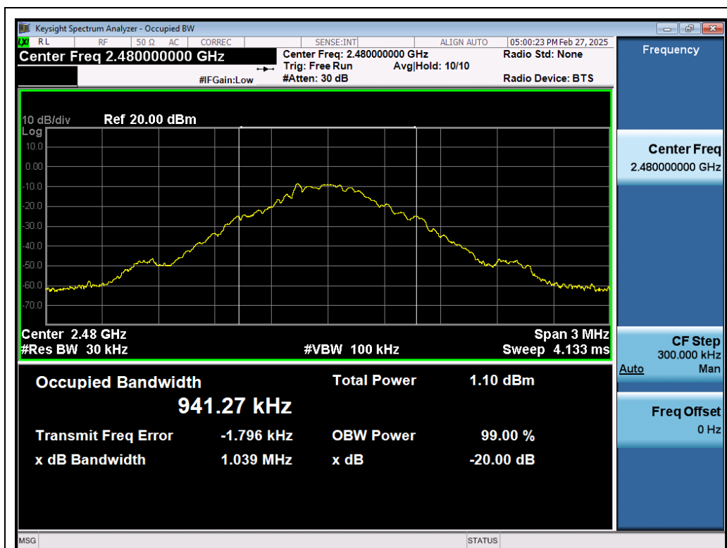
Test_Graph_BR_ANT1_2480_1Mbps_OBW
