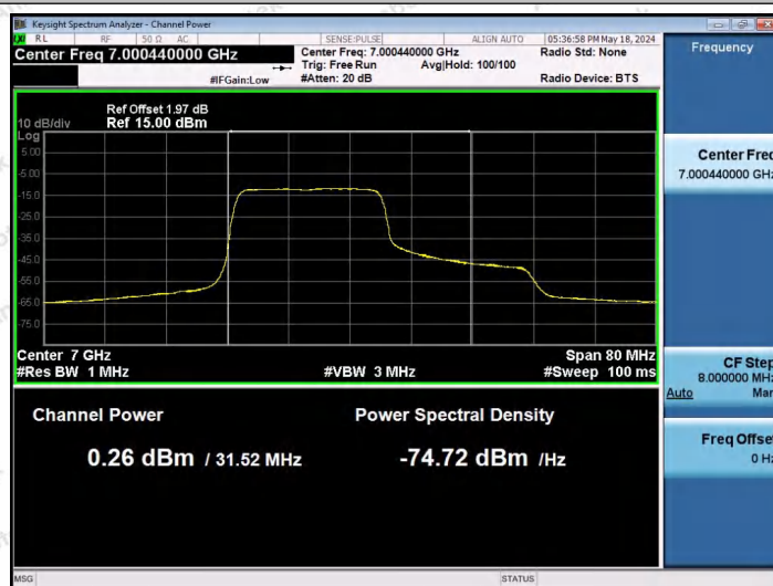
11AX40SISO-Ant1-7005-242Tone-RU61-PASS
