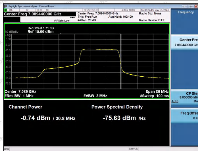
11AX40SISO-Ant1-7085-242Tone-RU62-PASS
