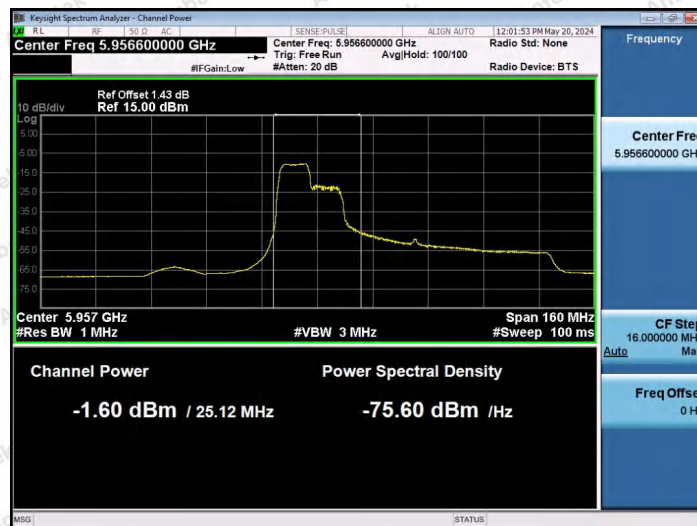
11AX80SISO-Ant1-5985-106Tone-RU53-PASS
