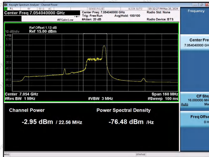
11AX80SISO-Ant1-7025-26Tone-RU36-PASS
