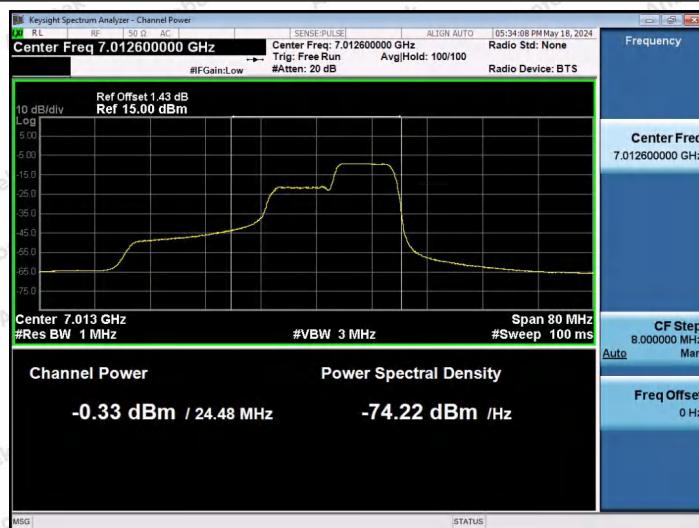
11AX40SISO-Ant1-7005-106Tone-RU56-PASS
