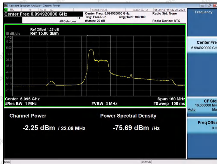
11AX80SISO-Ant1-7025-52Tone-RU37-PASS
