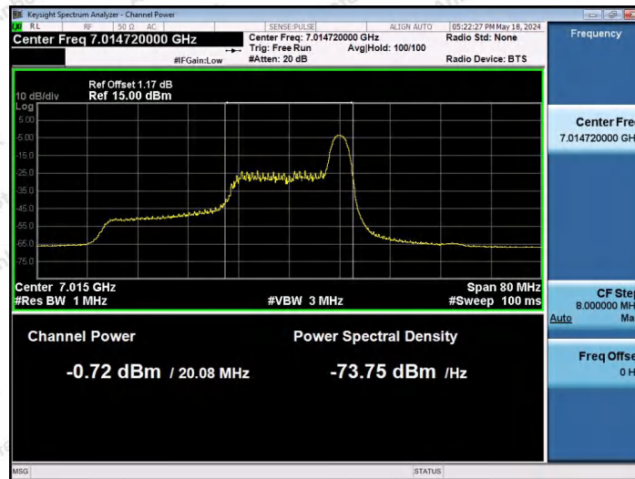
11AX40SISO-Ant1-7005-26Tone-RU17-PASS
