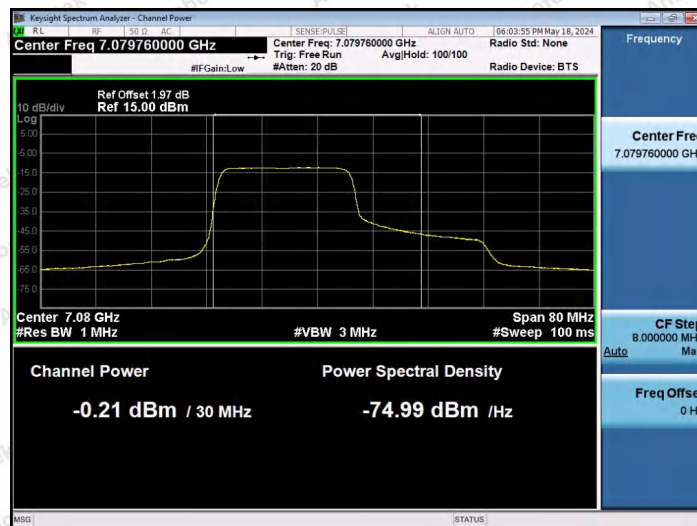
11AX40SISO-Ant1-7085-242Tone-RU61-PASS
