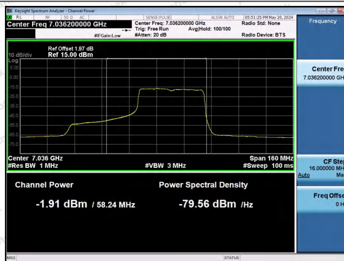
11AX80SISO-Ant1-7025-484Tone-RU66-PASS
