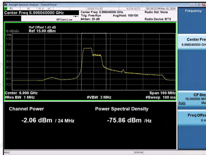
11AX80SISO-Ant1-7025-106Tone-RU53-PASS
