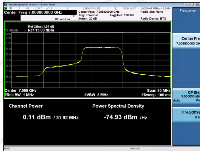
11AX40SISO-Ant1-7005-242Tone-RU62-PASS
