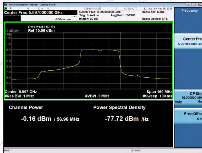
11AX80SISO-Ant1-5985-484Tone-RU66-PASS
