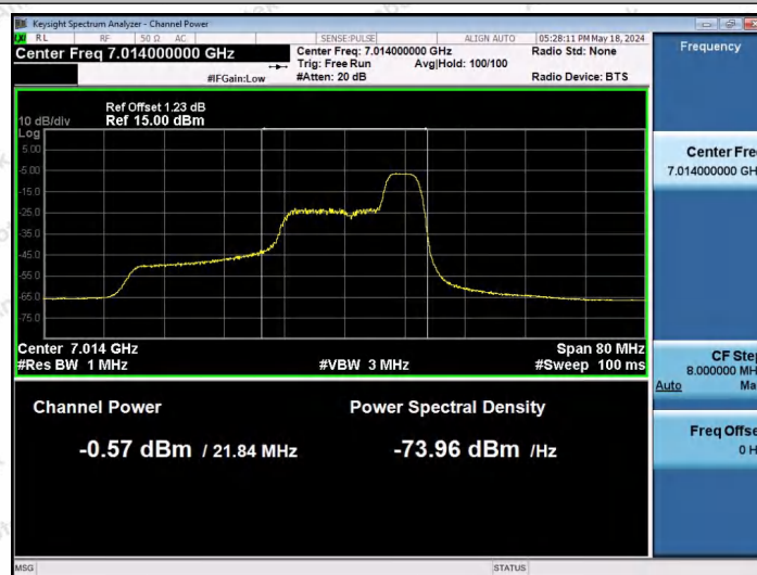
11AX40SISO-Ant1-7005-52Tone-RU44-PASS
