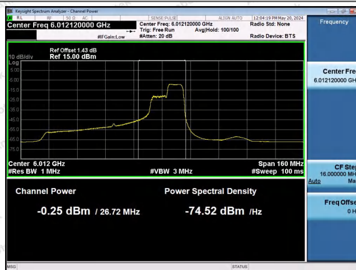
11AX80SISO-Ant1-5985-106Tone-RU60-PASS
