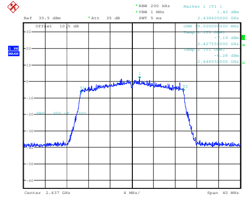
802.11ax20_2437MHz_RU_Full_Chain 0
