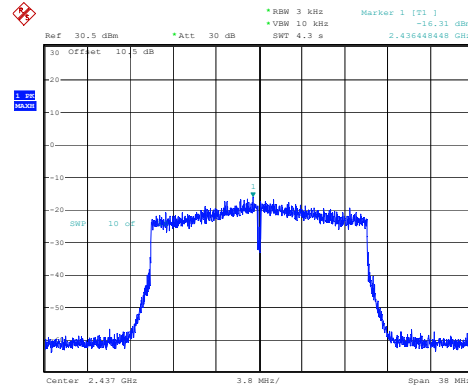
802.11ax20_2437MHz_RU_Full_Chain 0
