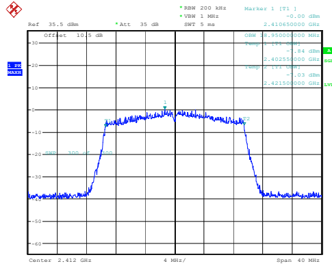
802.11ax20_2412MHz_RU_Full_Chain 0
