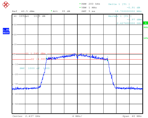
802.11ax20_2437MHz_RU_Full_Chain 1
