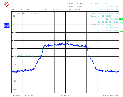
802.11g_2412MHz_Chain 1
