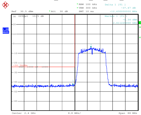
802.11ax20_2412MHz_RU_Full_Chain 0
