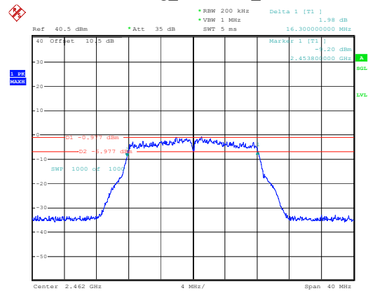
802.11g_2462MHz_Chain 1
