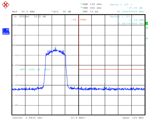
802.11ax20_2462MHz_RU_Full_Chain 1
