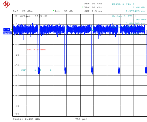
802.11g_2437MHz_Chain 0
