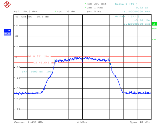
802.11g_2437MHz_Chain 0
