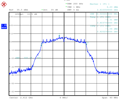
802.11g_2412MHz
