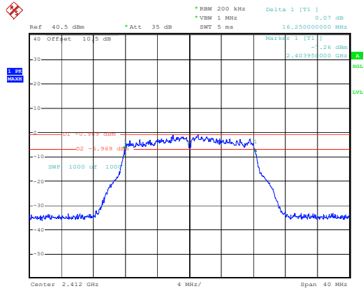
802.11g_2412MHz_Chain 0
