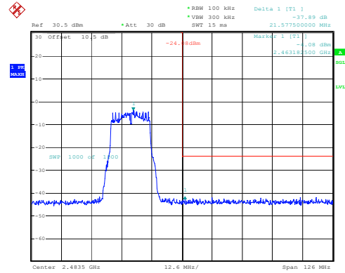
802.11g_2462MHz_Chain 0
