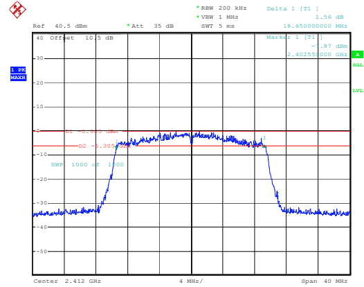
802.11ax20_2412MHz_RU_Full_Chain 1
