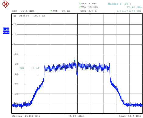
802.11g_2412MHz_Chain 0
