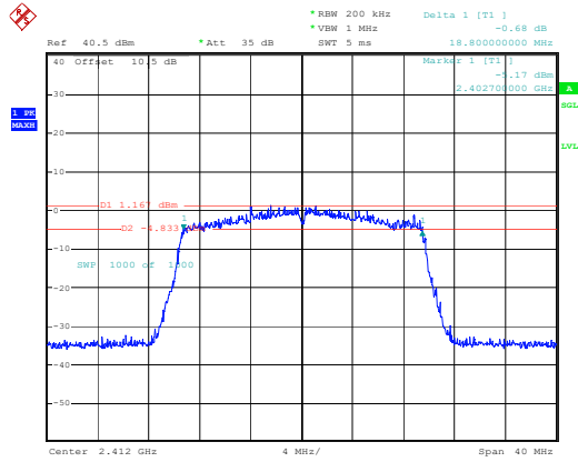
802.11ax20_2412MHz_RU_Full_Chain 0
