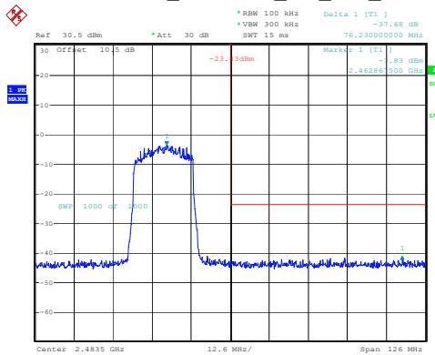
802.11ax20_2462MHz_RU_Full_Chain 0
