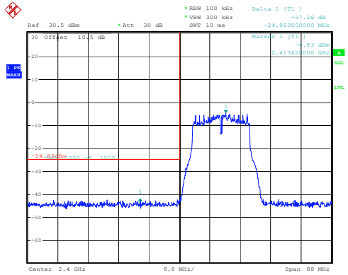
802.11g_2412MHz_Chain 0
