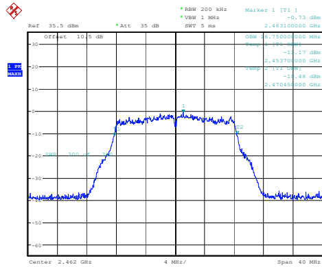
802.11g_2462MHz_Chain 0
