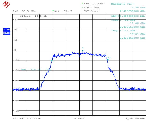
802.11g_2412MHz_Chain 0
