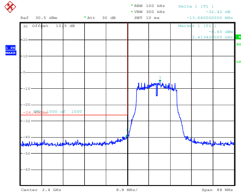
802.11g_2412MHz_Chain 1
