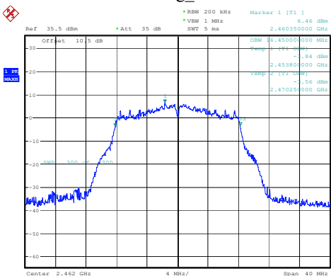
802.11g_2462MHz
