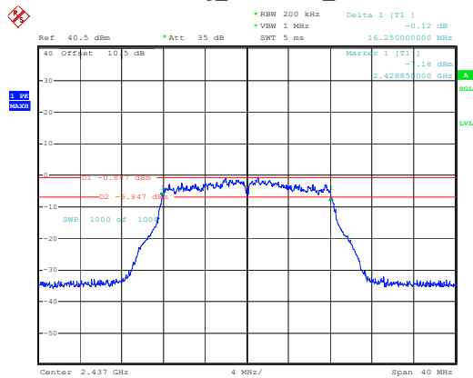
802.11g_2437MHz_Chain 1
