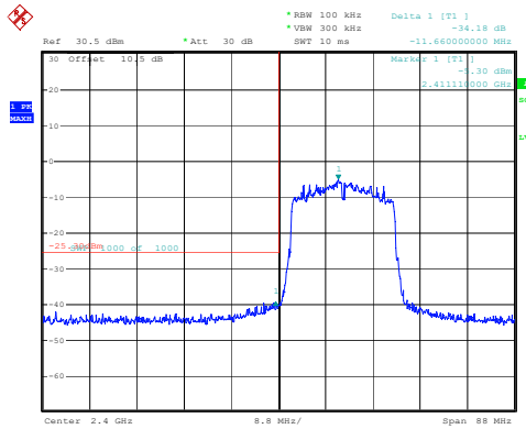
802.11ax20_2412MHz_RU_Full_Chain 1
