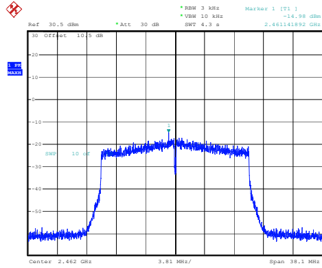
802.11ax20_2462MHz_RU_Full_Chain 0
