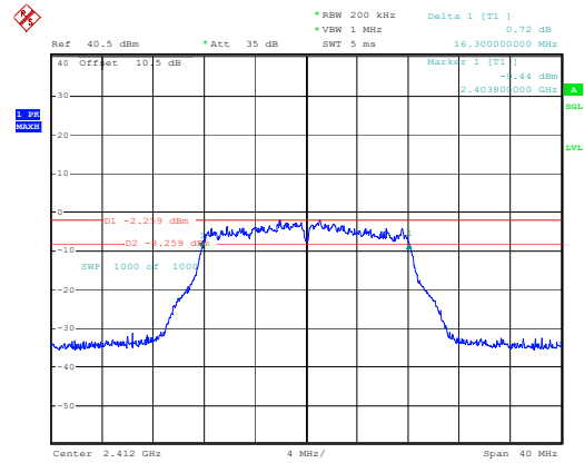
802.11g_2412MHz_Chain 1
