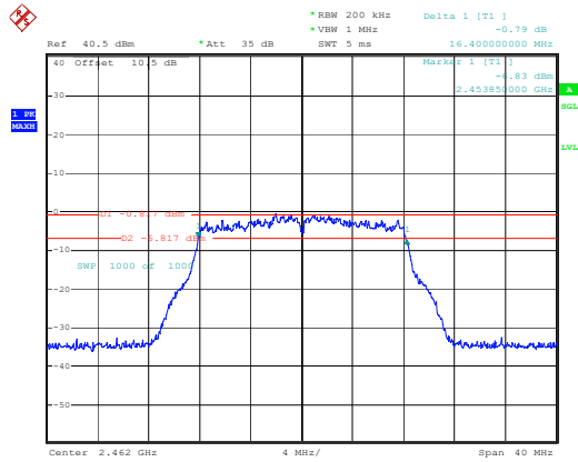
802.11g_2462MHz_Chain 0
