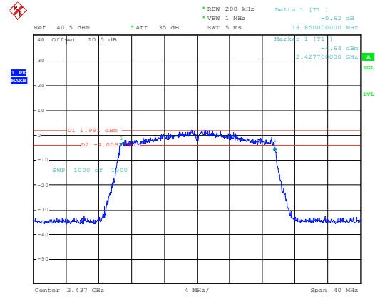
802.11ax20_2437MHz_RU_Full_Chain 0
