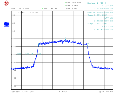
802.11ax20_2412MHz_RU_Full_Chain 1
