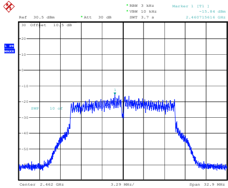
802.11g_2462MHz_Chain 0
