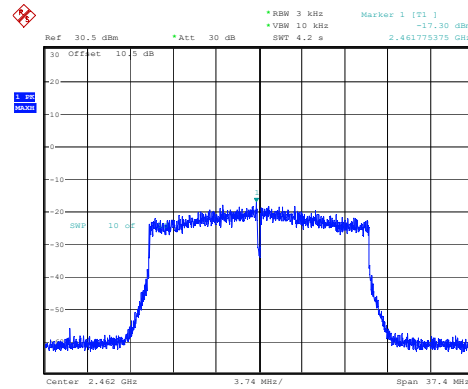
802.11ax20_2462MHz_RU_Full_Chain 1
