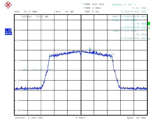
802.11ax20_2462MHz_RU_Full_Chain 1
