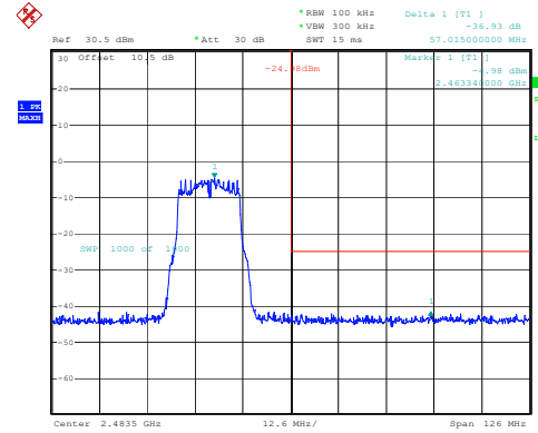
802.11g_2462MHz_Chain 1
