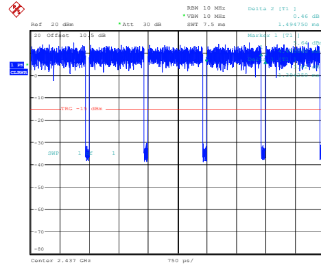
802.11g_2437MHz_Chain 1
