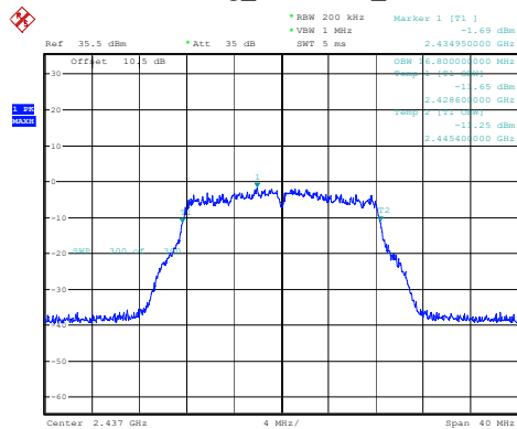
802.11g_2437MHz_Chain 1
