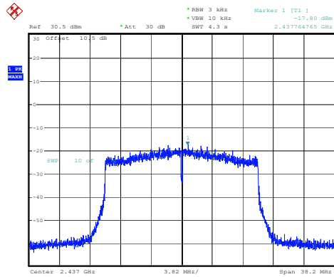
802.11ax20_2437MHz_RU_Full_Chain 1
