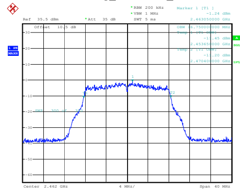
802.11g_2462MHz_Chain 1
