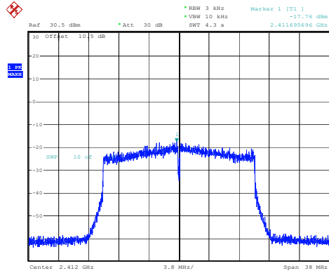
802.11ax20_2412MHz_RU_Full_Chain 0
