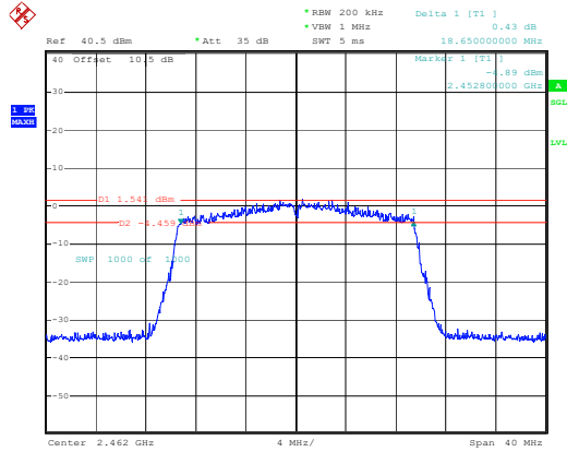
802.11ax20_2462MHz_RU_Full_Chain 0
