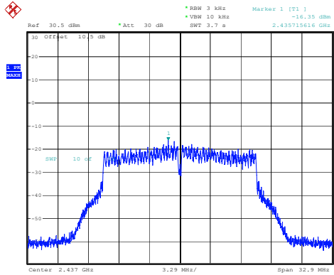
802.11g_2437MHz_Chain 1
