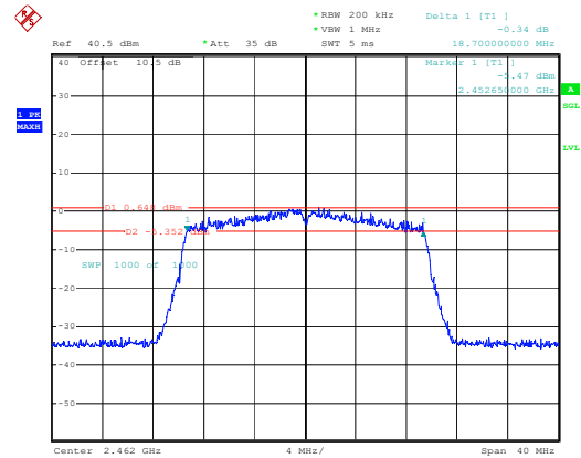
802.11ax20_2462MHz_RU_Full_Chain 1
