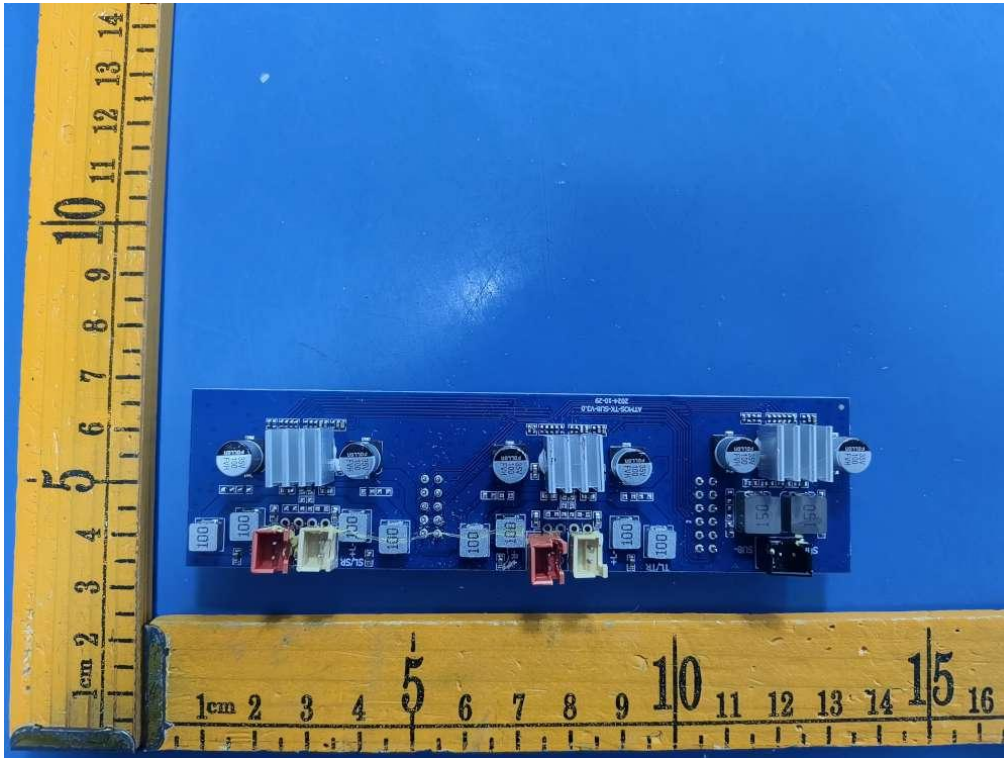
Internal view of unit (Model:A502PRO, A502)
