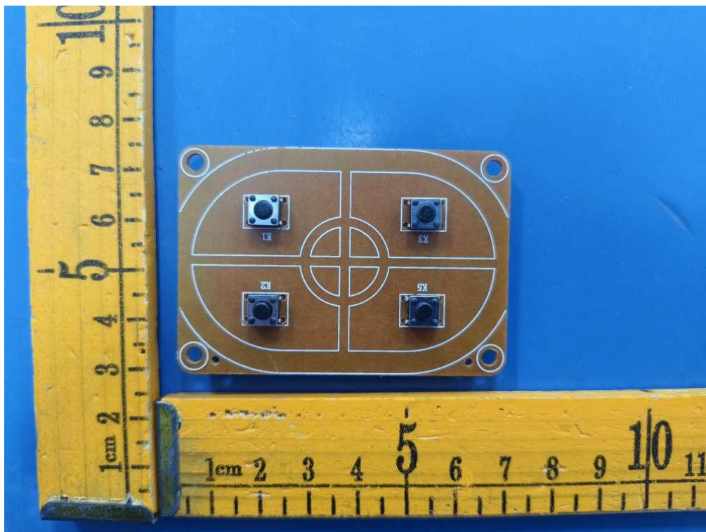
Internal view of unit (Model:A41, A21)
