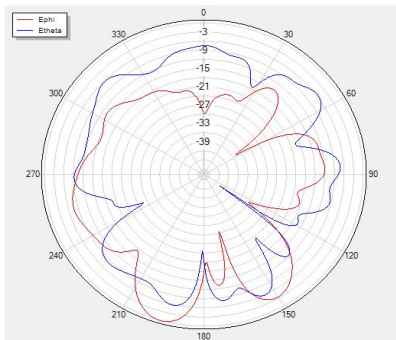
Phi=90 freq=2400MHz
