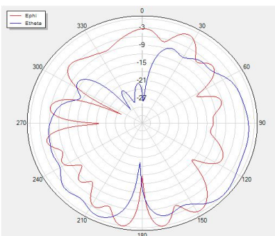
Phi=0 freq=2400MHz
