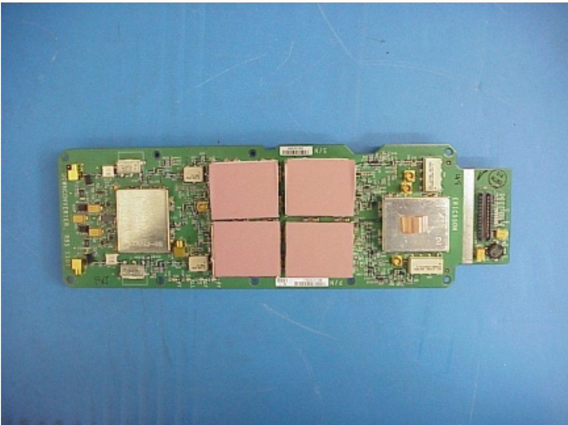
Downconverter Board
