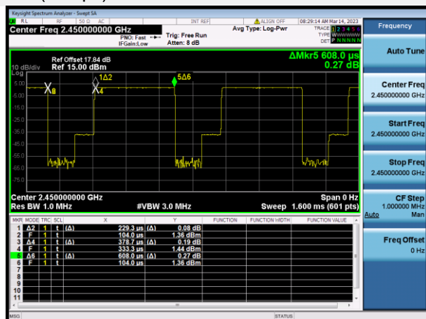
FSK(1Mbps)
