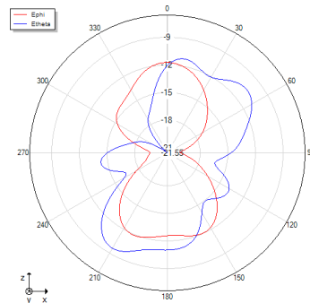
Phi=0 freq=1176.44995117188MHz
