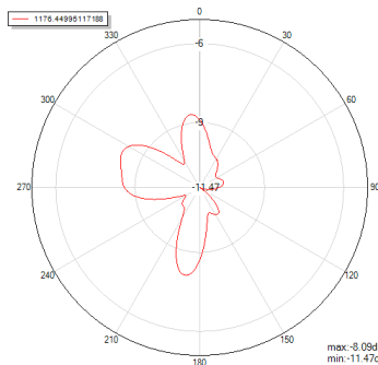
Phi=90 freq=1176.44995117188MHz
