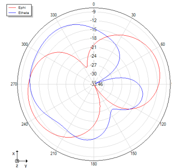
Theta=90 freq=1176.44995117188MHz
