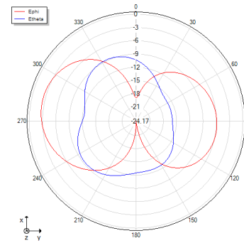
Theta=90 freq=1575.42004394531MHz
