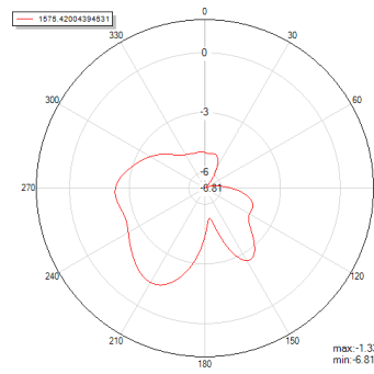
Phi=90 freq=1575.42004394531MHz
