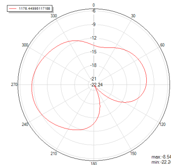
Theta=90 freq=1176.44995117188MHz
