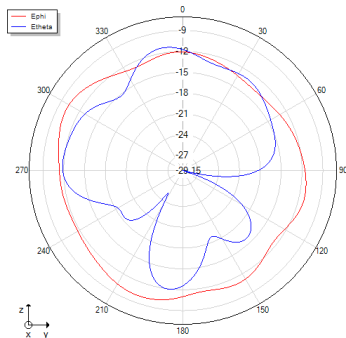
Phi=90 freq=1176.44995117188MHz
