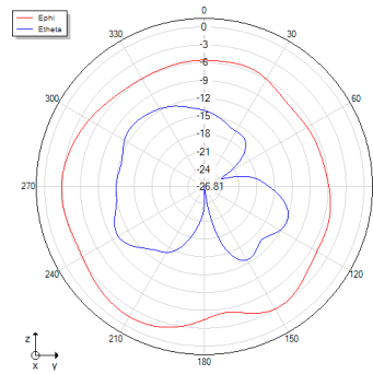
Phi=90 freq=1575.42004394531MHz
