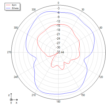
Phi=0 freq=1575.42004394531MHz
