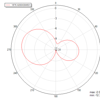
Theta=90 freq=1575.42004394531MHz
