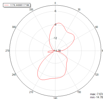
Phi=0 freq=1176.44995117188MHz
