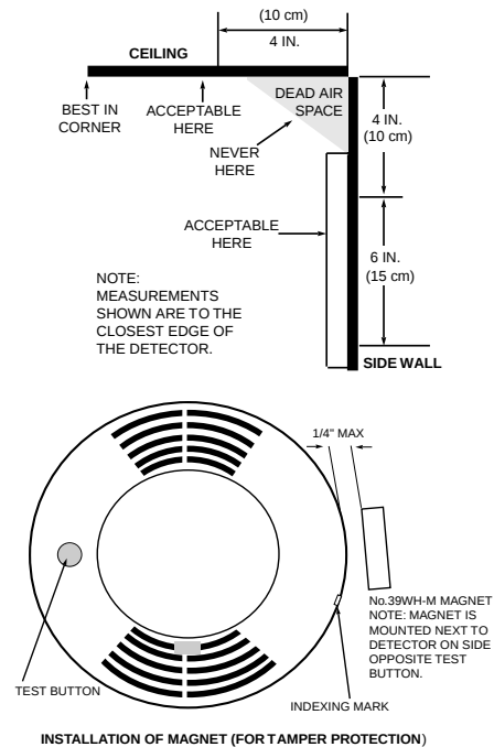
Figure 2. Mounting Details
