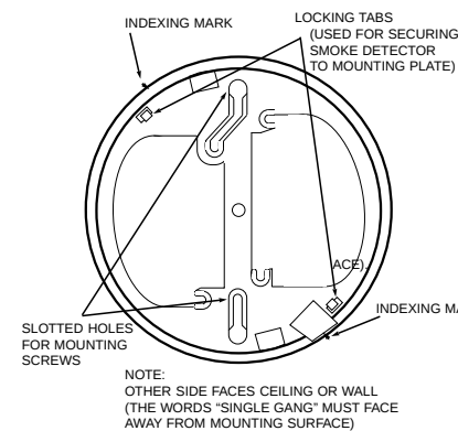
Figure 2. Mounting Details
