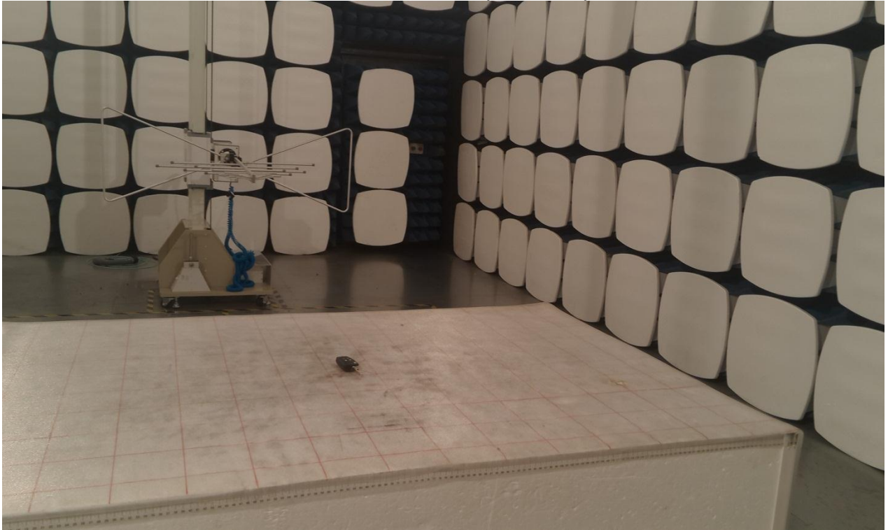
Radiated Emission(below 1G)
