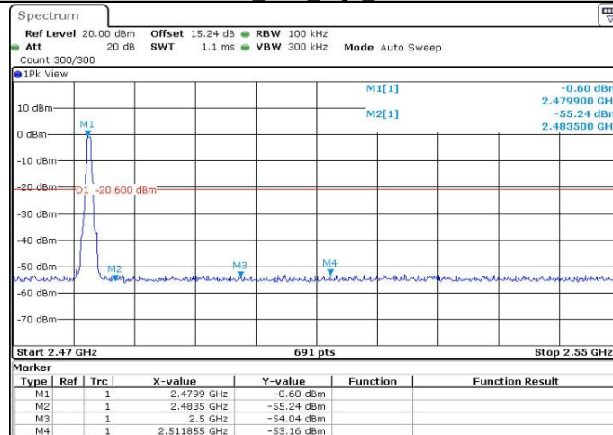
DH1_Ant1_High_2480
