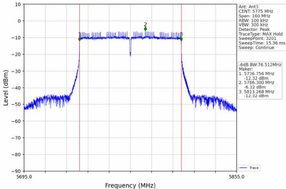
802.11ac(VHT80)_MCH_5775MHz_Ant3_NTNV
