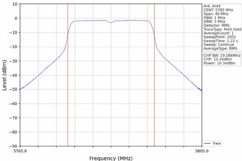
802.11ac(VHT20)_MCH_5785MHz_Ant4_NTNV
