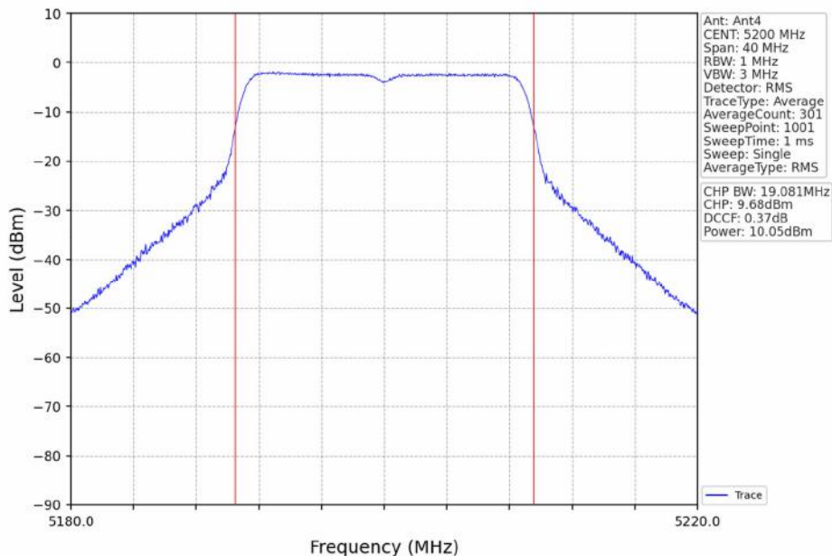
802.11n(HT20)_MCH_5200MHz_Ant4_NTNV
