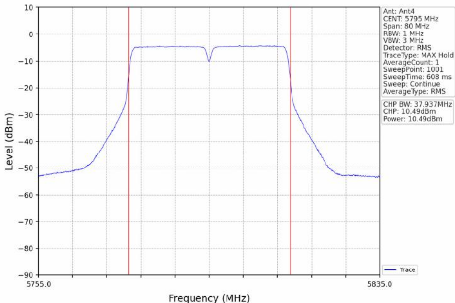
802.11ac(VHT40)_HCH_5795MHz_Ant4_NTNV
