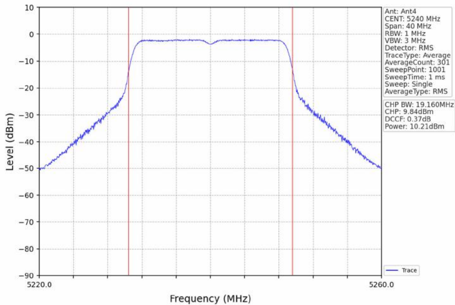
802.11n(HT20)_HCH_5240MHz_Ant4_NTNV
