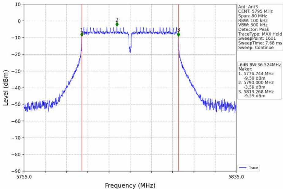
802.11n(HT40)_HCH_5795MHz_Ant3_NTNV
