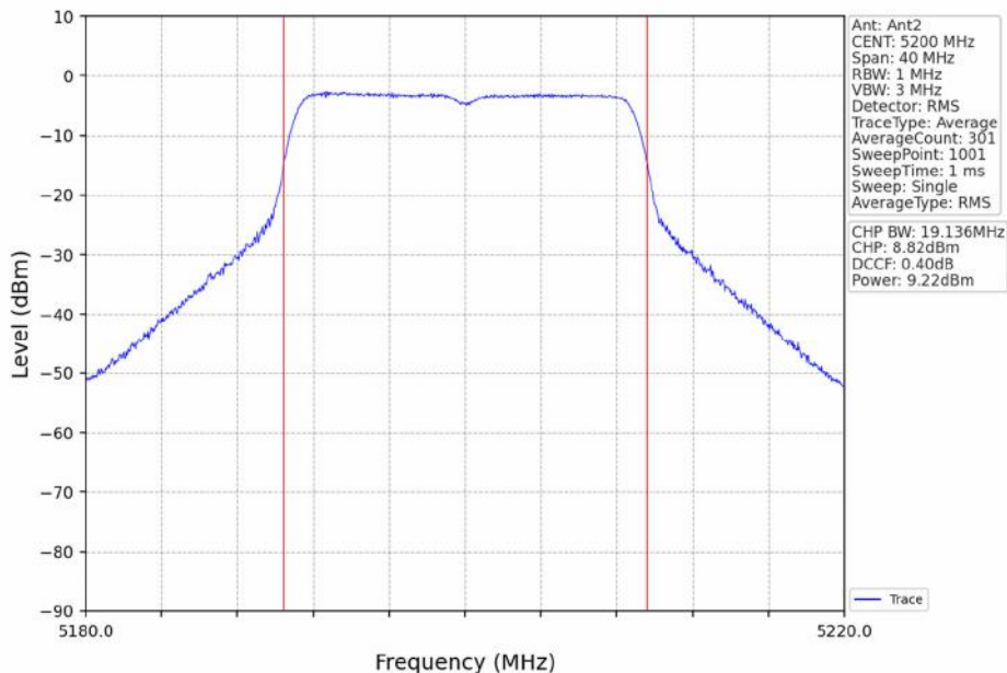
802.11ac(VHT20)_MCH_5200MHz_Ant2_NTNV
