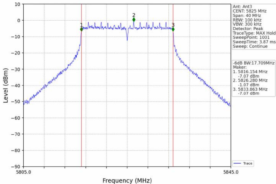
802.11n(HT20)_HCH_5825MHz_Ant3_NTNV
