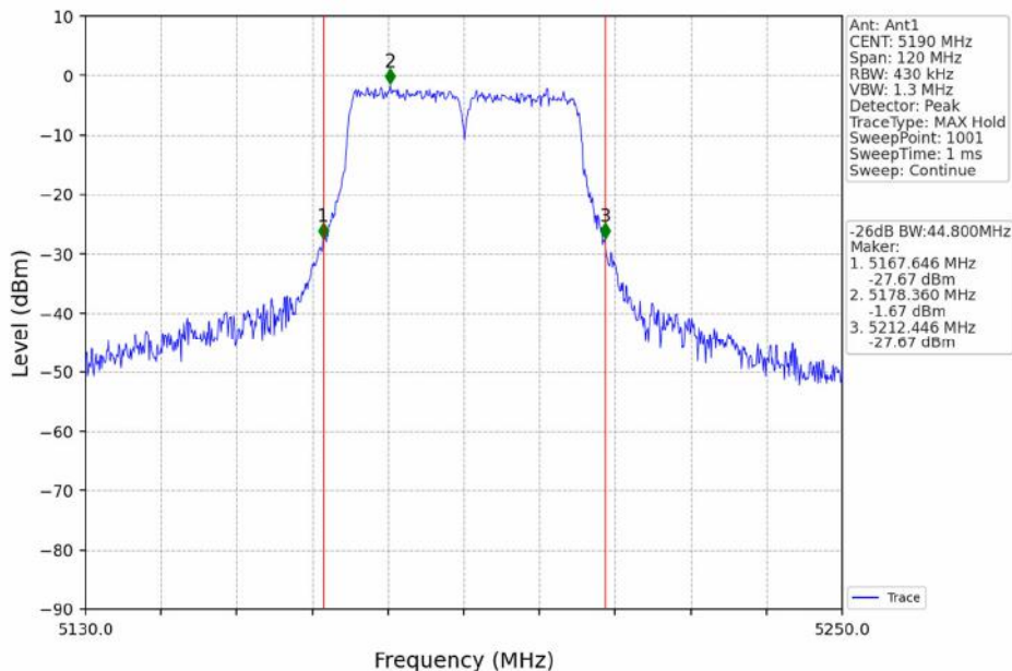
802.11ac(VHT40)_LCH_5190MHz_Ant1_NTNV
