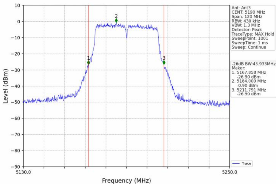
802.11ac(VHT40)_LCH_5190MHz_Ant3_NTNV
