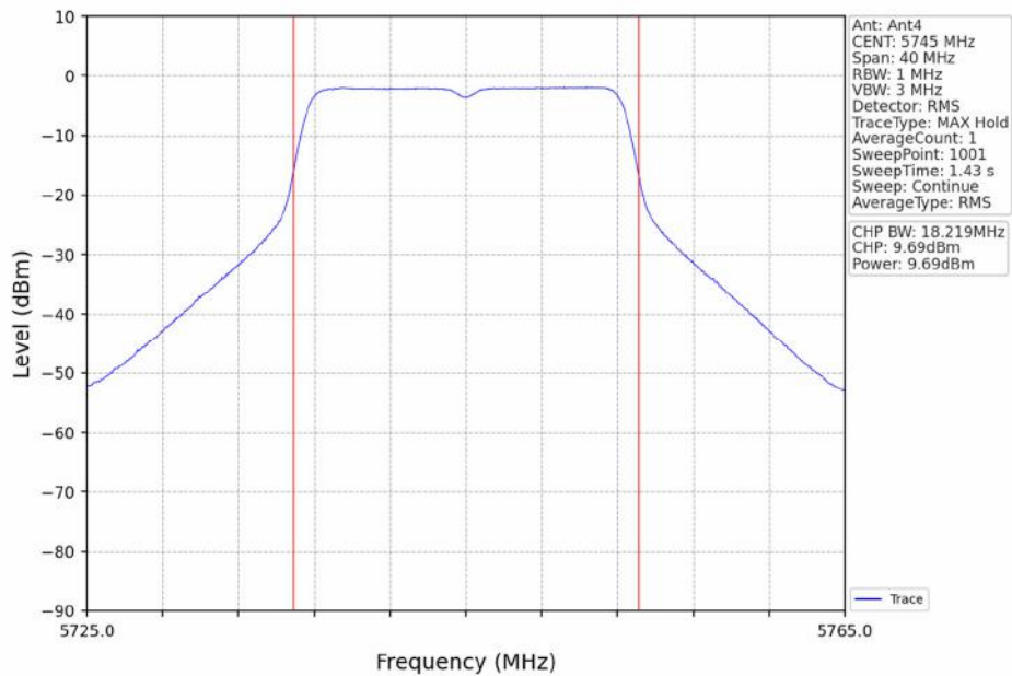
802.11a_LCH_5745MHz_Ant4_NTNV
