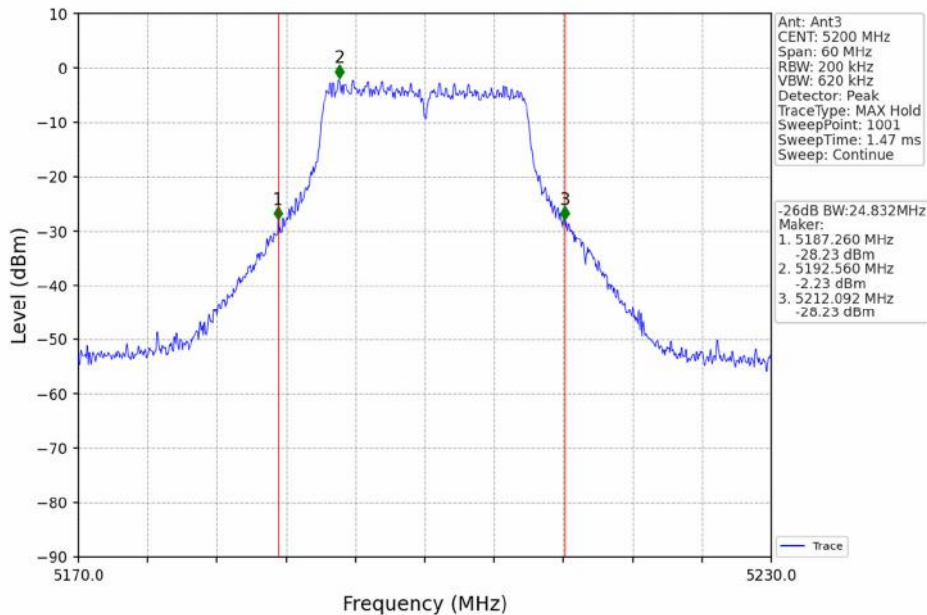
802.11ac(VHT20)_MCH_5200MHz_Ant3_NTNV
