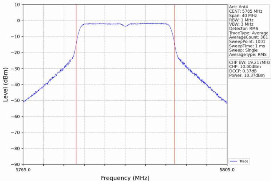
802.11n(HT20)_MCH_5785MHz_Ant4_NTNV
