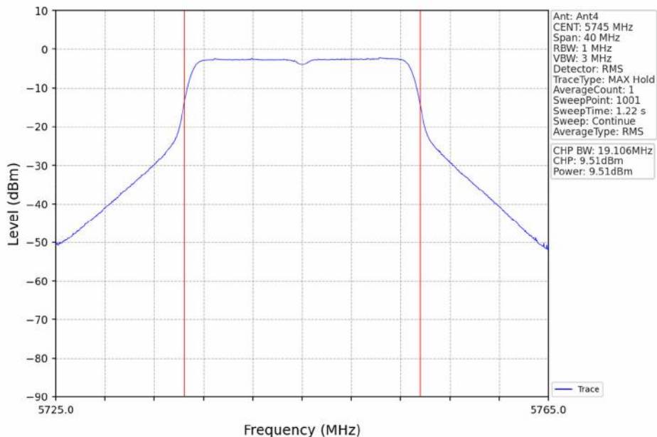
802.11ac(VHT20)_LCH_5745MHz_Ant4_NTNV
