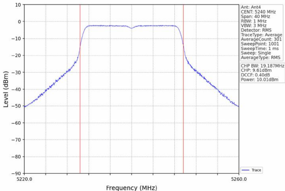
802.11ac(VHT20)_HCH_5240MHz_Ant4_NTNV
