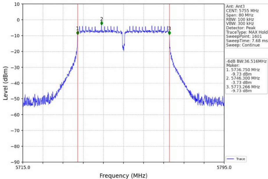
802.11ac(VHT40)_LCH_5755MHz_Ant3_NTNV
