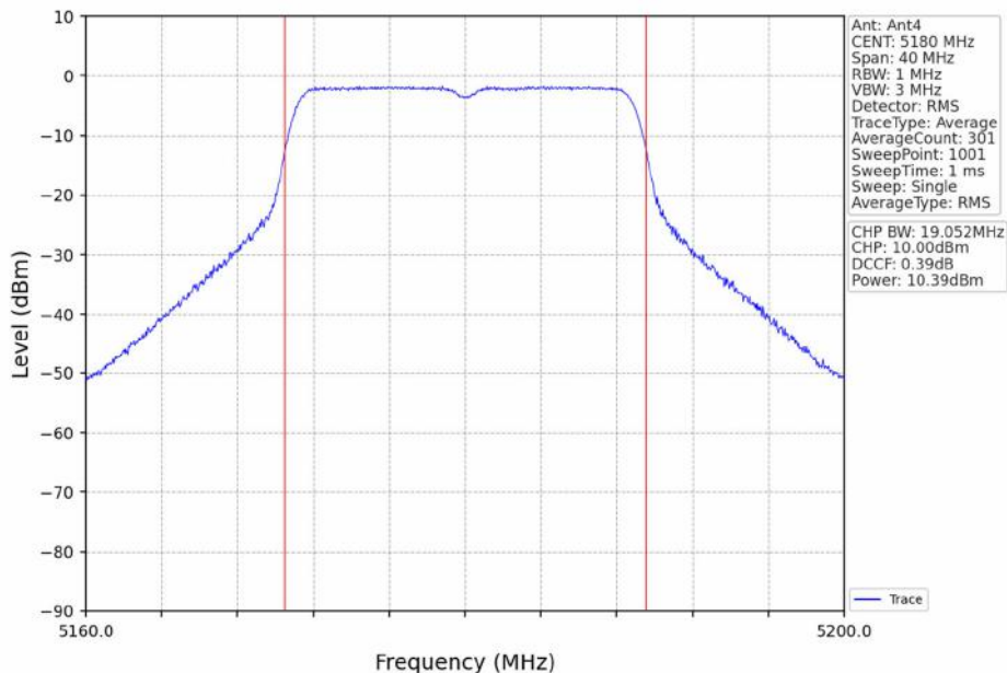
802.11ac(VHT20)_LCH_5180MHz_Ant4_NTNV
