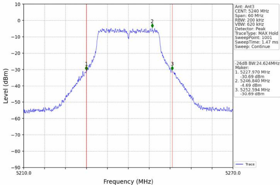
802.11n(HT20)_HCH_5240MHz_Ant3_NTNV
