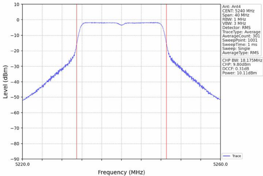
802.11a_HCH_5240MHz_Ant4_NTNV
