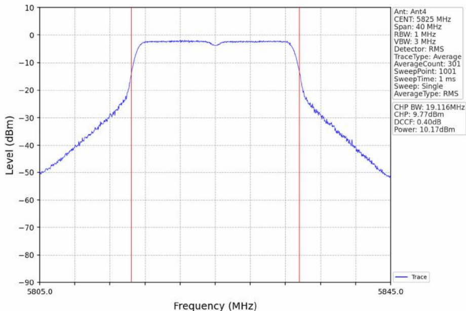
802.11ac(VHT20)_HCH_5825MHz_Ant4_NTNV
