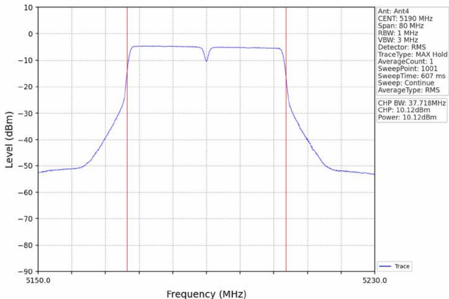
802.11ac(VHT40)_LCH_5190MHz_Ant4_NTNV
