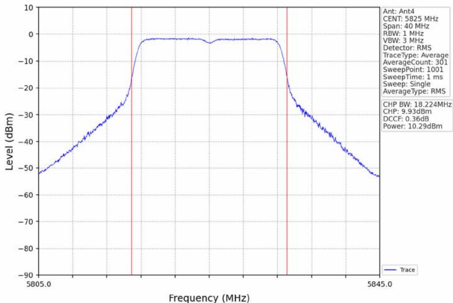
802.11a_HCH_5825MHz_Ant4_NTNV
