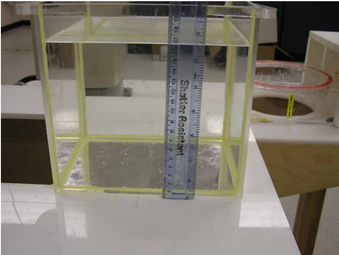
Photo 9: Photo to demonstrate 15 cm Z-axis flat phantom GPRS
