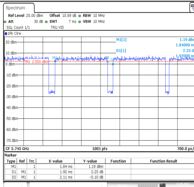
NTNV-11N20MIMO-Ant2-5745
