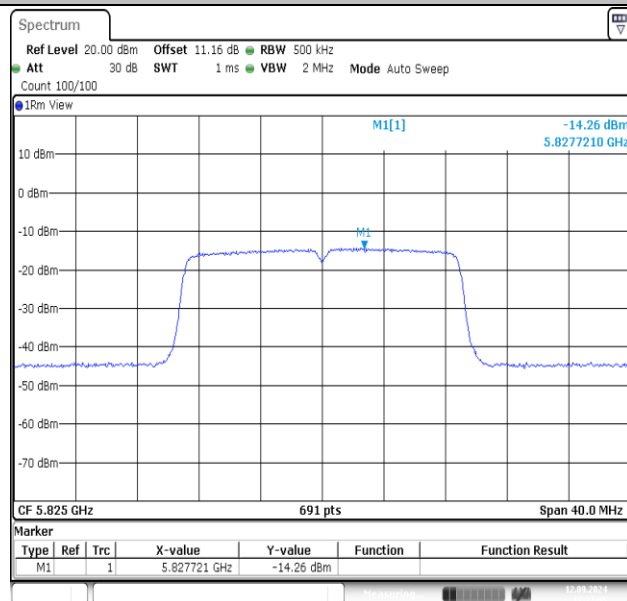
11AC20MIMO-Ant1-5825-PASS
