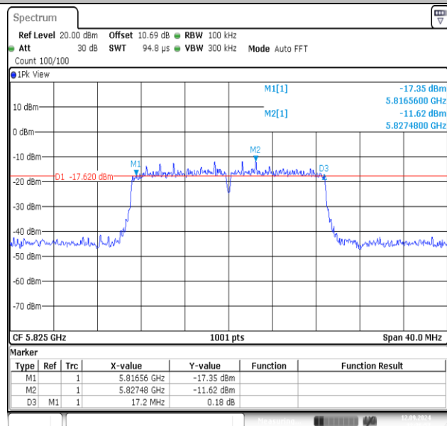
11AC20MIMO-Ant1-5825-PASS
