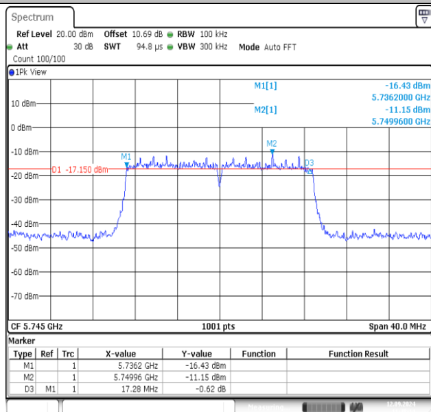
11N20MIMO-Ant2-5745-PASS
