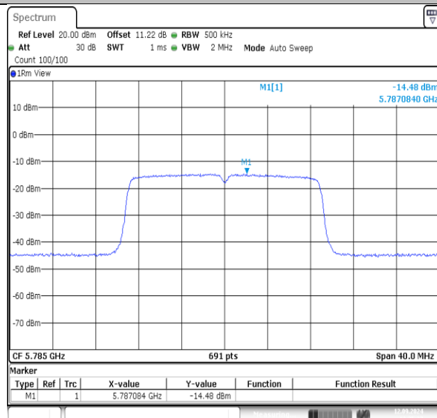
11AC20MIMO-Ant1-5785-PASS
