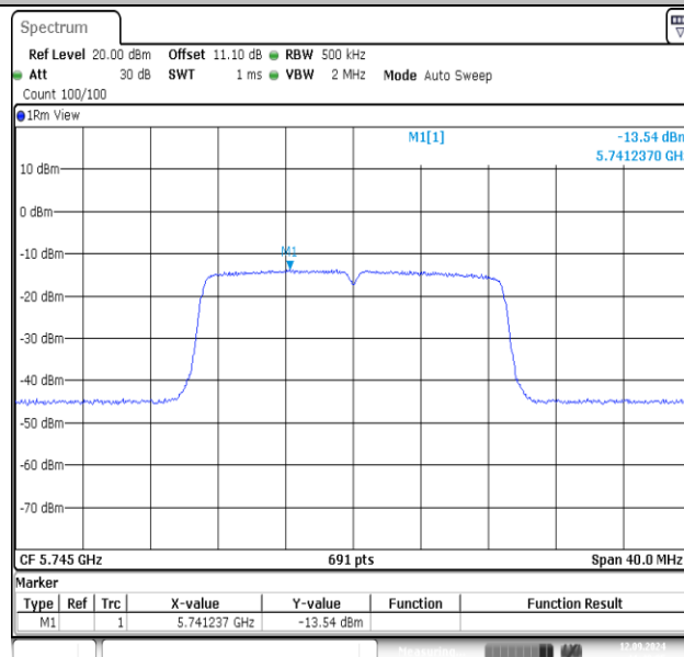
11N20MIMO-Ant2-5745-PASS
