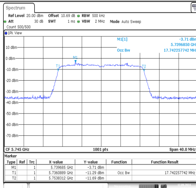
11AC20MIMO-Ant2-5745
