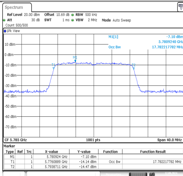
11N20MIMO-Ant1-5785
