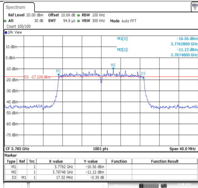
11AC20MIMO-Ant1-5785-PASS
