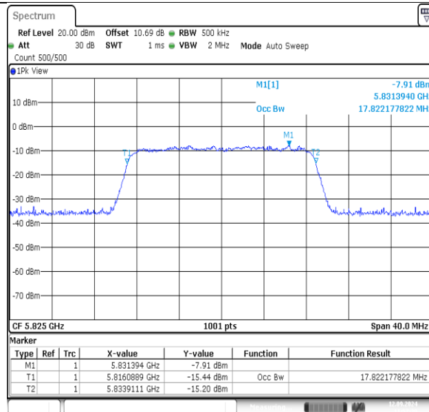
11N20MIMO-Ant2-5825
