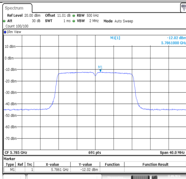
11A-Ant1-5785-PASS
