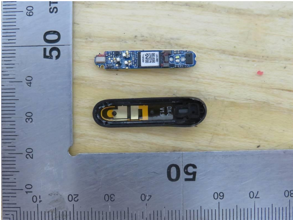
Internal View of EUT-Left Earbud-3
