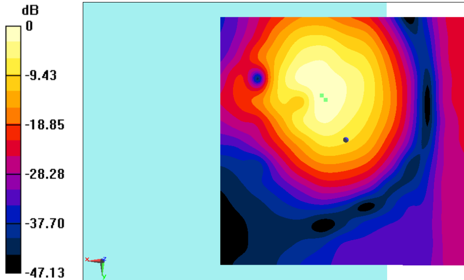
Fig B.4 T-Coil LTEB2
