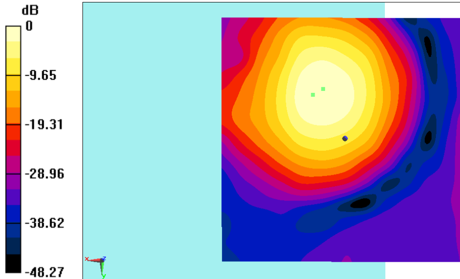
Fig B.2 T-Coil WiFi2.4G
