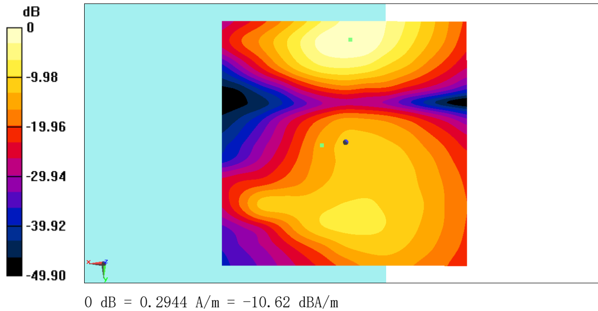
Fig B.3 T-Coil WiFi5G
