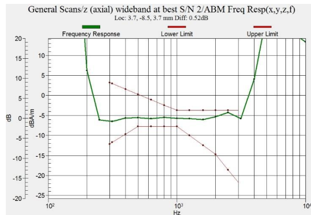
Figure C.2 Frequency Response of LTEBand 2 - OTT VoIP
